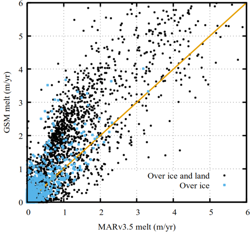
Figure 4. Comparison of net melt (total melt - refreezing) between the GSM and the results of 20 km resolution regional climate modelling (1879:1999 mean climatology, MARv3.5.2, Fettweis et al., 2017) for the present-day GRIS. The GSM used the mean monthly precipitation and 2-meter temperature climatologies from the latter.
