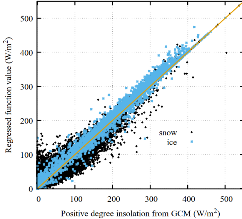
Figure 3. Comparison of GCM computed and regressed function used in GSM for monthly mean of positive degree daily surface insolation. Results are disaggregated for snow and ice surfaces for with ensemble parameter C_{\text{RadSMB}} in eq. 17 set to its nominally regressed value of 0.345.
