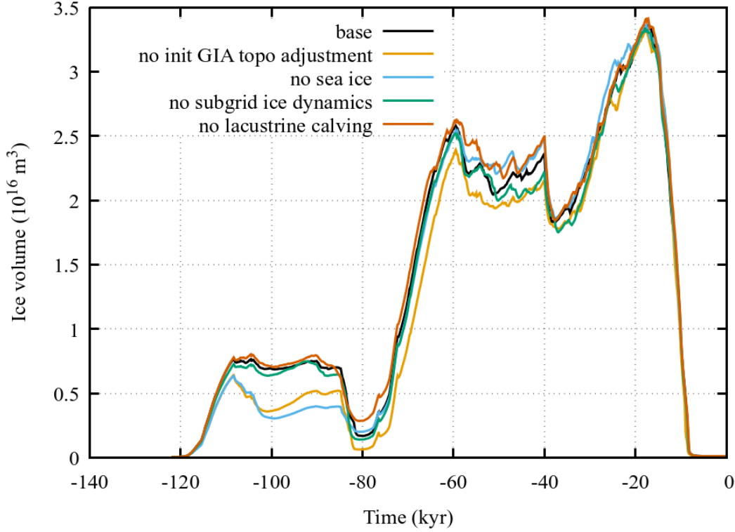
Figure 5. Some example examples of GSM sensitivities to one at a time process removal for a NAIS simulation.
