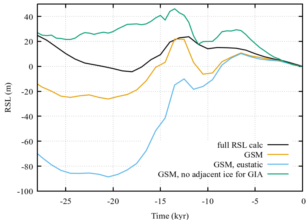
Figure 8. Comparison of computed relative sea level (RSL) for Franz Joseph Fjord Greenland ( 27.42^\circ west, 73.02^\circ N). Shown are: the gravitationally-self consistent solution from post-processing (“full RSL calc”), the GSM internal solution using linear geoidal deflection (“GSM”), the solution when geoidal deflection is typically neglected (“GSM, eustatic”), and the GSM solution when ice outside of the regional grid is not accounted for in the visco-elastic bedrock response calculation (“GSM, no adjacent ice for GIA”).
