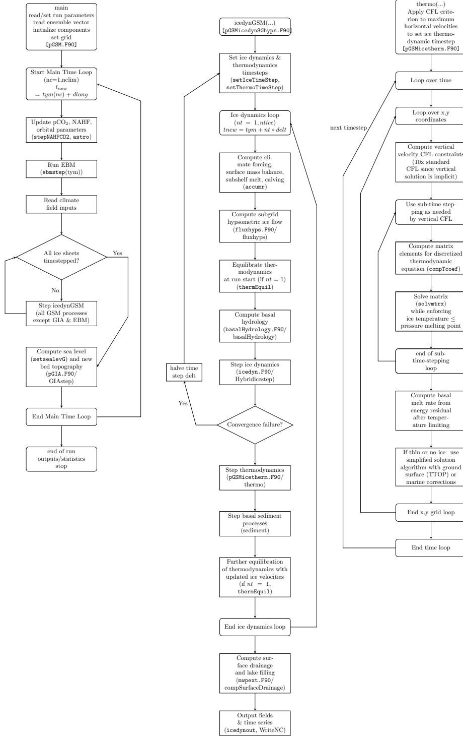
Figure A1. GSM nested flow chart. Relevant GSM subroutine or variable names are shown within parentheses and relevant source files are either enclosed with square brackets or have a '/' separating it from the embedded subroutine name.
