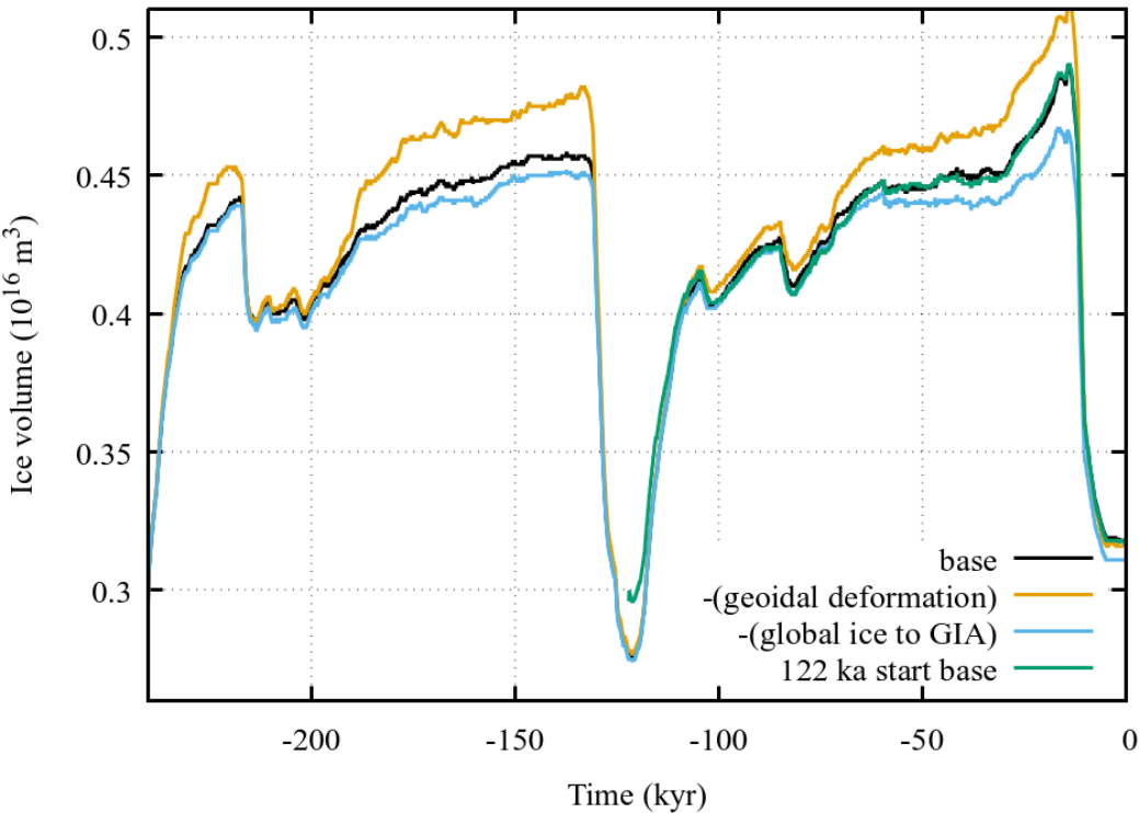
Figure 7. Example Examples of process removal sensitivities as given by mean response for a 10 member GRIS ensemble. The listed time series are identified by the GSM process that has been removed.
