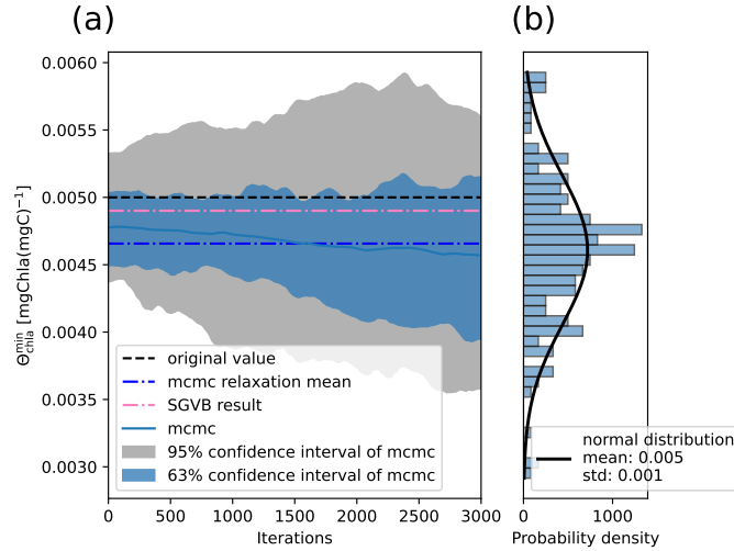
Figure 9. Result of the Metropolis-Hasting Algorithm for the parameter \Theta_{\text{chla}}^{\min} [ \text{mgChla}(\text{mgC})^{-1} ], using the transition probability shown in Eq. (23), with initial conditions close to the value obtained after performing Alternate Minimization. (a) Evolution of the parameter after each iteration of the algorithm, (b) final probability density estimated as a Gaussian distribution.
