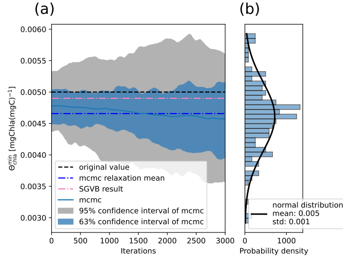
Figure 9. Result of the Metropolis-Hasting Algorithm for the parameter \Theta_{chl a}^{min} [ \text{mgChla}(\text{mgC})^{-1} ], using the transition probability shown in Eq. (23), with initial conditions close to the value obtained after performing Alternate Minimization. (a) Evolution of the parameter after each iteration of the algorithm, (b) final probability density estimated as a Gaussian distribution.
