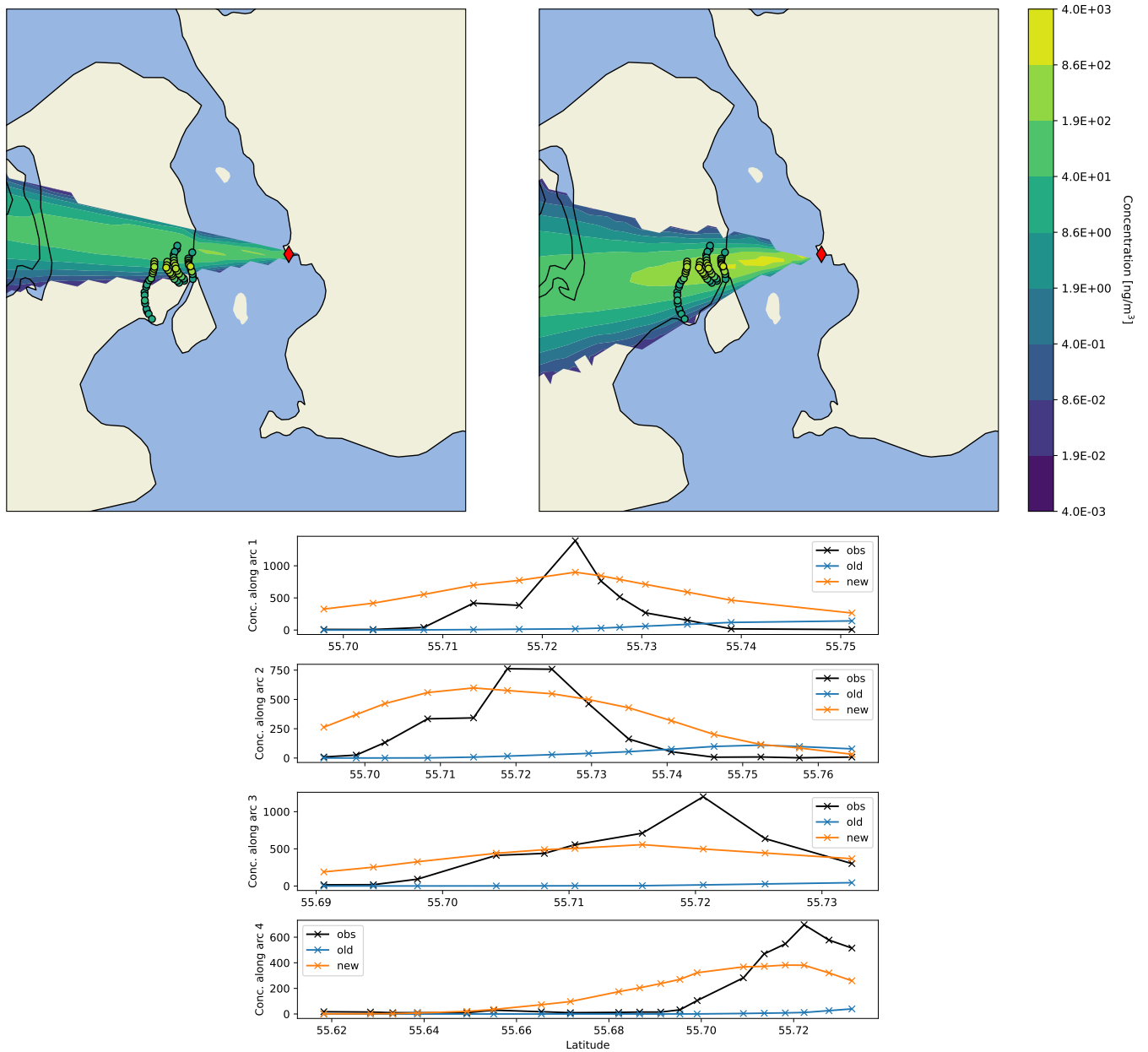
Figure 3. Examples of results are shown for a selected dispersion scenario for the Øresund experiment. The measurements and model results show average air concentrations during the interval 10 UTC to 11 UTC, 6 June 1984. In the upper plots, the plumes show the model results of both the old (left) and new (right) models, while the dots show the measured values. In the lower plot, observations are shown together with model predictions at the measurement locations. The arcs are numbered from 1 to 4, with 1 being the arc closest to the release location.
