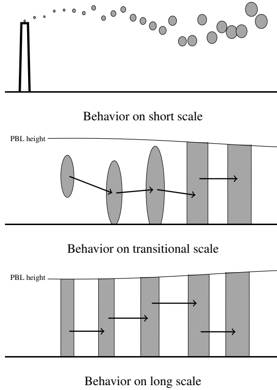
Figure 1. Illustration of the formulation used in the new version of DERMA. The upper sketch shows how puffs are released from the top of a stack and are randomly displaced vertically. The middle sketch shows the transition when a puff starts using a uniform concentration distribution in the vertical direction. Finally, the lower sketch shows how the long-range formulation works; puffs assume a uniform vertical distribution inside the PBL, and the height of the puff centroid is displaced vertically with the stochastic transport scheme.
