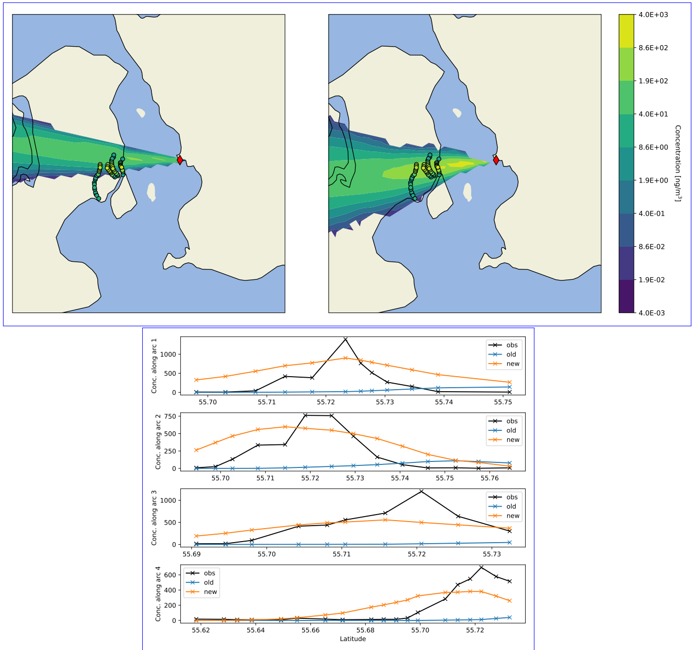
Figure 3. Examples of results are shown for a selected dispersion scenario for the Øresund experiment. The measurements and model results show average air concentrations during the interval 10 UTC to 11 UTC, 6 June 1984. In the upper plots, the plumes show the model results of both the old (left) and new (right) models, while the dots show the measured values. In the lower plot, observations are shown together with model predictions at the measurement locations. The arcs are numbered from 1 to 4, with 1 being the arc closest to the release location.
