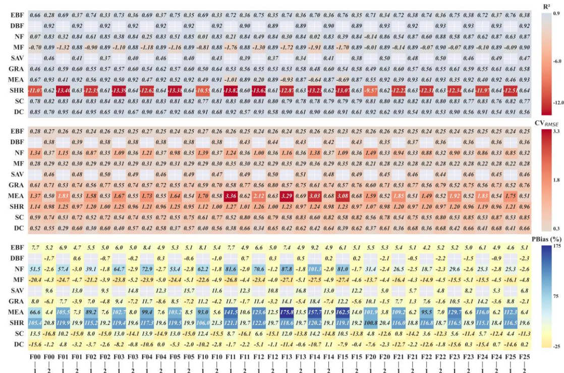
Figure 12. Comparison of statistical indicators ( R^2 , CV_{RMSE} , PB_{ias} ) of FLAML-LUE model under drought conditions and non-drought conditions for different land cover types (1 represents drought, 2 represents non-drought).
