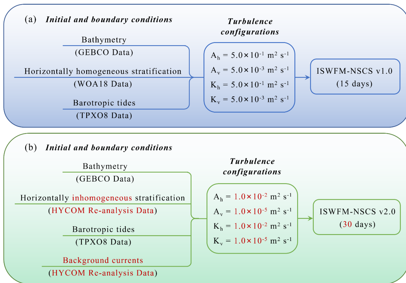
Figure 1. (a) The schematic of configuration and implementation of ISWFM-NSCS v1.0, which includes initial and boundary conditions. (b) Same as (a) but for ISWFM-NSCS v2.0. Note that the major model updates are marked in red in (b).
