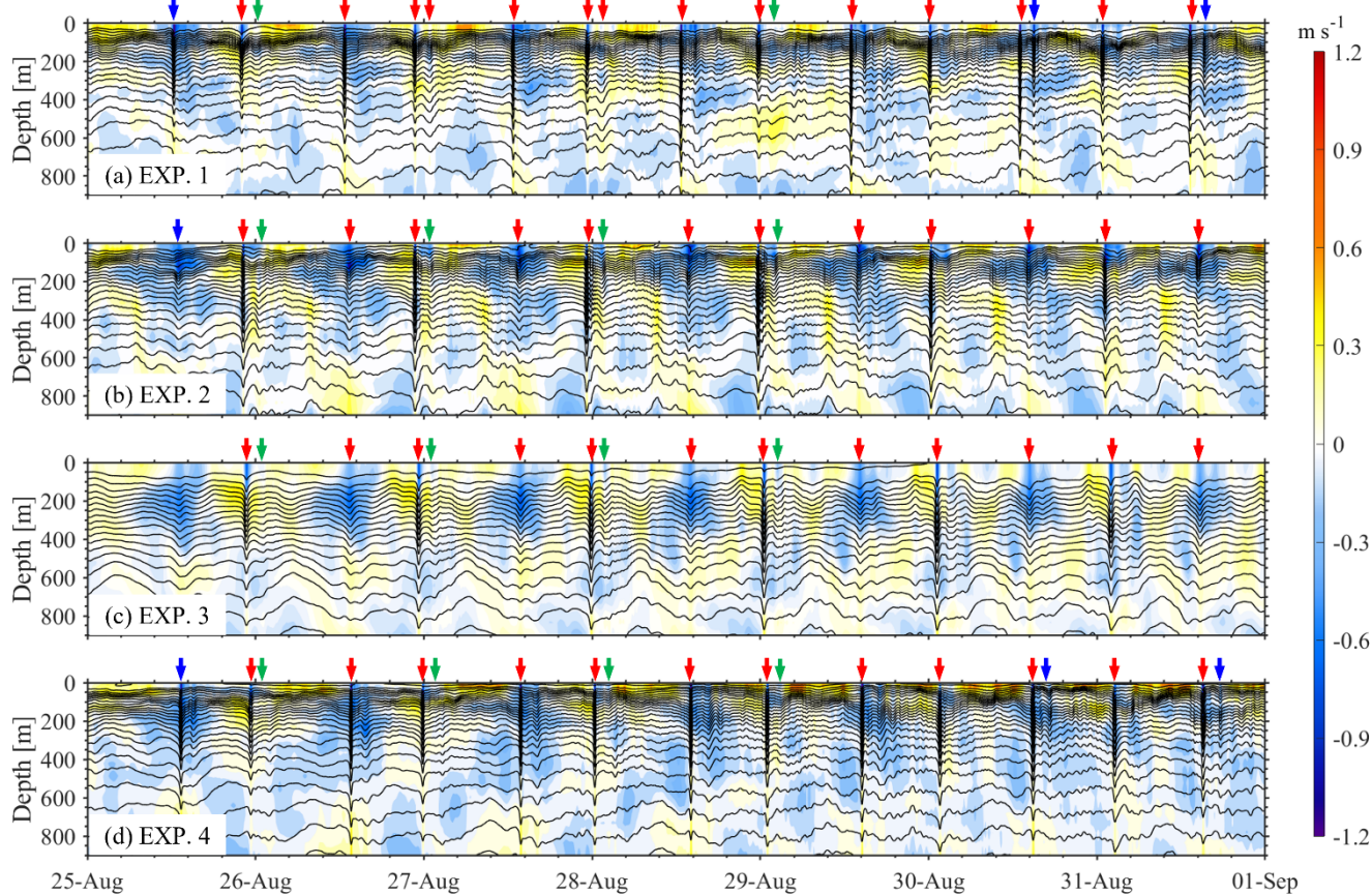
Figure 10. Time series of temperature and baroclinic velocities at station DS from 25 August to 01 September 2014 for the 530 model runs: (a) EXP. 1, (b) EXP. 2, (c) EXP. 3, and (d) EXP. 4. Red arrows highlight ISWs detected by the model, while blue and green arrows denote the false positive and false negative results, respectively.
