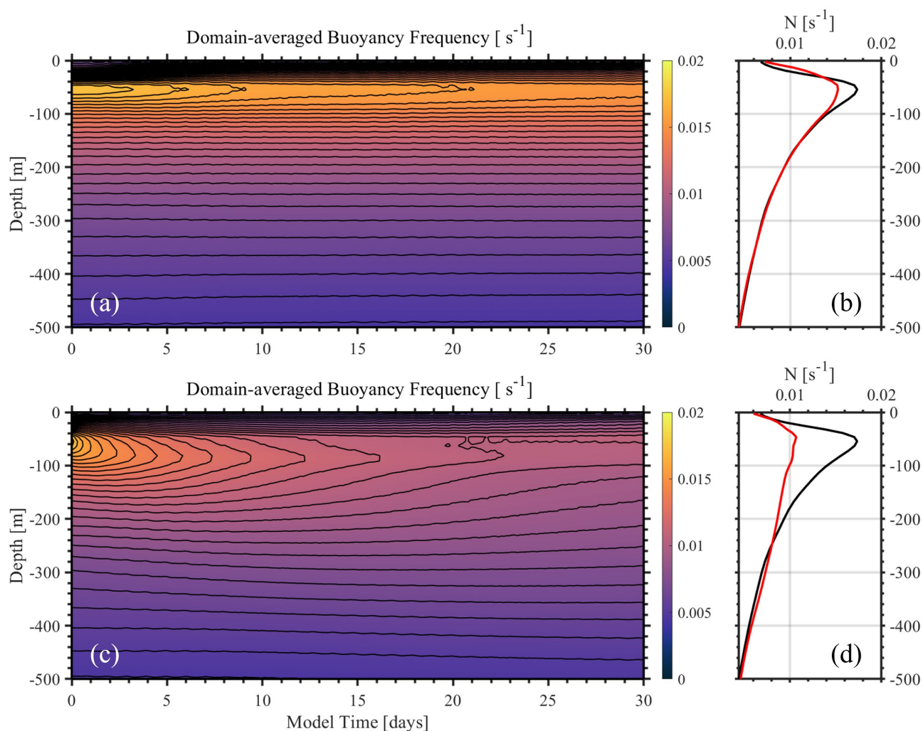
520 Figure 8. (a) Time series of horizontally-averaged background buoyancy frequency in the upper 500 m through the entire model domain in EXP. 2. (b) Black and red lines represent the averaged buoyancy frequency profiles at the beginning and at the ending of the model, respectively. (c-d) Same as (a-b) but in EXP. 3.
