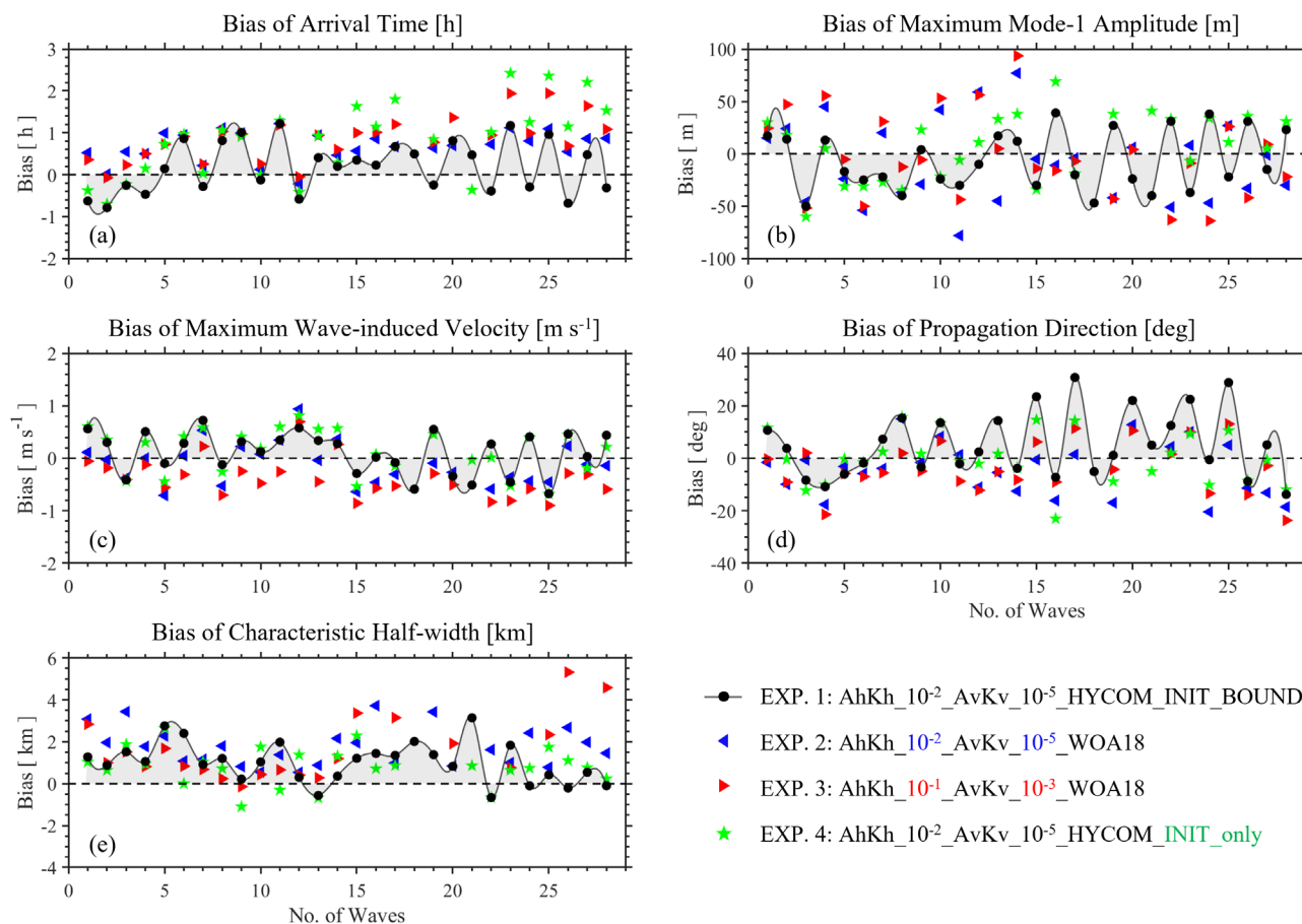
Figure 11. Bias in arrival time (a), maximum mode-1 amplitudes (b), wave-induced velocities (c), propagation directions (d), and half-widths (e) for twenty-eight ISWs at station DS. Different colours represent results from different experiments (EXP.
