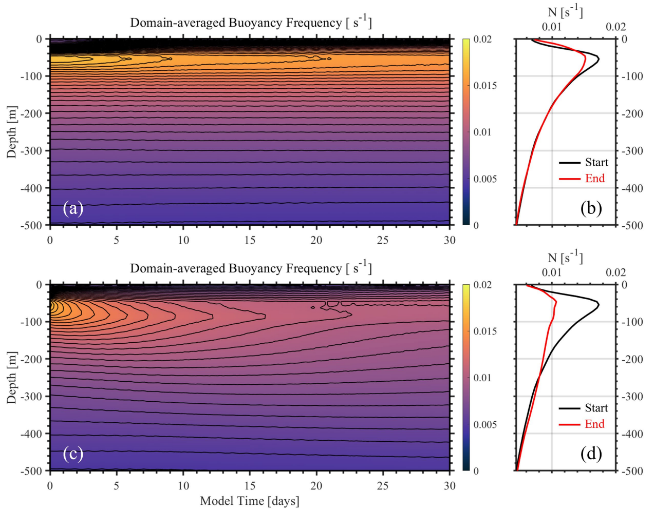
635 Figure 8. (a) Time series of horizontally-averaged background buoyancy frequency in the upper 500 m through the entire model domain in EXP. 2. (b) Black and red lines represent the averaged buoyancy frequency profiles at the beginning and at the ending of the model, respectively. (c-d) Same as (a-b) but in EXP. 3.
