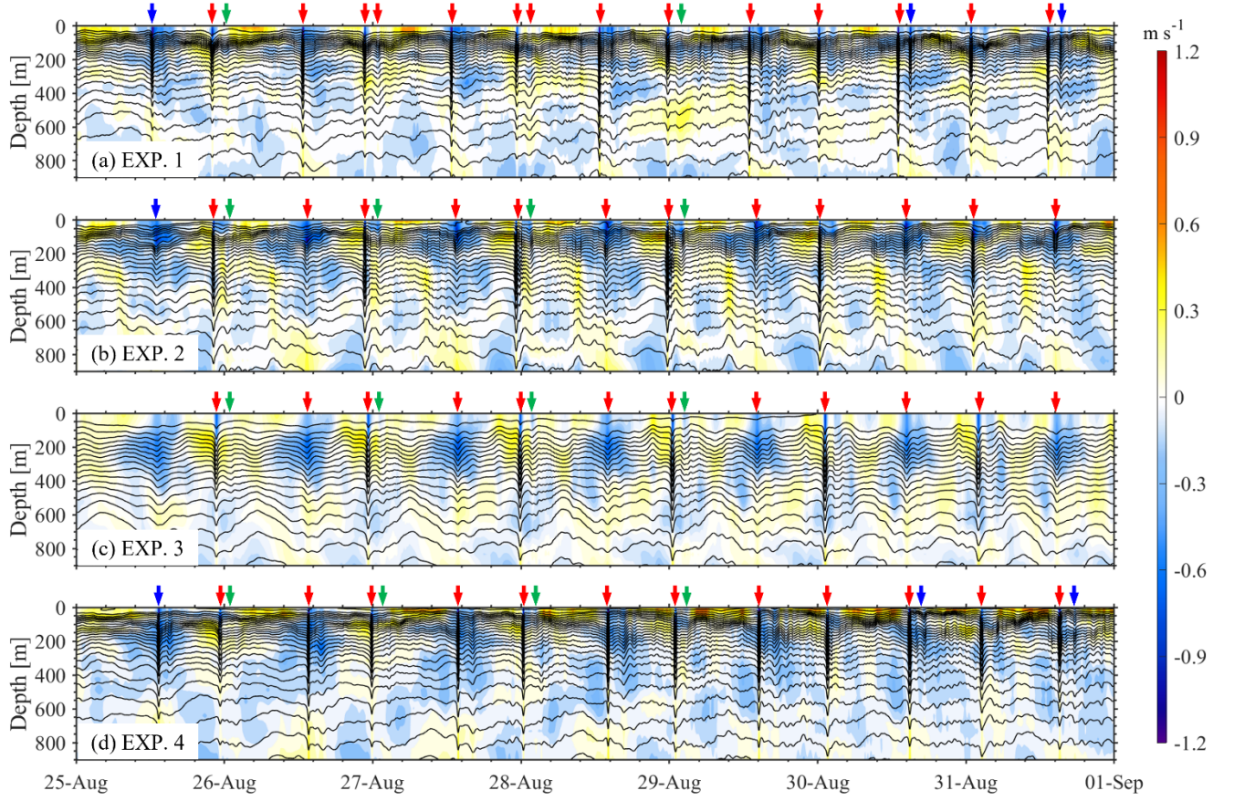
Figure 10. Time series of temperature and baroclinic velocities at station DS from 25 August to 01 September 2014 for the 645 model runs: (a) EXP. 1, (b) EXP. 2, (c) EXP. 3, and (d) EXP. 4. Red arrows highlight ISWs detected by the model, while blue and green arrows denote the false positive and false negative results, respectively.
