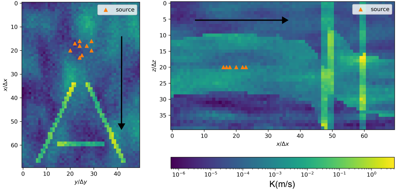
Figure 2. Sections of the hydraulic conductivity field (in m/s) for the fault scenario (1, 1, 1), where all three faults act as pathways (i.e., increase conductivity). The hydraulic conductivity field is generated using a multi-Gaussian spatial random field model with heterogeneous geological units. (a) Horizontal section at depth index z/\Delta z = 30 ; (b) Vertical section at lateral index y/\Delta y = 15 . Fault planes are vertical and orthogonal to the x-y plane. The orange dots represent the possible contaminant injection locations. The black arrow indicates the main direction of flow (along the x-axis). Axes are labeled in terms of discretization units.
