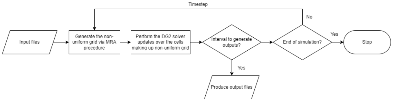
Figure 1: The main operations involved in the GPU-MWDG2 solver (further detailed in Appendix A).
