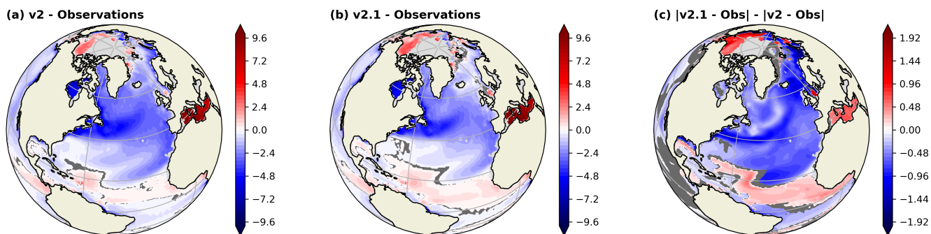
Figure 4. Same as Figure 3 but for SSS (psu).
