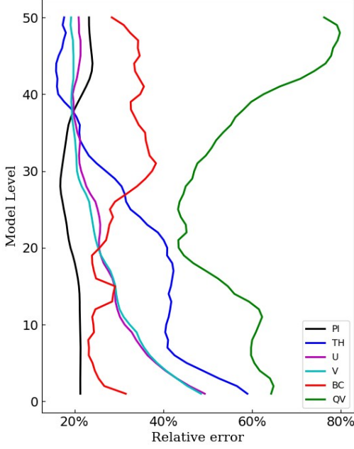
Figure 4: The vertical distribution of the globally averaged relative error between the perturbation forecasts of the CMA-GFS-AERO TLM and NLM at the resolution of 1.0^\circ . (black line: non-dimensional pressure, blue line: potential temperature, red line: BC, magenta line: u-wind, cyan line: v-wind; green line: specific humidity).
