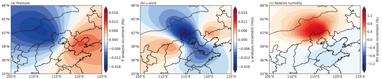
Figure 8: The analysis increments of (a) pressure, (b) east-west component of horizontal wind, and (c) relative humidity at the first model layer at the beginninginitial of the assimilation time window, 0300 UTC, with the BC observation placed at the end of the assimilation time window, 0900 UTC. The black triangle represents the ideal observation location (116.47°E, 39.8°N).
