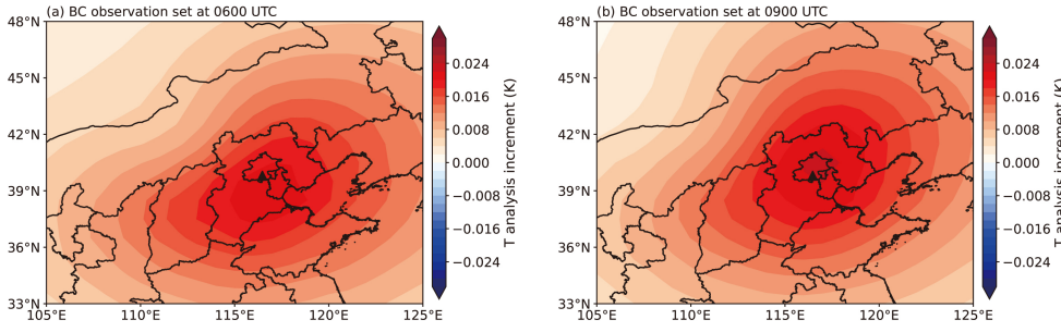
Figure 7: The analysis increments of temperature at the first model layer at the beginninginitial of the assimilation time window, 0300 UTC, with the BC observation placed at (a) the middle of the assimilation window, 0600 UTC; (b) the end of the assimilation time window, 0900 UTC. The black triangle represents the ideal observation location (116.47°E, 39.8°N).
