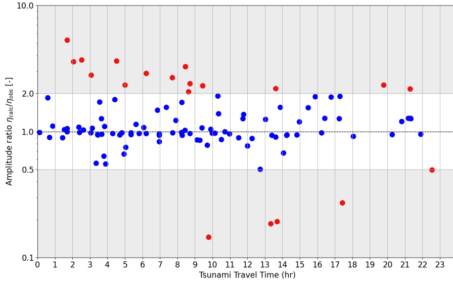
Figure 18. Amplitude ratio against tsunami travel time for Tateyama 2009, Tohoku 2011 and Alaska 2018 study cases at various DART buoy locations with tsunami travel time up to 24hr.
