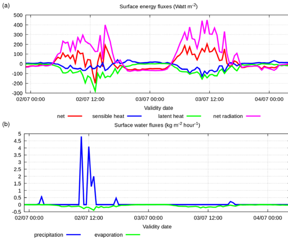
885 Figure 13. Observation data (BALTEX) in Falkenberg 2-3 July 2003, parameters at the surface: (a) solar radiation and heat fluxes (W m -2 ); (b) precipitation and evaporation rate (kg m -2 hour -1 ).
