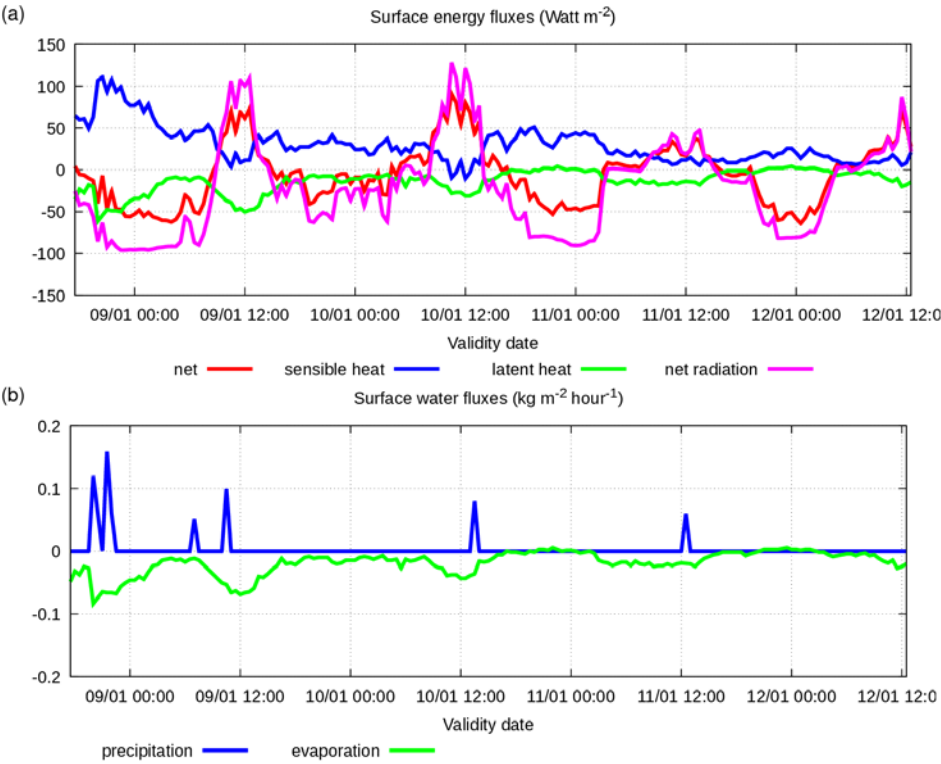
Figure 16. Observation data (BALTEX) in Falkenberg 8-12 January 2005, parameters at the surface: (a) solar radiation and heat fluxes (W m -2 ); (b) precipitation and evaporation rate (kg m -2 hour -1 ).
