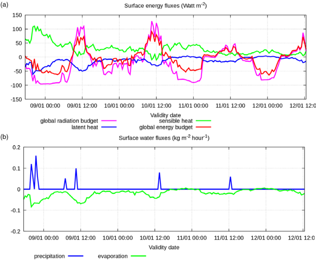
965 Figure A4. Observation data (BALTEX) in Falkenberg 8-12 January 2005, parameters at the surface: (a) solar radiation and heat fluxes (W m -2 ); (b) precipitation and evaporation rate (kg m -2 hour -1 ).
