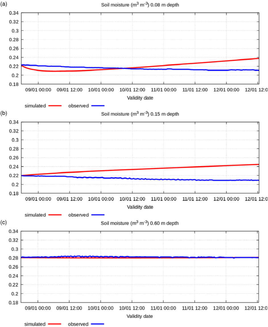
940 Figure 18. Simulated and observed 8-12 January 2005 soil specific volumetric water content ( \text{m}^3 \text{m}^{-3} ) at various depths: (a) -0.08 m; (b) -0.15 m; (c) -0.60 m.
