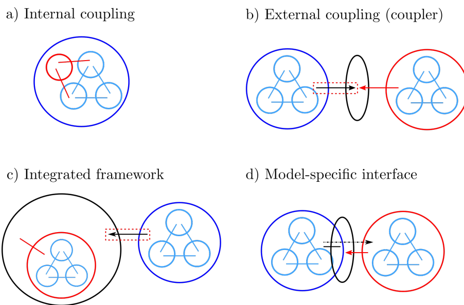
Figure 1. Overview of model extension methods. In each approach one ESM component acts as the host model (blue circle with smaller light blue circles indicating internal functionalities like parameterisations and dynamical core), which can be extended by these four methods. Extensions are highlighted by red colour and software to support these extensions in approaches b) to d) by black circles. Red circles are set around new ESM components (approach b)-d)) or smaller extensions (approach a)). Straight lines indicate exchange of data and access to routines. An arrow is added if access to routines between components is only possible one-way. For example software A can call routines of software B but not vice versa, where software A could be an ESM component and software B a coupler. In this case, the arrowhead is located at the software B (the coupler), to indicate the software, from which routines can be called. Red dashed rectangles indicate that additional infrastructure is required for each host model component when it becomes connected to the coupler or IF for the first time but that the corresponding coding effort is only required once. The red line in approach c), connecting the new component and the IF, indicates that the component needs to be integrated into the IF. For a model-specific interface (approach d)) the dot-dashed line from the host model to the new component visualises the fact that routines are called, but only indirectly via the interface itself (callback mechanism introduced in Section 2).
