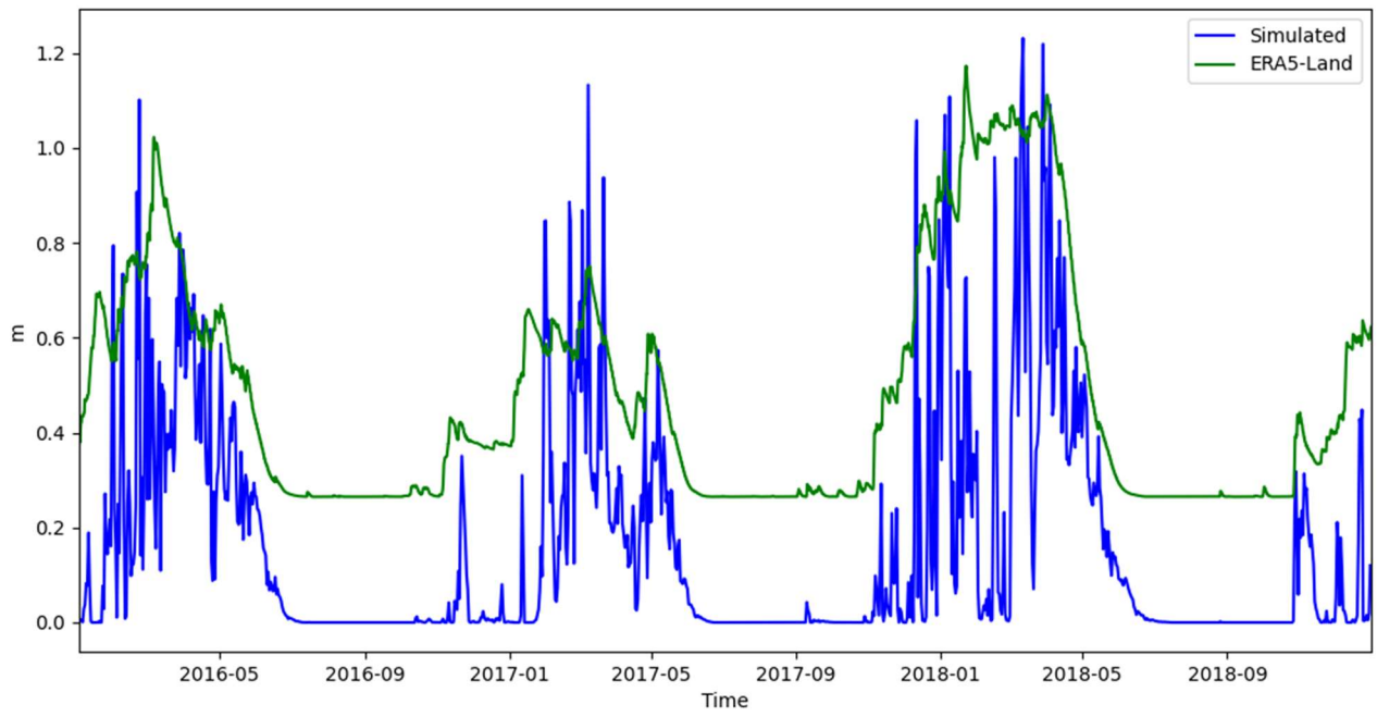
Fig S1. Spatial daily mean snow depth from WRF-Hydro output (blue) and ERA5-Land dataset (green).
