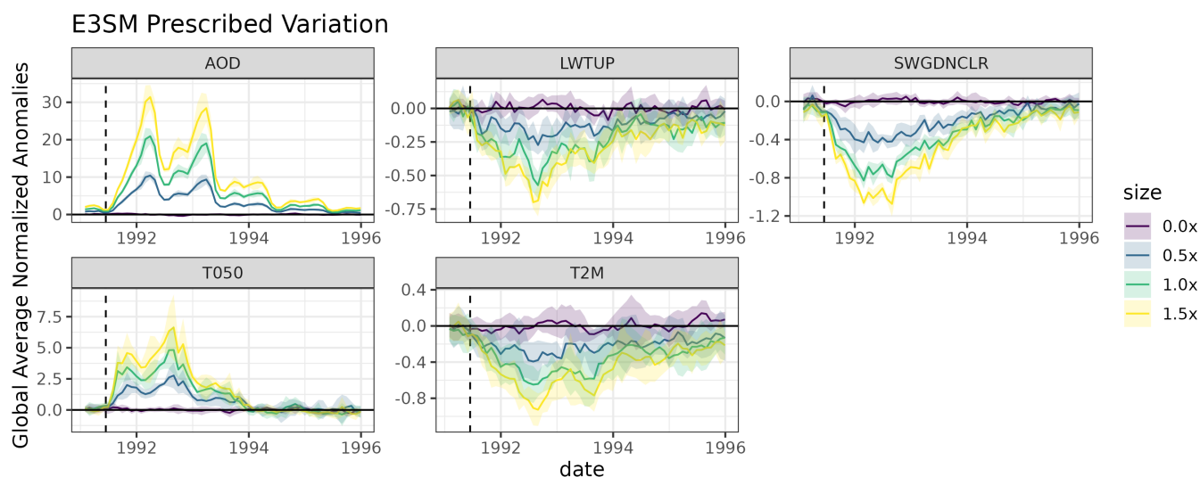
Figure C1. Globally averaged normalized anomalies for prescribed variation E3SM. Note the y-axis scale is different for each plot. Shaded area represents \pm one standard deviation of ensemble variability.
