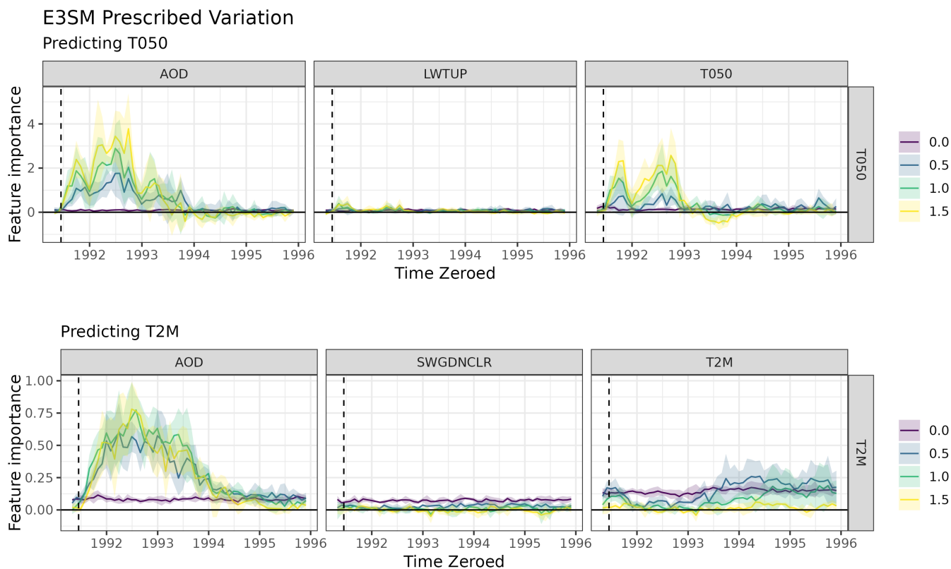
Figure C2. stZFI for E3SM simulations with prescribed eruptions. Color denotes relative size of eruption compared to actual Pinatubo eruption. Note the y-axis scales are different for the two rows.
