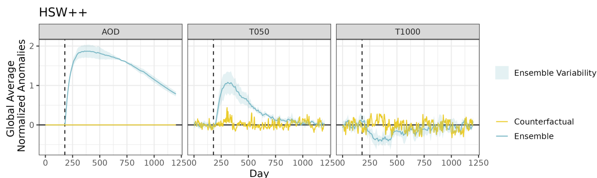
Figure 2. Globally averaged normalized anomalies for HSW++ for aerosol injection ensemble and counterfactual. Solid line is mean across ensembles. Vertical dashed lines on day 179 denote the aerosol injection. Shaded regions represent \pm 1 standard deviation of ensemble variability. There is only one counterfactual run.
