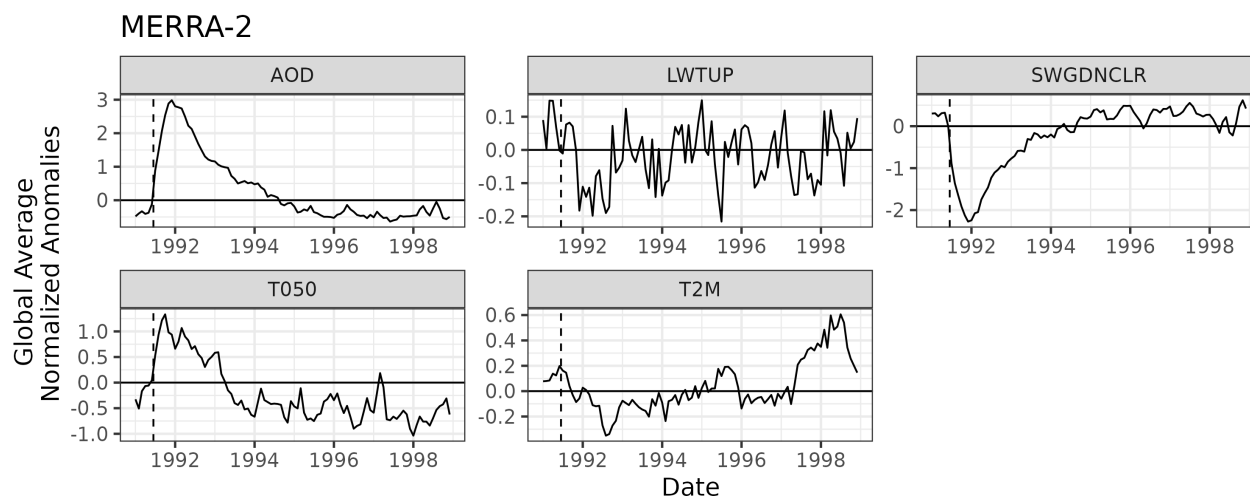
Figure 9. Globally averaged normalized anomalies for MERRA-2. Note the y-axis is different for each plot. Vertical dashed lines denote the June 15, 1991 Mount Pinatubo eruption.
