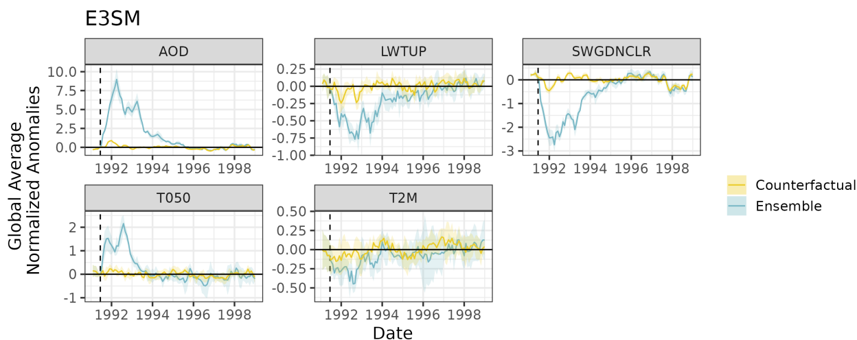
Figure 6. Globally averaged normalized anomalies for E3SM ensemble and counterfactuals. Note the y-axis is different for each plot. Shaded area represents \pm one standard deviation of ensemble variability. Vertical dashed lines denote the June 15, 1991 Mount Pinatubo eruption.
