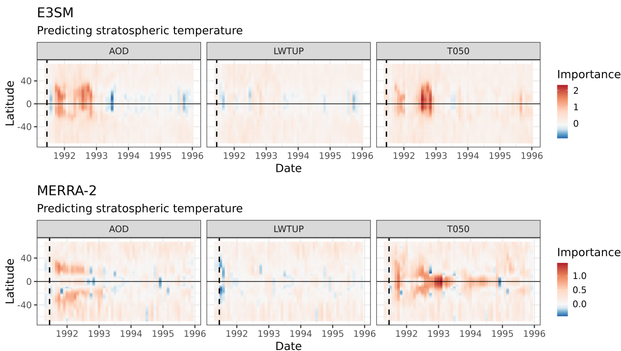
Figure 11. Latitudinal contributions to stZFI for E3SM and MERRA-2 for models predicting T050. Note importance scales are different for E3SM and MERRA-2. Vertical dashed lines denote the June 15, 1991 Mount Pinatubo eruption.
