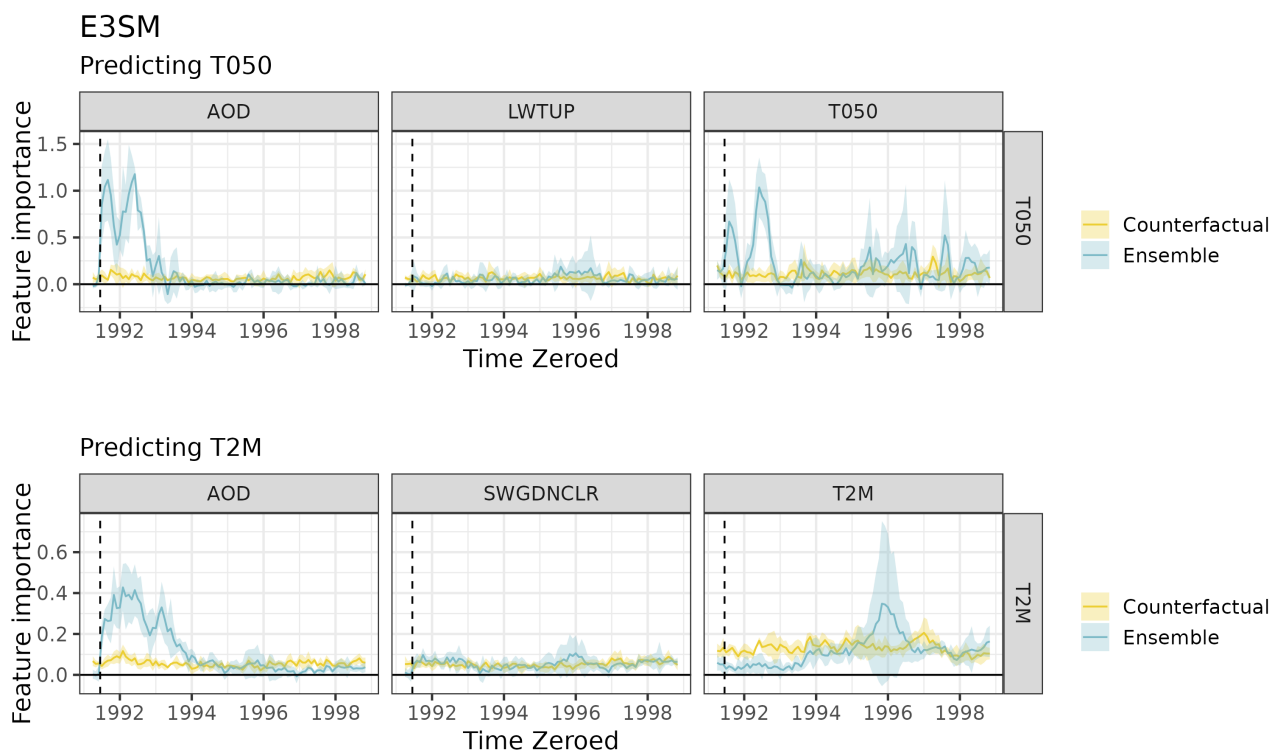
Figure 7. stZFI for E3SM ensembles and counterfactuals. Shaded region denotes \pm one standard deviation of ensemble variability. Vertical dashed lines denote the June 15, 1991 Mount Pinatubo eruption.
