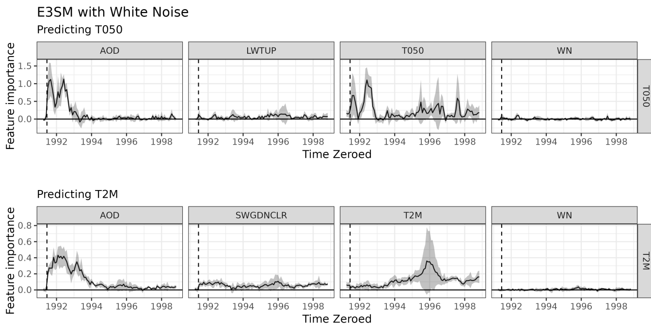
Figure C3. stZFI for E3SM with WN added as an input. Note y-axis scale differs for the two rows.
