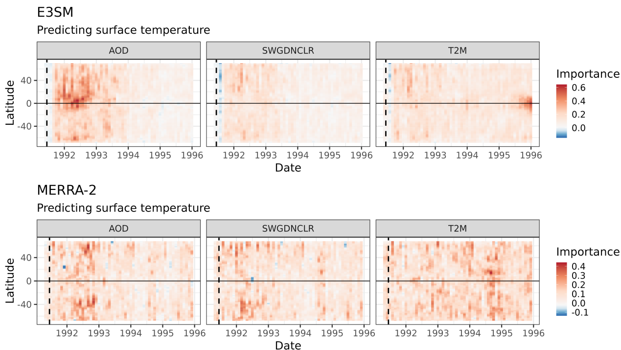
Figure 12. Latitudinal contributions to stZFI for E3SM and MERRA-2 for models predicting T2M. Note importance scales are different for E3SM and MERRA-2. Vertical dashed lines denote the June 15, 1991 Mount Pinatubo eruption.
