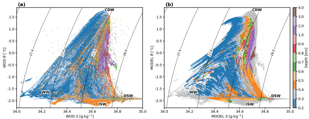
290 Figure 5. Temperature-salinity diagrams from (a) the WOD dataset and (b) the RAISE model simulation over the model domain. The major water masses are labeled, including the Dense Shelf Water (DSW), Circumpolar Deep Water (CDW), Ice Shelf Water (ISW) and Winter Water (WW).
