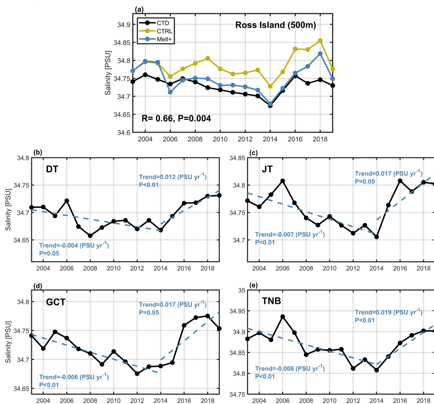
420 Figure 12. (a) Time series of summer bottom water salinity near the Ross Island from the CTRL simulation, the Melt+ simulation and CTD observations from Jacobs et al. (2022) during 2003–2019. (b–e) Time series of simulated summer bottom water salinity in CTRL at the long-term observation locations in (b) the Drygalski Trough, (c) the Joides Tough, (d) the Glamor Challenger Trough and (e) the Terra Nova Bay during 2003–2019. See the locations in Fig. 1b. The trends for the periods prior to 2014 and after 2014 with the significance test results 425 are labeled in panels b–e.
