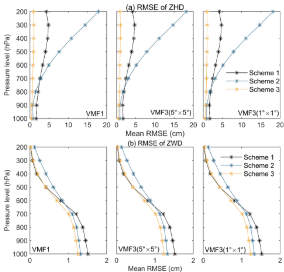
230 Figure 3 Mean RMSE of the (a) ZHD and (b) ZWD interpolated from VMF1_FC and VMF3_FC for each scheme at each pressure level in the 3-year (2020 – 2022) period at all global grid points
