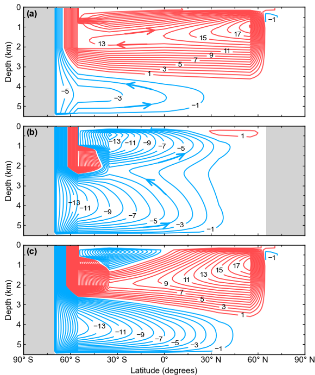
795 Figure 3. Pre-industrial, steady state model representation of the meridional overturning circulation ( S_v ) for: (a) the Atlantic Ocean, (b) the Pacific Ocean and (c) the global ocean. Red contours (positive values) represent clockwise circulation and blue contours (negative values) are for counterclockwise circulation as indicated schematically by arrows.
