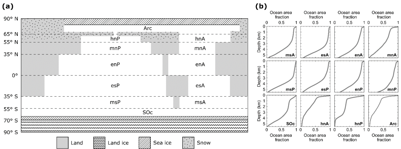
Figure 1. (a) Pre-industrial model land continental distribution and meridional boundaries of ocean boxes-sectors (dashed lines). There are twelve ocean boxes-sectors with their respective identifiers: Arc: Arctic Ocean, SOc: Southern Ocean, hn: high north, mn: mid north and en: equatorial north for Atlantic (A) and Indian-Pacific (P) Ocean. Box-Sector names in the Southern Hemisphere follow the same convention. High latitude North Pacific sector (hnP) and the Arctic Ocean are connected through the Bering Strait. Land south of 70° S is fully ice covered. Meridional sea-ice and snowline extents vary freely. (b) Observed present-day ocean area fraction profile of each ocean model box-sector calculated from Amante and Eakins (2009). 75
