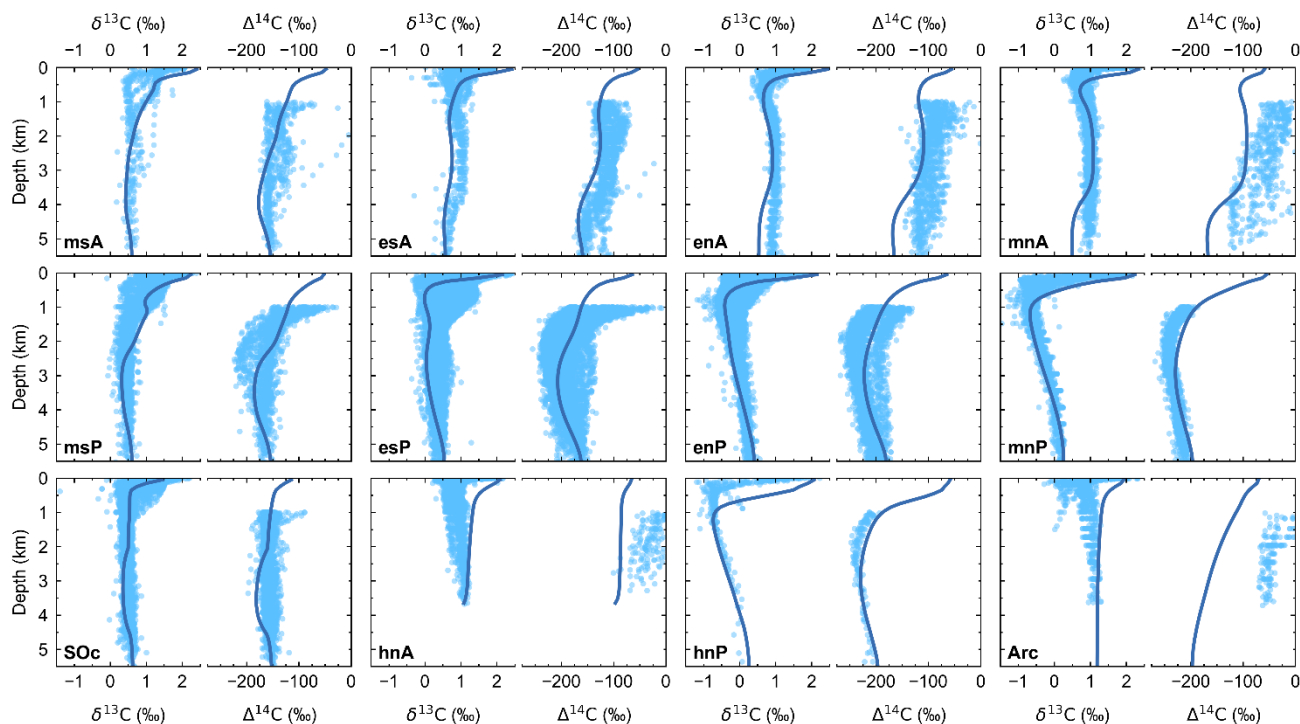
905 Figure 8. Pre-industrial, steady state model ocean vertical profiles (dark blue lines) of isotopic excursion of ^{13}\text{C} ( \delta^{13}\text{C} ) and isotopic excursion of ^{14}\text{C} ( \Delta^{14}\text{C} ) compared to observed data (light blue dots) for each ocean model box-sector shown in Fig. 1a. Observed values are from the GLODAPv2 database (Lauvset et al., 2022). For \Delta^{14}\text{C} only values below 1000 m depth have been plotted as shallower depths are strongly affected by the anthropogenic signal including atomic bomb ^{14}\text{C} inputs. Note that bomb ^{14}\text{C} also affects deeper levels in the North Atlantic and Arctic boxes-sectors (mnA, hnA and Arc).
