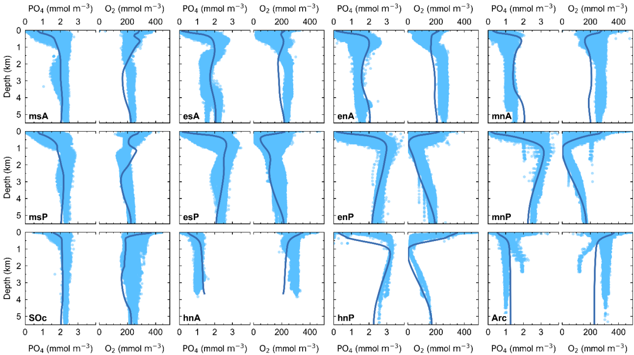
865 Figure 5. Pre-industrial, steady state model ocean vertical profiles (dark blue lines) of phosphate ( \text{PO}_4 ) and dissolved oxygen ( \text{O}_2 ) compared to observed data (light blue dots) for each ocean model box -sector shown in Fig. 1a. Observed values are from the GLODAPv2 database (Lauvset et al., 2022).
