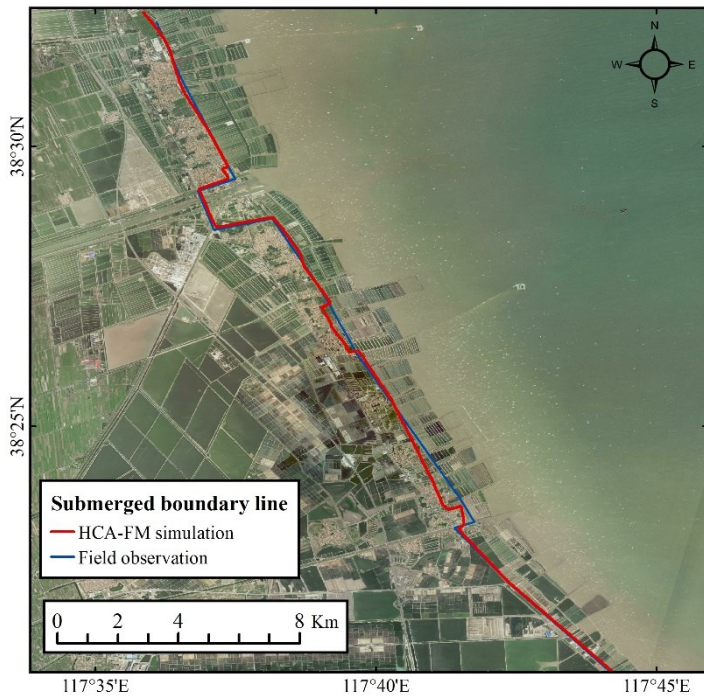
200 Figure 4: Comparison of inundation between the HCA-FM simulation and field observation in Cangzhou, Hebei during Typhoon Lekima; red line represents submerged boundary line simulated by the HCA-FM and blue line by field survey (Base map by Esri, Maxar, Earthstar Geographics, and the GIS User Community).
