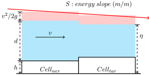
90 Figure 1: Illustration of hydrodynamic structure between the target cell and neighbor cell.
