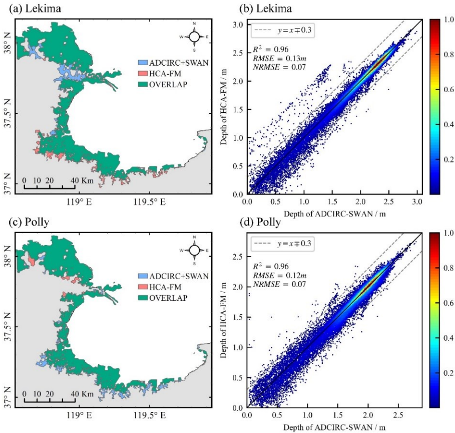
280 Figure 6: Comparison between the HCA-FM and ADCIRC+SWAN models. (a) & (c) Comparison of flood extent during Typhoons Lekima and Polly, respectively; (b) & (d) scatter plot of ADCIRC+SWAN versus HCA-FM simulated water depth during Lekima and Polly, respectively.
