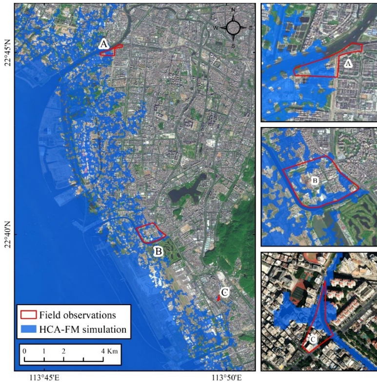
Figure 5: Comparison of inundation in three survey sites (A, B, C) on the west coast of Shenzhen, Guangdong during Typhoon Hato; blue region represents flood extent simulated by the HCA-FM and red polygons represent survey regions being submerged (Base map by Esri, Maxar, Earthstar Geographics, and the GIS User Community).
