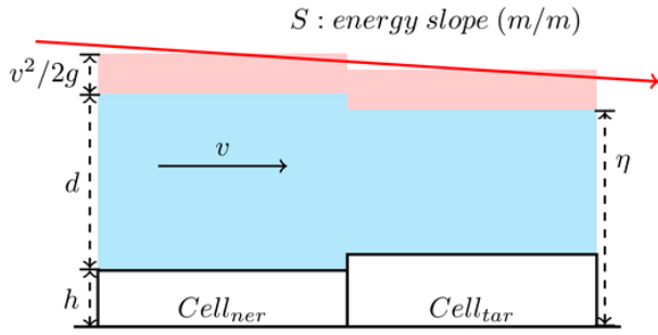
95 Figure 1: Illustration of hydrodynamic structure between the target cell and neighbor cell.
