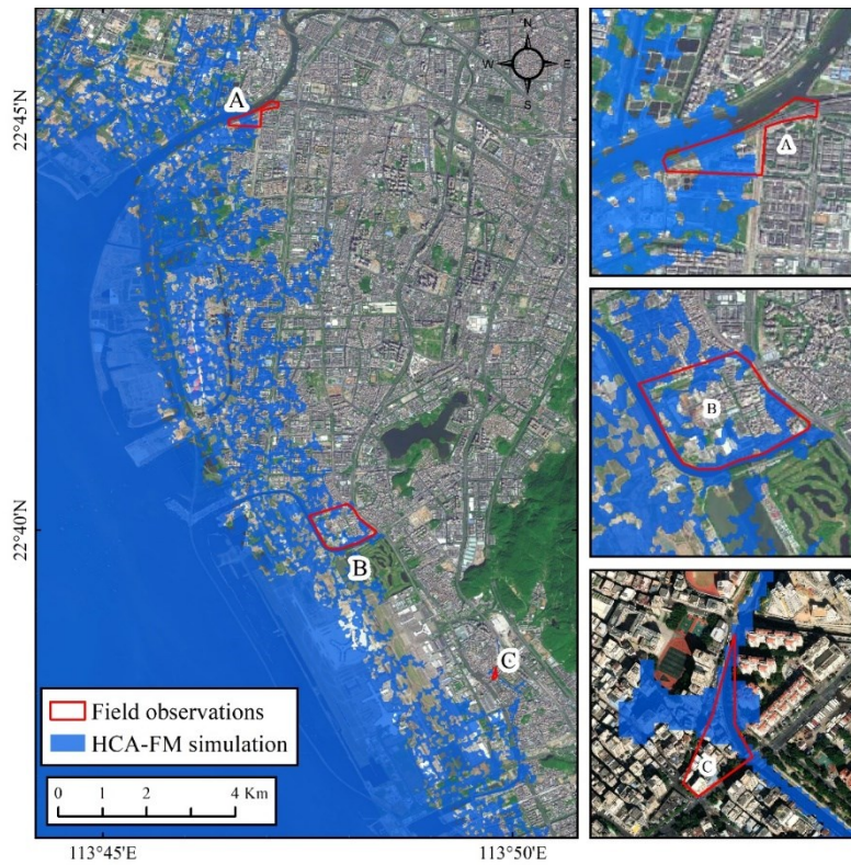
225 Figure 5: Comparison of inundation in three survey sites (A, B, C) on the west coast of Shenzhen, Guangdong during Typhoon Hato; blue region represents flood extent simulated by the HCA-FM and red polygons represent survey regions being submerged (Base map by Esri, Maxar, Earthstar Geographics, and the GIS User Community).
