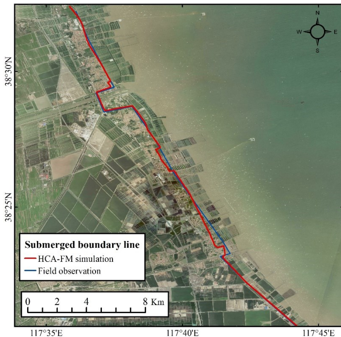
210 Figure 4: Comparison of inundation between the HCA-FM simulation and field observation in Cangzhou, Hebei during Typhoon Lekima; red line represents submerged boundary line simulated by the HCA-FM and blue line by field survey (Base map by Esri, Maxar, Earthstar Geographics, and the GIS User Community).
