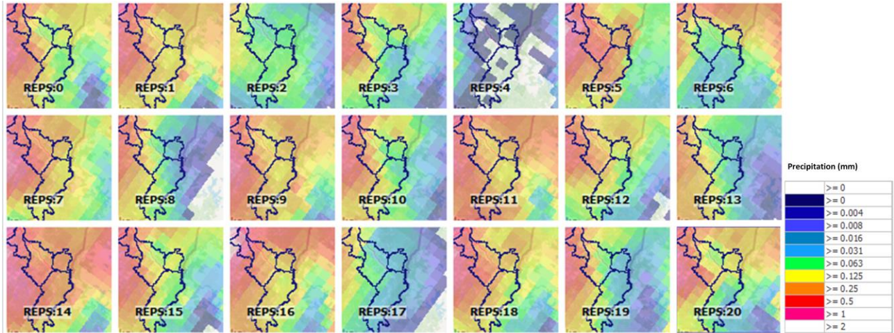
Figure 4: Members of REPS precipitation (in mm) for the 24-01-2019. Figure adapted from Montero et al. (2023).
