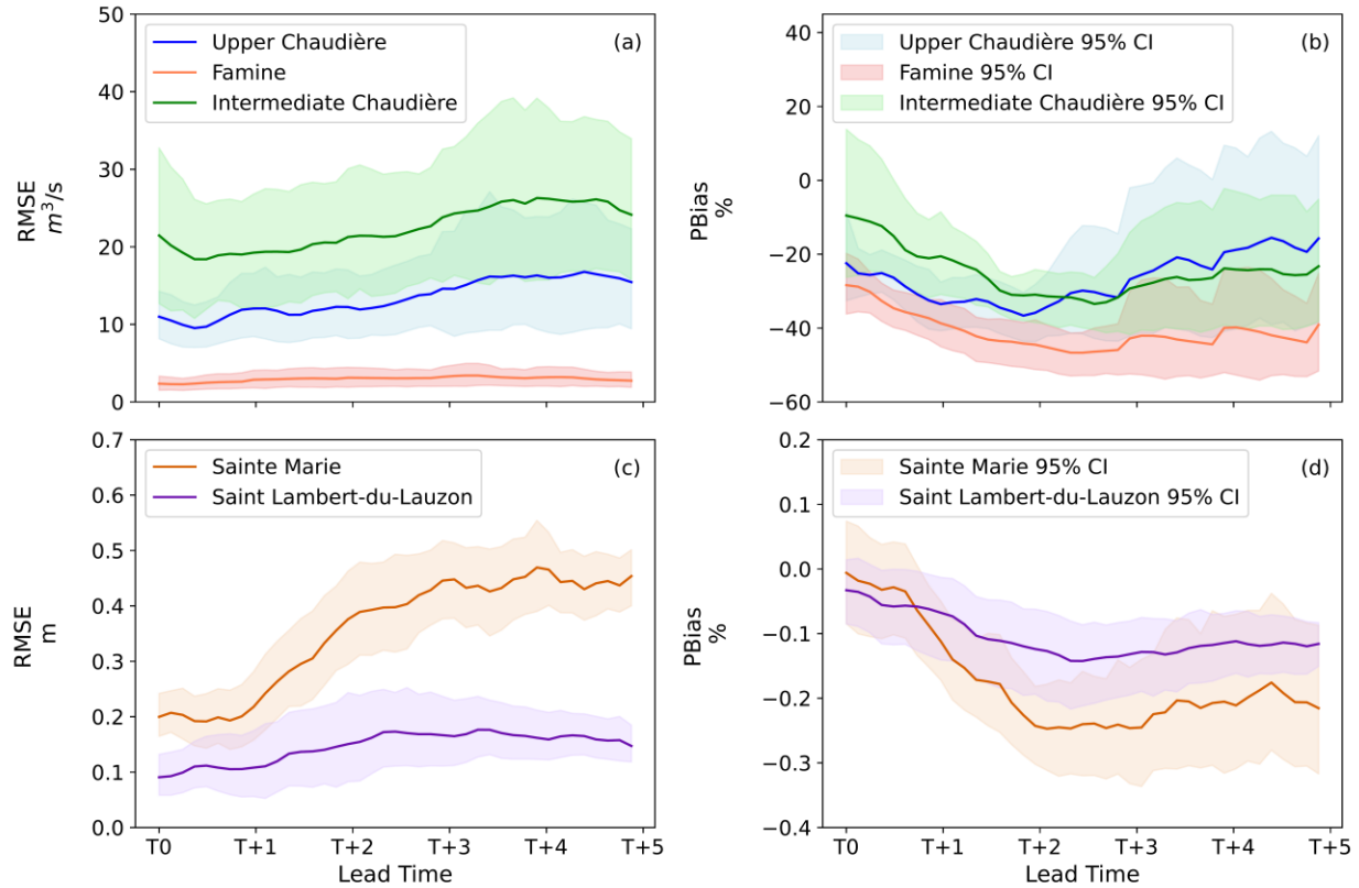
Figure 14: Performance evaluation of the coupled modelling system using RMSE and PBias scores. The top panel (subplots (a) and (b) represents the results of hydrologic module, while the bottom panel (subplots (c) and (d) represents the results of hydraulic module.
