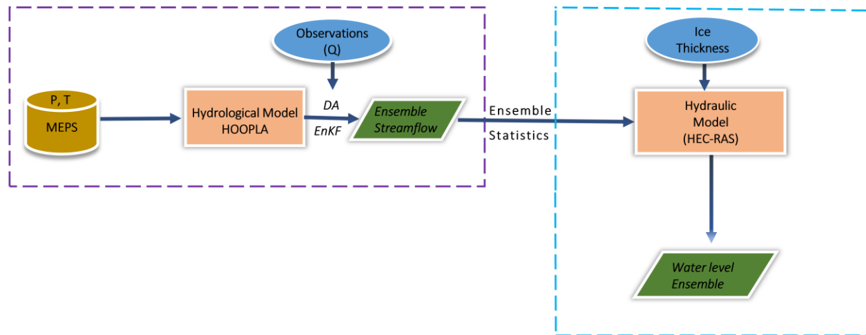
Figure 3 A schematic overview of methodology followed for probabilistic forecasting of under ice discharge. P is precipitation, T is air temperature, Q is discharge. Meteorological data is input to the hydrological modelling framework HOOPLA to produce a streamflow ensemble. Data Assimilation (DA) is implemented through the Ensemble Kalman filter (EnKf) inside HOOPLA. The streamflow ensemble is post processed for ensemble statistics and run through a river ice hydraulic model that produces a water level ensemble.
