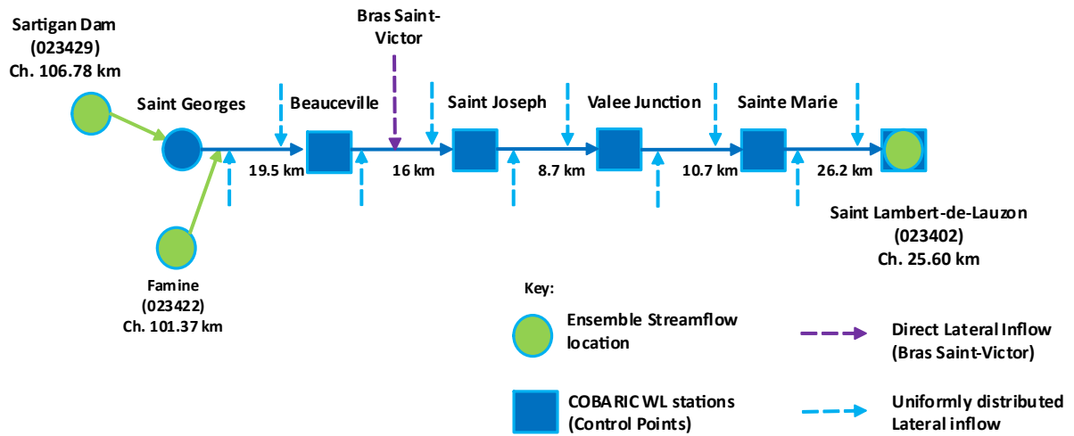
Figure 5: Schematic of the 1D unsteady river ice Hydraulic model setup in HEC-RAS for the Intermediate Chaudière reach. The green circles represent ensemble streamflow locations obtained from the hydrological module of the system. The blue squares represent the water level control points located along the reach.
