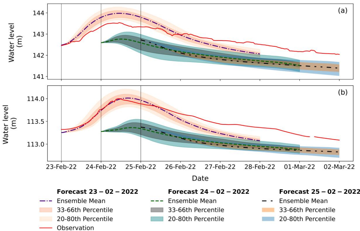
Figure 13 Ensemble water level forecast at Sainte Marie (subplot (a)) and Saint Lambert-du-Lauzon (subplot (b)) stations along the Chaudière River for forecasting on February 23, 24 and 25, 2022. The grey vertical lines in the subplots correspond to the issue time of each forecast.
