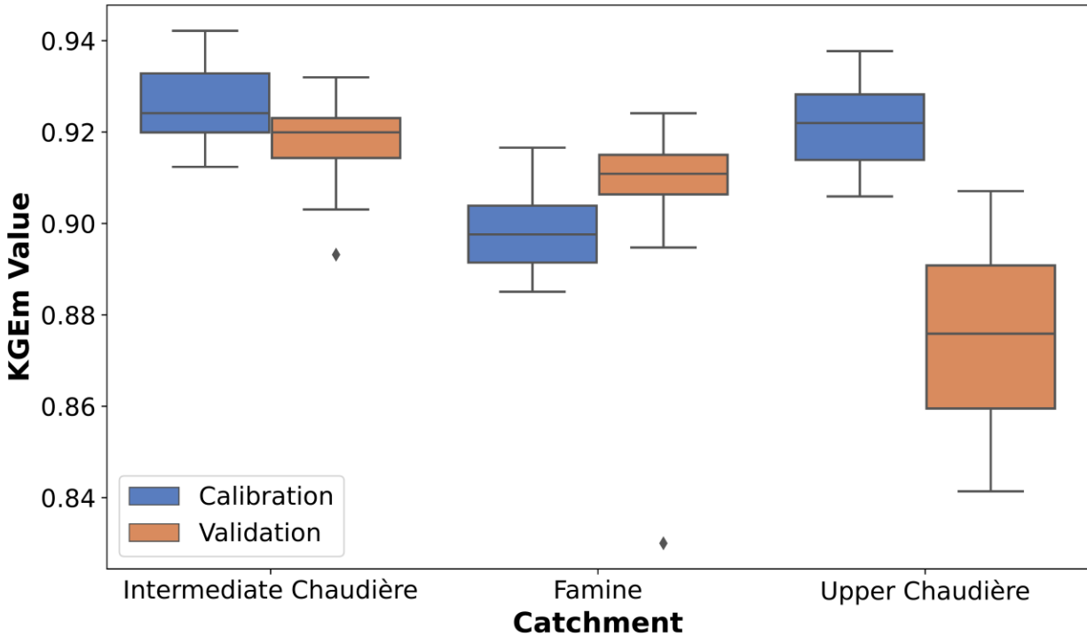
Figure 11: Boxplot showing the modified Kling-Gupta Efficiency (KGEm) distribution of all 20 hydrological models in HOOPLA framework for each catchment during calibration and validation periods.
