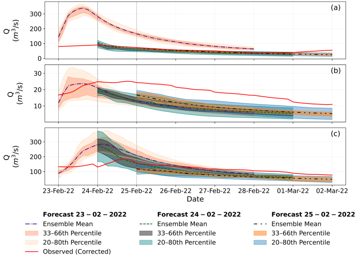
Figure 12: Ensemble hydrologic forecast evolution for February 23, 24 and 25, 2022 at the three sub-catchments of the Chaudière River. The grey vertical lines in the subplots correspond to the issue time of each forecast. The subplots (a), (b) and (c) show the hydrological forecasts at Upper Chaudière, Famine and Intermediate Chaudière respectively.
