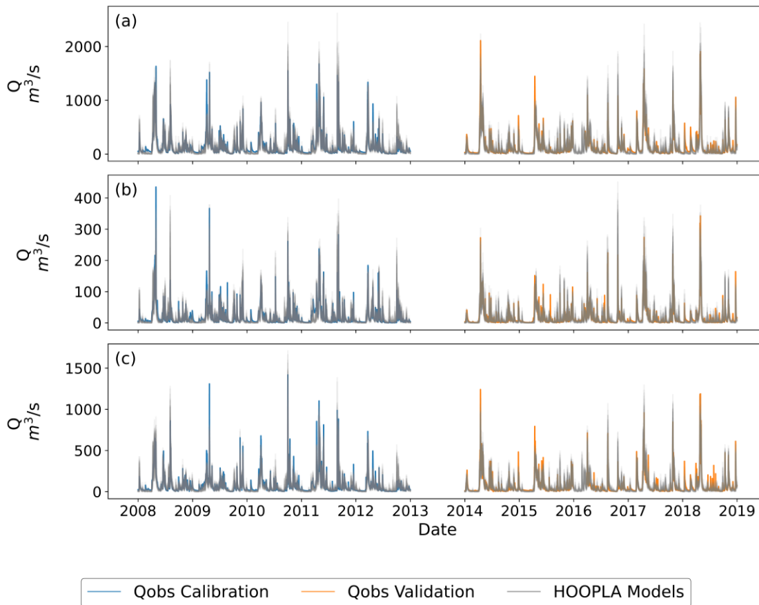
Figure 10: Calibration and validation of HOOPLA framework performed on the three sub-catchments defined in the Chaudière River Basin. Subplot (a) shows the results for the Intermediate Chaudière sub-catchment, subplot (b) shows the results for the Famine sub-catchment, and subplot (c) shows the results for the Upper Chaudière sub-catchment.
