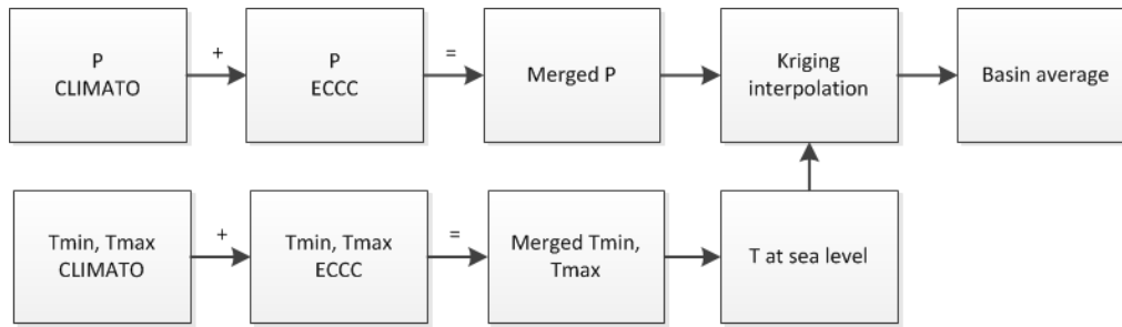
Figure 7: Preprocessing of observed data to create inputs for hydrological historical update runs. P is precipitation and T is air temperature. Figure adopted from Montero et al. (2023).
