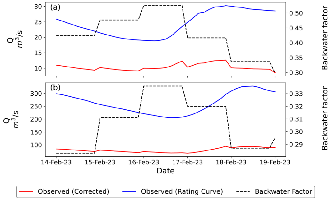
Figure 2: Example of correction of instantaneous hydrograph using daily backwater flow factors calculated by MELCCFP for Famine (subplot (a)) and Saint Lambert-de-Lauzon (subplot (b)) stations.
