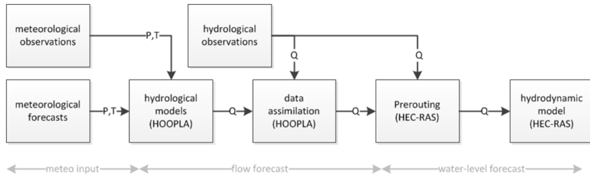
Figure 6: Schematic overview of workflow for the hydrological forecasts. P is precipitation, T is air temperature, Q is discharge. Figure adapted from Montero et al. (2023).
