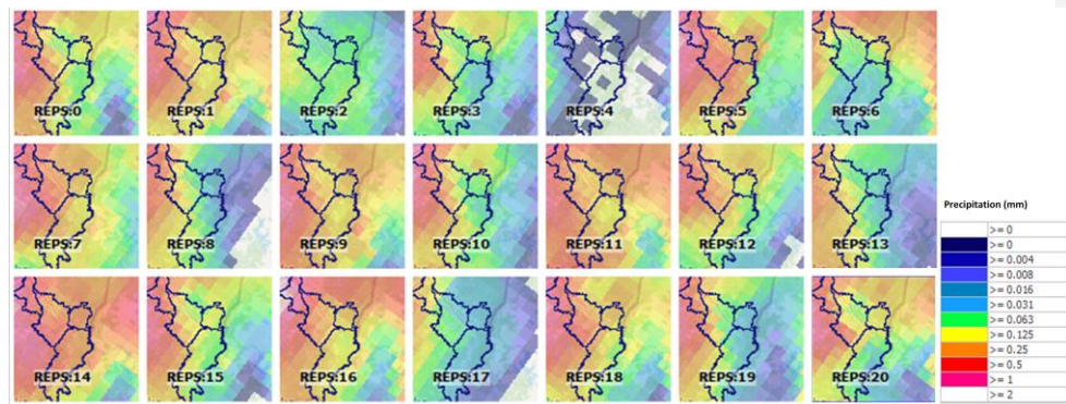
Figure 4: Members of REPS precipitation (in mm) for the 24-01-2019. Figure adapted from Montero et al. (2023).
