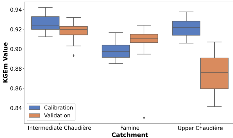
Figure 11: Boxplot showing the modified Kling-Gupta Efficiency (KGE) distribution of all 20 hydrological models in HOOPLA framework for each catchment during calibration and validation periods.
