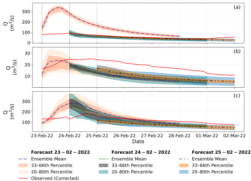
Figure 12: Ensemble hydrologic forecast evolution for February 23, 24 and 25, 2022 at the three sub-catchments of the Chaudière River. The grey vertical lines in the subplots correspond to the issue time of each forecast. The subplots (a), (b) and (c) show the hydrological forecasts at Upper Chaudière, Famine and Intermediate Chaudière respectively.
