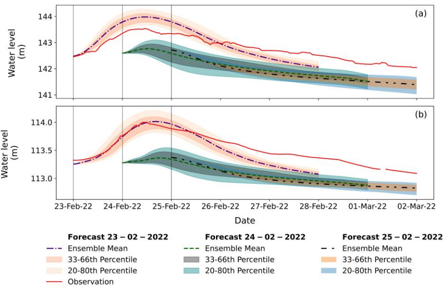
655 Figure 13 Ensemble water level forecast at Sainte Marie (subplot (a)) and Saint Lambert-du-Lauzon (subplot (b)) stations along the Chaudière River for forecasting on February 23, 24 and 25, 2022. The grey vertical lines in the subplots correspond to the issue time of each forecast.
