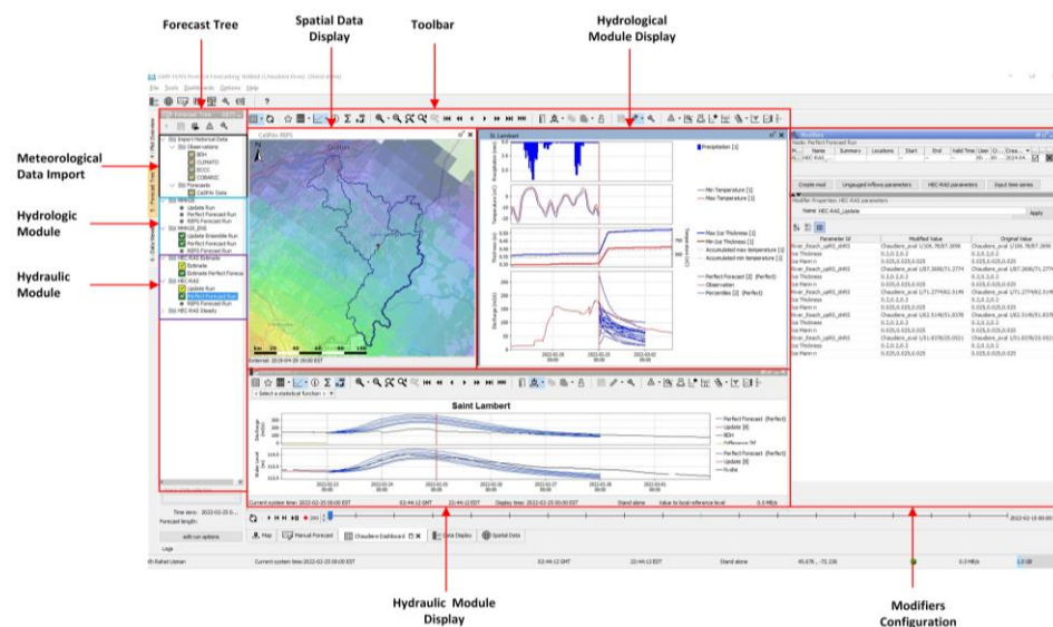
Figure 8: A screenshot of the Delft-FEWS River Ice Forecasting testbed system for the Chaudière River.
