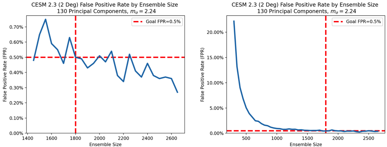
Figure 20. Experimental FPR for the UF-ECT when used with the CESM 2.3 model, N_{PC} = 130 , and m_\sigma = 2.24 . The effects of PCA variance estimation bias can be clearly seen in the right-hand plot. While sufficient ensemble size is key to reduce the FPR, there is a diminishing benefit to very large ensembles. Plots represents mean of 10,000 trials at each ensemble size and display the same data with different axis ranges.
