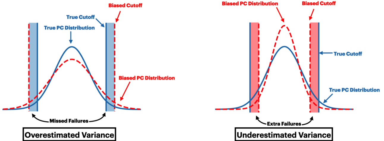
Figure 5. True PC distributions are in blue and estimated PC distributions are in red. Vertical lines represent true and estimated m_\sigma . If the estimate of a PC variance is overestimated (as in the left figure) the ECT will miss failures that occur in the blue region. Alternatively, if the estimate of variance is underestimated (as in the right figure) the ECT will return additional false positive failures in the red region. Importantly, the effects of different directions of PC bias (as in Figure 4) do not cancel each other out.
