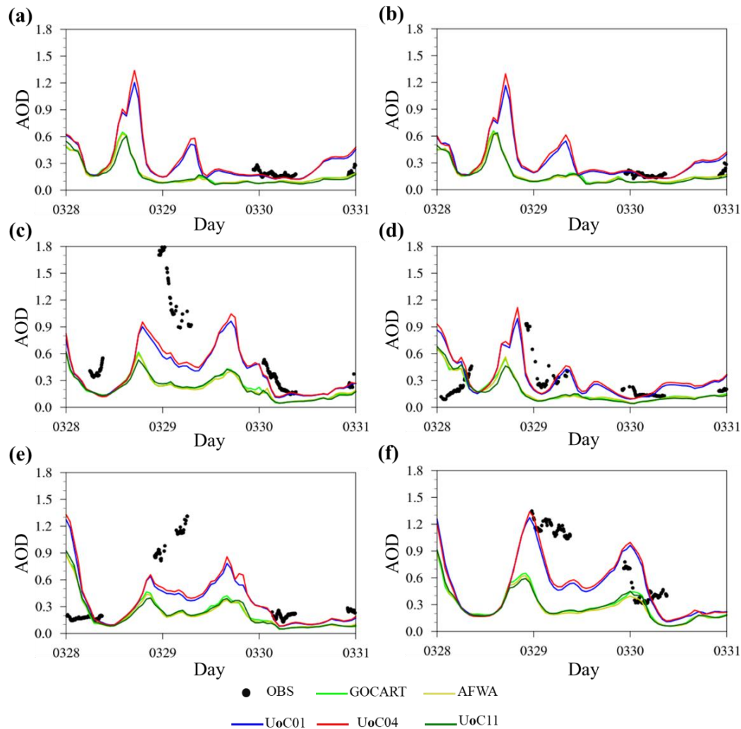
Figure 9: Hourly time series of AERONET and simulated AOD in (a) Yonsei University, (b) Seoul, (c) Gwangju, (d) Gangneung, (e) Ulsan, and (f) Gosan in South Korea. The black dots represent AERONET AOD values, and the colored lines depict various
