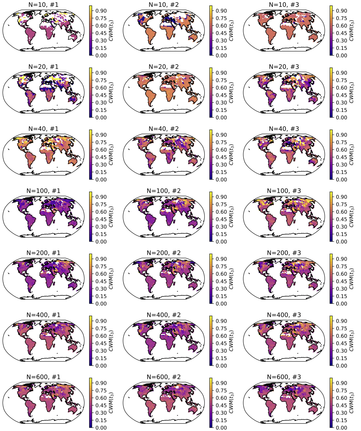
Figure 1: Global distribution of CWM(t_3) of tree strategies for the three ensemble members at different potential diversity. A value of t_3 closer to zero indicates that a strategy can start the growing season at lower air temperatures compared to one with a t_3 value closer to one (see Eq. (13)).
