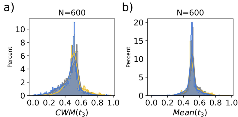
Figure 2 The abundance distribution of (a) CWM( t_3 ) and (b) Mean( t_3 ) from all grid cells at 600 strategies for each ensemble member.
