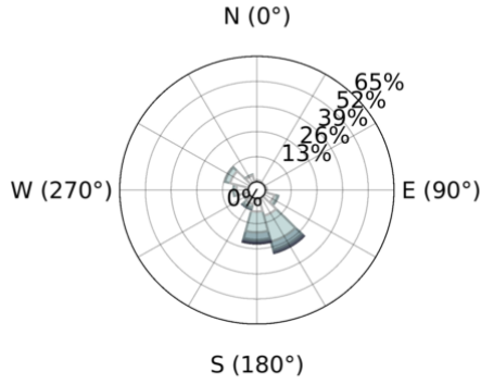
(c) NZWAVE
