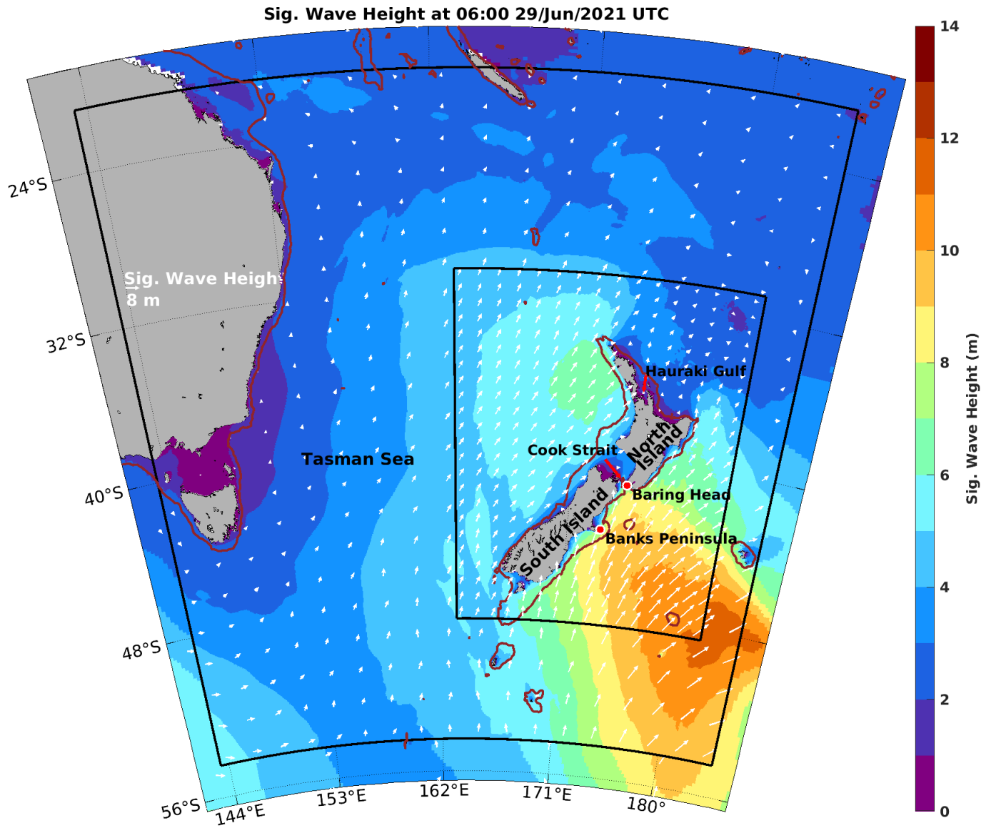
Figure 1. (a) Nested model domains and respective forecasted wave fields for 6 am UTC 29 of Jun 2021. Colour shade represents significant wave height from each domain. Global model outputs are shown as the most external colour shade. Basin scale model outputs are shown inside the largest black contour area. The innermost contour highlights the area of the high-resolution model around the mainland of Aotearoa New Zealand. The white arrows show wave height and peak wave direction plotted every 40th grid point. The red circles are the location of in situ measurements from wave buoys at Banks Peninsula and Baring Head (the northernmost red dot in this figure). The 200-m isobath is shown as a dark red contour.
