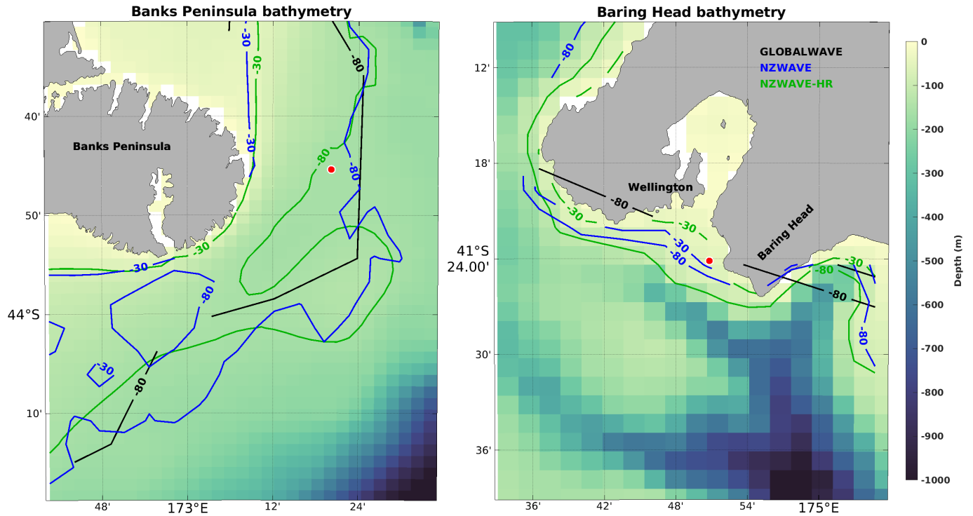
Figure 2. Model bathymetries at Banks Peninsula (a) and Baring Head (b) showing locations of wave buoy measurements (red dots). NZWAVE-HR bathymetry is displayed using the colour shade and green contour. The 30- and 80-m isobaths from NZWAVE (blue) and GLOBALWAVE (black) are also shown for comparison.
