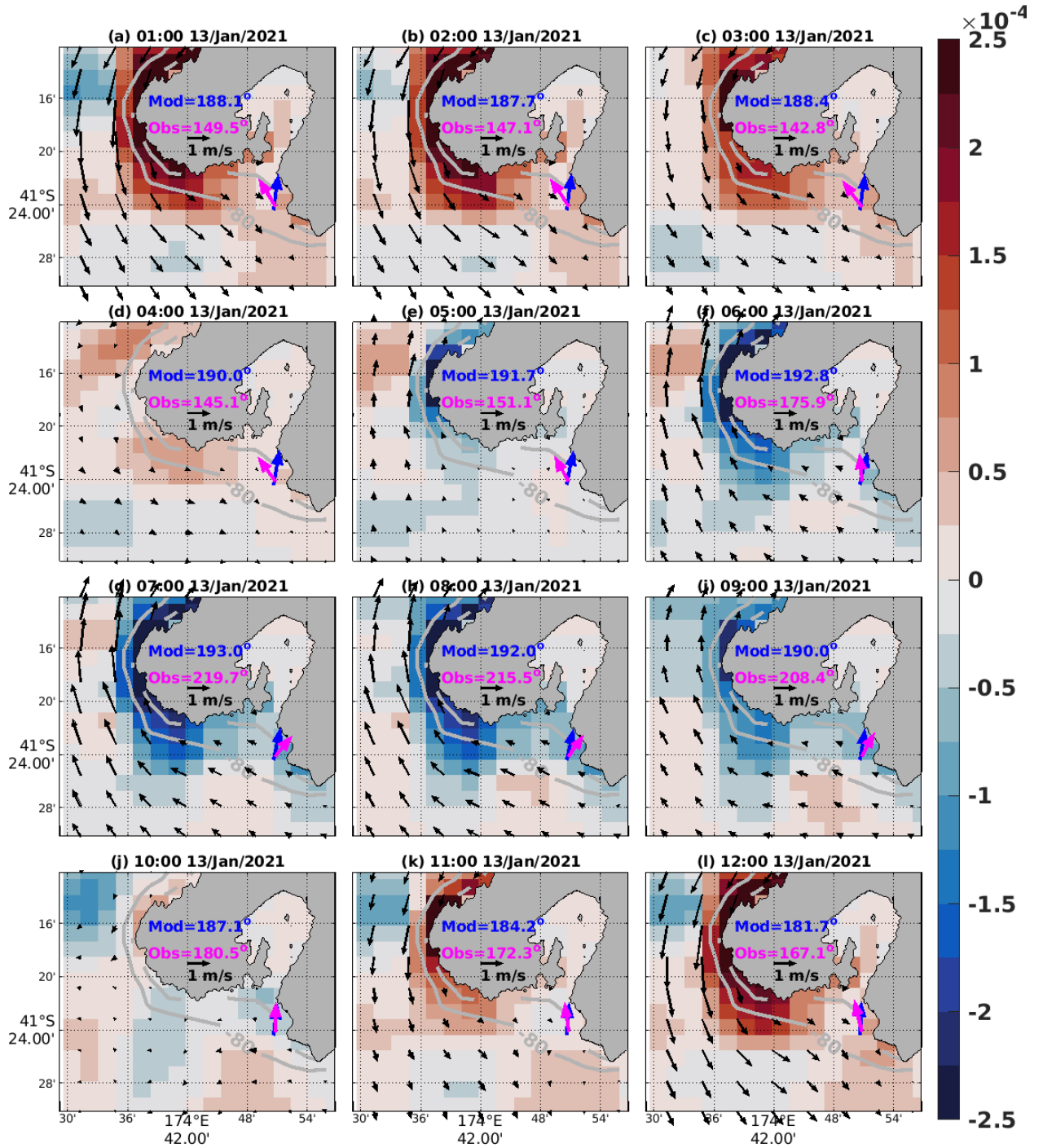
Figure 12. Hourly maps of ocean currents in m/s (black arrows) and relative vorticity ( s^{-1} , red and blue shade) from NZTIDE. Observed (magenta arrow) and NZWAVE-HR-predicted (blue arrow) significant wave height and peak direction at different times on the 13th of January 2021 at Baring Head. Observed and predicted (NZWAVE-HR) peak direction for each time frame are written for reference. Model wave variables are extracted from the closest grid point to the observations.
