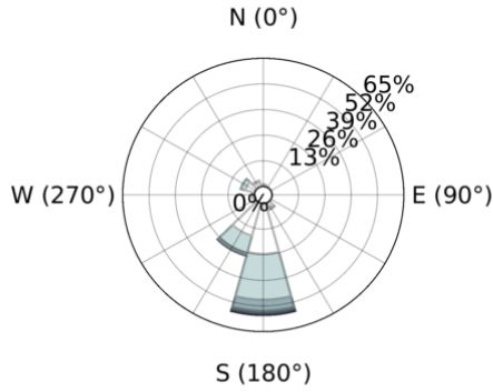
(e) NZWAVE-HR-NOTIDES
