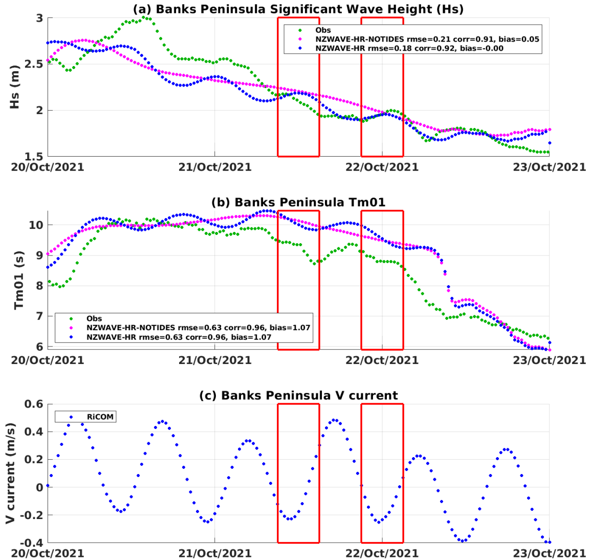
Figure 9. Timeseries of significant wave height (a), first-order mean period ( Tm01 ) and depth-averaged meridional currents (c) at Banks Peninsula from buoy measurements (green), NZWAVE-HR-NOTIDES (magenta) and NZWAVE-HR (blue). RMSE, correlation coefficient and bias are presented next to each experiment label in the legend. Those statistical metrics were computed for the period shown in the figure.
