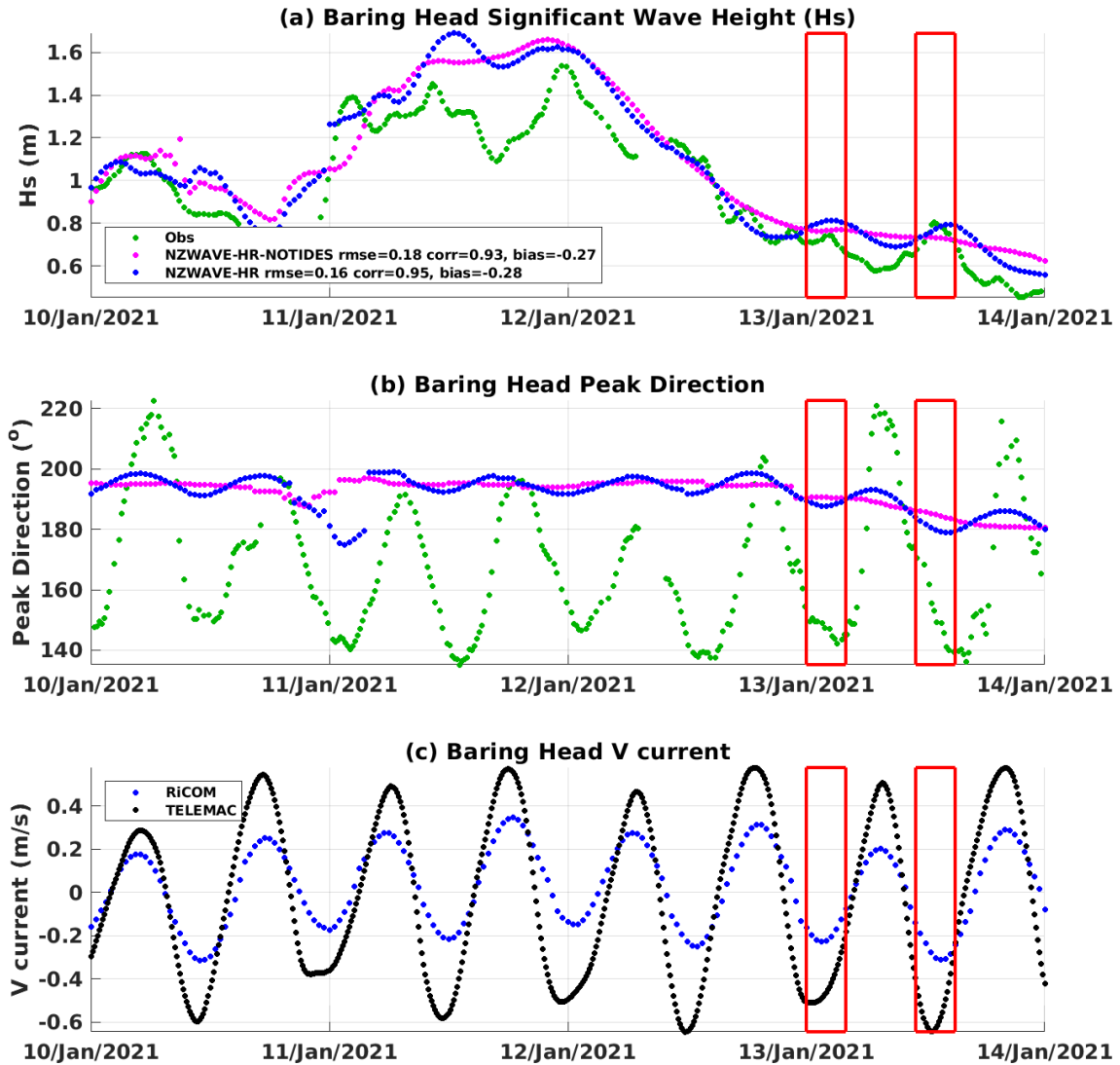
Figure 11. Timeseries of significant wave height (a), peak direction and depth-averaged meridional currents (c) at Baring Head from buoy measurements (green), NZWAVE-HR-NOTIDES (magenta) and NZWAVE-HR (blue). In (c), black dots represent depth averaged currents from TELEMAT. RMSE, correlation coefficient and bias are presented next to each experiment label in the legend. Those statistical metrics were computed for the period shown in the figure.
