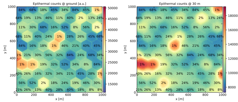
Figure 4. Simulated counts of epithermal neutrons near the ground (1-2 m, left) and at 30 m (right) in hexland_tracks , an artificial landscape with maximized heterogeneity. The black annotations indicate the soil moisture of the top layer prescribed to the hexagons.
