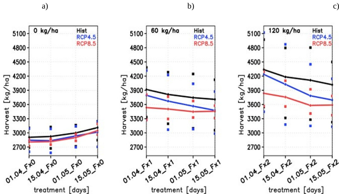
Fig. 5 Simulated Harvest (kg/ha) under Hist (black), RCP4.5 (blue) and RCP8.5 (red) scenarios, for four sowing dates across three fertilization levels (Table 1a): 0 (a), 60 (b), and 120 (c) kg N/ha (from left to right). The maximum and minimum value over the ensemble members for each treatment and climate is shown (dots) and the lines represent the ensemble means.
