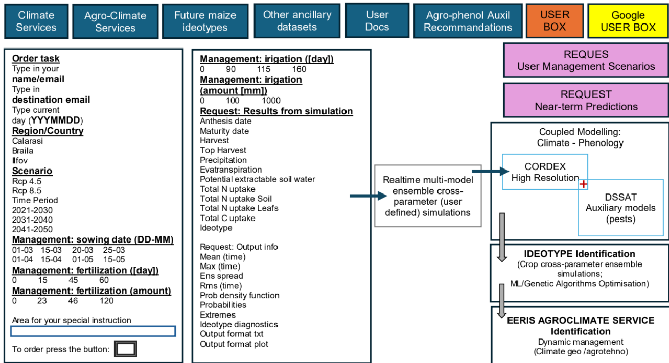
Fig. 1 a): Info-Platform: Provides local-regional scale information derived from high-resolution regional climate models (CORDEX), e.g. climate, agro-climate data and indicators, indices of agro-climate extremes at the NUTS3 level. b): User-Platform for adaptation support: Processes in real time specific user requests, and simulates management scenarios, identifying optimal paths: Users input parameters (left, e.g: region, period (present / future climate scenarios), management options (e.g. sowing date, fertilization/irrigation time and amount,
