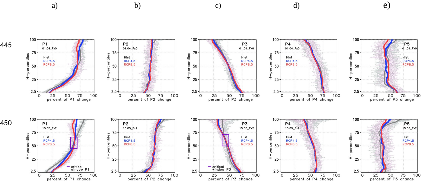
Fig. 8 Parameters' values corresponding to percentiles of the H distribution (ordered from maximum to minimum H value). On X axis is the percent of parameter change (increase) relative to the maximal change tested for each, normalised to its control value. The figure compares these percentiles for Hist (black), RCP4.5 (blue) and RCP8.5 (red), running mean values (full lines, 100 values window), ensemble mean, time-mean; unsmoothed values are shown by dots only for Hist (grey shade) and RCP8.5 (pink shade), the RCP4.5 values being generally intermediate. Percentiles are from a number of 1890 genotype simulations. These are shown for two treatments (01.04_Fx0 at top and 15.05_Fx2 at bottom). The plum rectangle indicates a critical parameter range for P1 and P3 (text) defined as \pm 5\%H around threshold values (the parameter value at the intersection between scenario and H curves). Thresholds are defined as the (neutral) value of the parameter for which the same H-percentile is reached in scenario and Hist. Thresholds control the limit parameter values for which the scenario leads better/ worse H percentiles than in Hist.
