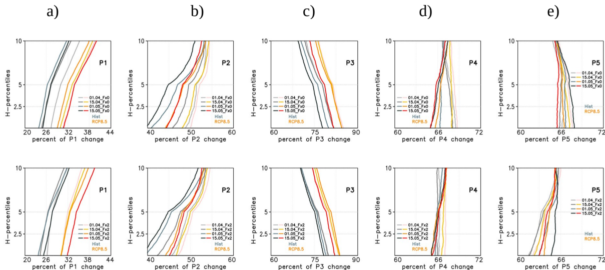
Fig. 9 As in Fig. 8 but for all sowing dates, no fertilization Fx0 (top) and with fertilization Fx2 (bottom). Parameters are shown for the top 10% highest harvest. On X axis is the percent of parameter change relative to the interval tested for each. Grey colours are for Hist and yellow-red for RCP8.5 (light to dark is from earlier to latest sowing).
