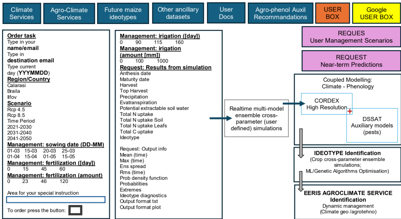
235 Fig.1 a): Info-Platform: Provides local-regional scale information derived from high-resolution regional climate models (CORDEX), e.g. climate, agro-climate data and indicators, indices of agro-climate extremes at the NUTS3 level. b): User-Platform for adaptation support: Processes in real time specific user requests, and simulates management scenarios, identifying optimal
