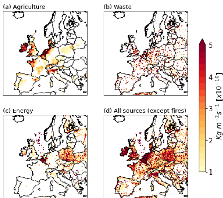
Figure 2. Spatial distribution of EDGARv6.0 CH 4 emission rates for the concerned key sectors for May 2018 in the 30 km modeling domain. Each grid point in panel (d) represents the sum of emission rates from all different sectors (except biomass burning) based on country-specific temporal profiles.
