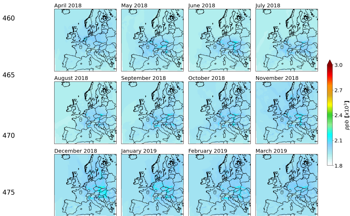
Figure 5. Monthly mean spatial distributions of simulated CH 4 concentration interpolated to roughly 100 m (shaded), 480 together with monthly mean CH 4 concentrations from the ICOS sites with sampling heights of 100 m (circles), both data sets averaged over the period from April 1, 2018 to March 31, 2019. The concentrations are in ppb and were computed based on quality-controlled ICOS CH 4 data for all stations simultaneously.
