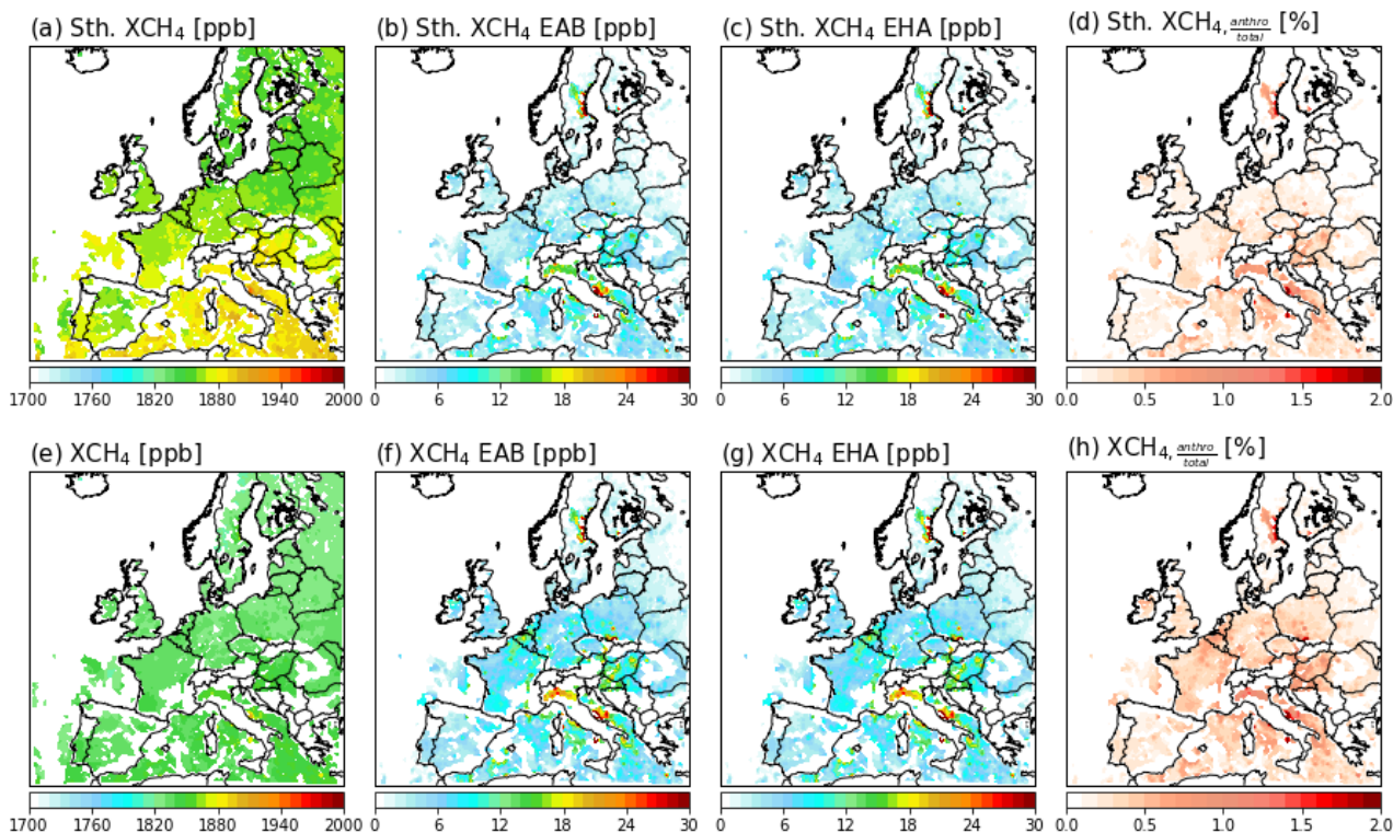
620 Figure 8. Temporal mean spatial distributions with and without smoothing of simulated XCH 4 concentration (panels (a) and (e)), XCH 4 enhancement above background (EAB) (panels (b) and (f)), XCH 4 enhancement from human activities (EHA) (panels (c) and (g)), and contribution of anthropogenic sources to the XCH 4 concentration (panels (d) and (h)). Concentrations were averaged for grid points with satellite measurements during the period from May 1 to August 31, 2018, months with the best model performance for smoothed concentrations (see Fig. 4).
