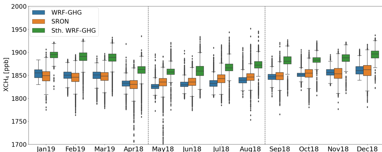
Figure 7. Monthly boxplots of observed and simulated XCH 4 concentrations with and without smoothing for the period from 555 April 01, 2018 to March 31, 2019. The months from May to August of 2018 (between dashed lines) were selected for model evaluation of the contribution of anthropogenic sources to the XCH 4 concentration, discussed ahead in section 4.
