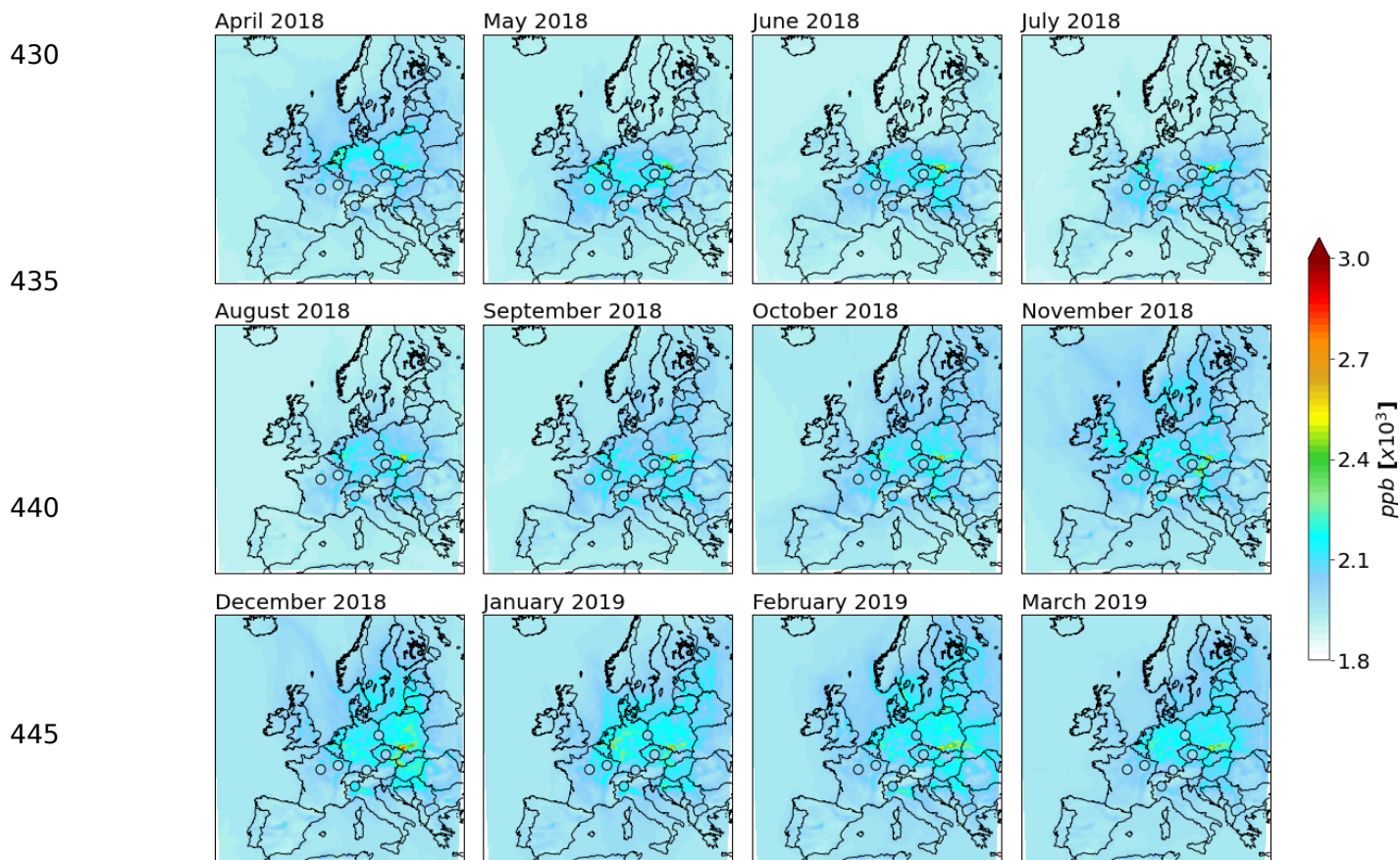
450 Figure 4. Monthly mean spatial distributions of simulated CH 4 concentration interpolated to roughly 50 m (shaded), together with monthly mean CH 4 concentrations from the ICOS sites with sampling heights between 40 and 50 m (circles), both data sets averaged over the period from April 1, 2018 to March 31, 2019. The concentrations are in ppb and were computed based on quality-controlled ICOS CH 4 data for all stations simultaneously.
