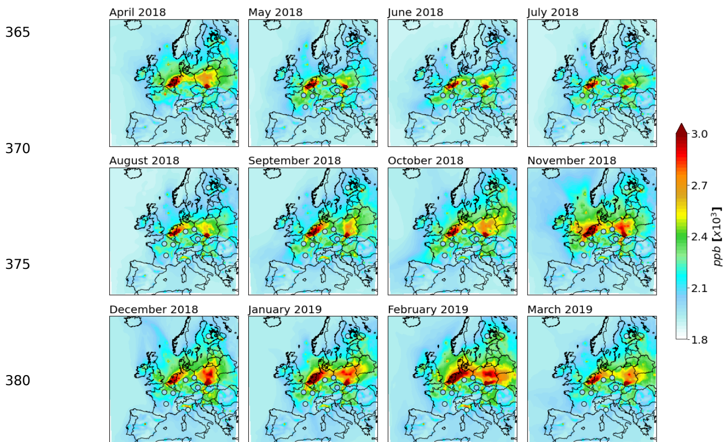
385 Figure 3. Monthly mean spatial distributions of simulated CH 4 concentration interpolated to roughly 10 m (shaded), together with monthly mean CH 4 concentrations from the ICOS sites with sampling heights between 8 and 16.8 m (circles), both data sets averaged over the period from April 1, 2018 to March 31, 2019. The concentrations are in ppb and were computed based on quality-controlled ICOS CH 4 data for all stations simultaneously.
