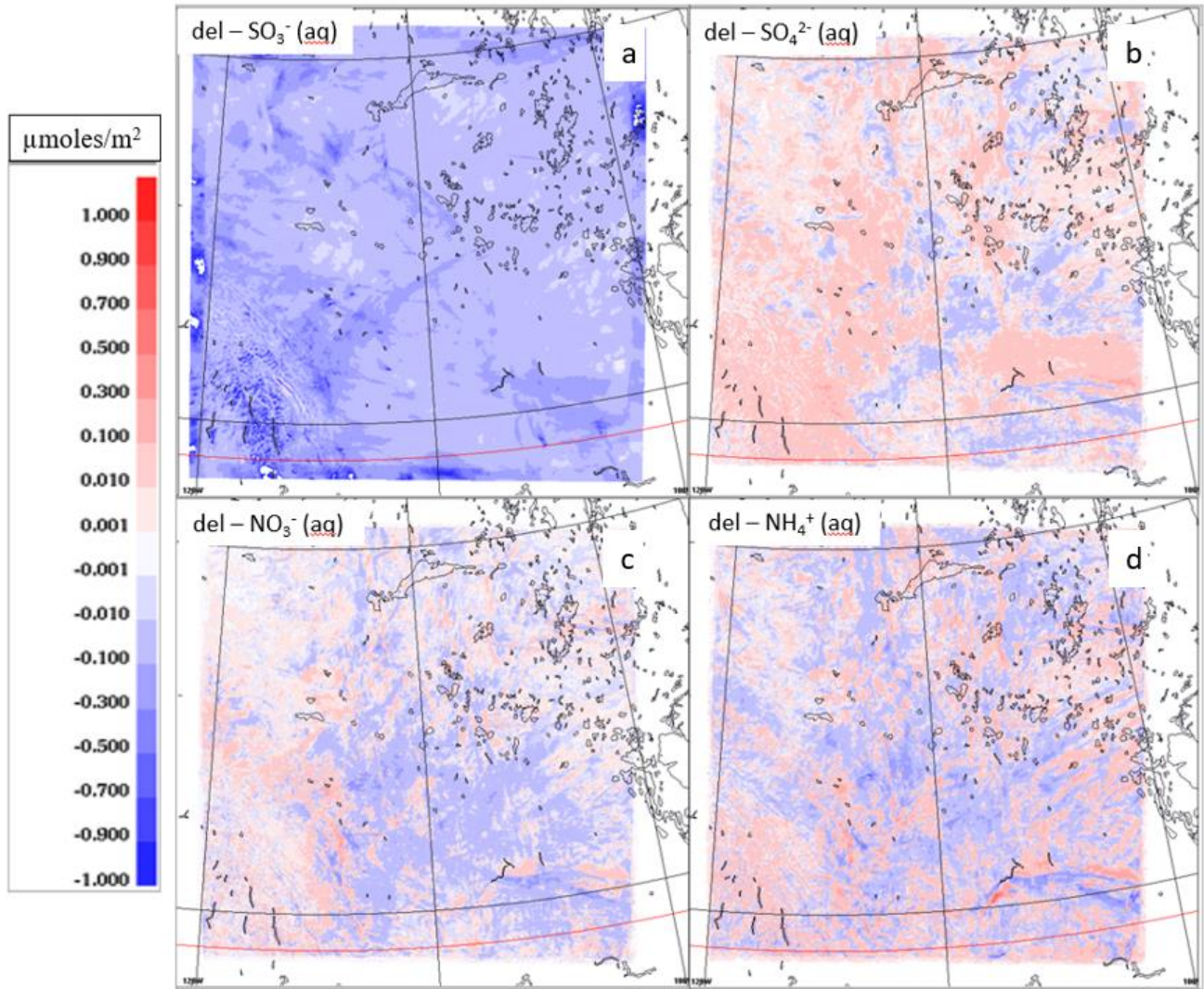
870 Figure 8: The net differences of hourly accumulated mean deposited flux of \text{SO}_3^- , \text{SO}_4^{2-} , \text{NH}_4^+ and \text{NO}_3^- for the multi-phase and base-case experiments (e.g. multi-phase – base-case) over April 2018. Domain-mean deposition values are \text{SO}_3^- = 0.123 (9.84), \text{SO}_4^{2-} = 0.083 (7.970), \text{NO}_3^- = 0.139 (7.645), \text{NH}_4^+ = 0.377 (4.147) \mu\text{mol}/\text{m}^2 ( \mu\text{g}/\text{m}^2 ) for base-case, and \text{SO}_3^- = 0.015 (1.20), \text{SO}_4^{2-} = 0.089 (8.54), \text{NO}_3^- = 0.135 (7.42), \text{NH}_4^+ = 0.371 (4.081) \mu\text{mol}/\text{m}^2 ( \mu\text{g}/\text{m}^2 ) for multi-phase experiment.
