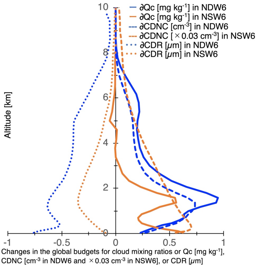
Figure 14: Global budgets of the annual averages of the NDW6- and NSW6-simulated Q_c (mixing ratio of cloud droplets), the NDW6-simulated CDNC, the NSW6-simulated CDNC (which is equal to CCN number concentrations), and the NDW6- and NSW6-simulated CDR (cloud droplet effective radius for warm clouds)
