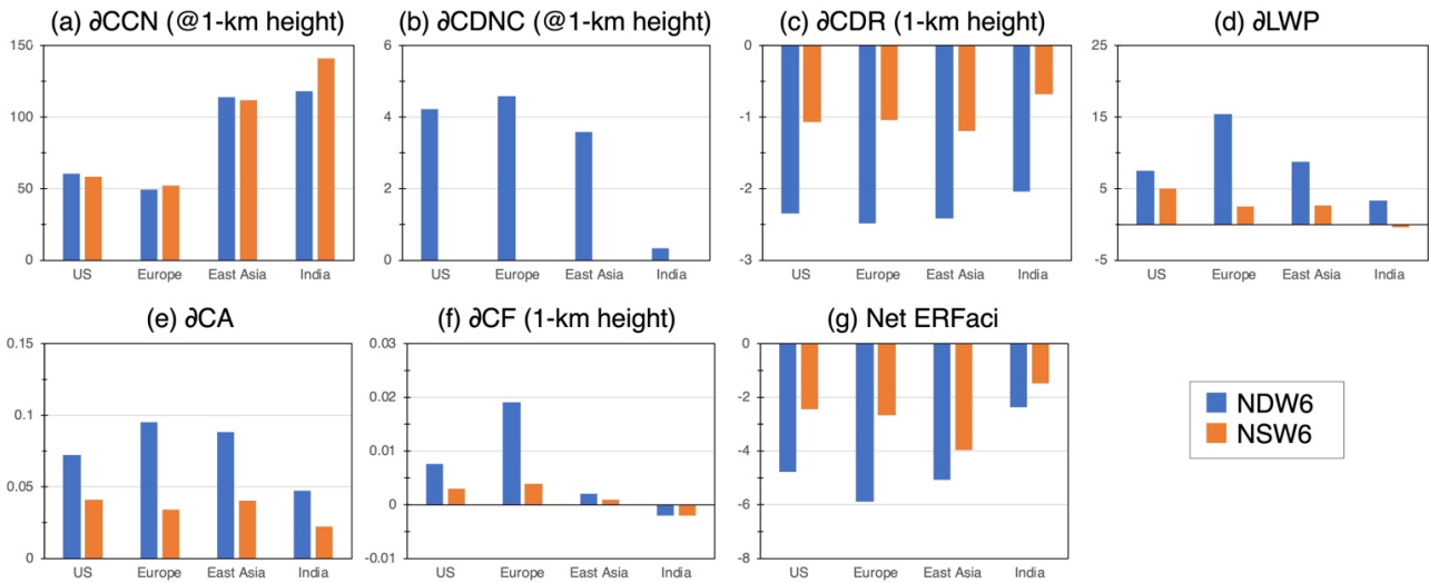
1305 Figure 13: Regional averages of the differences in CCN at 1-km height, CDNC (only in NDW6), CDR at 1-km height, LWP, CA, CF at a 1-km height, and net ERFaci between the preindustrial and the present days. The regions are defined as US (90°W-60°W, 30°N-50°N), Europe (0°E-30°E, 40°N-60°N), East Asia (110°E-140°E, 20°N-50°N), and India (70°E-90°E, 10°N-35°N).
