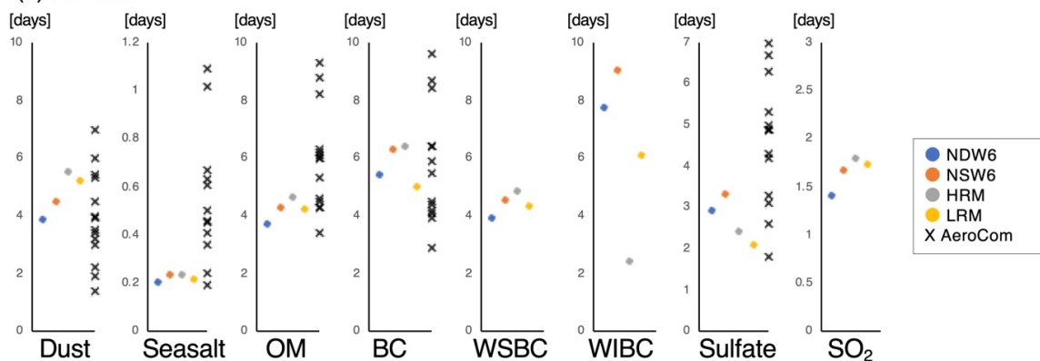
Figure 5: Global and annual mean values of (a) column burdens [Tg or TgS], (b) emission fluxes [Tg yr -1 or TgS yr -1 ], and (c) atmospheric lifetimes of the simulated aerosols and SO 2 [days]. The results include NDW6 and NSW6 in this study and references for the HRM and LRM in Goto et al. (2020) and AeroCom (Gliß et al., 2021). The values are also listed in Table A2.
