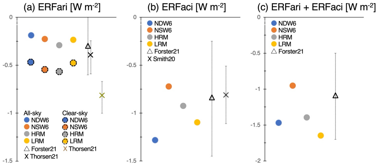
Figure 11: Global and annual mean values of (a) effective radiative forcing for anthropogenic aerosol-radiation interaction (ERFari) for net (sum of shortwave and longwave) radiation, (b) ERFaci for anthropogenic aerosol-cloud interaction, and (c) the net ERF (sum of ERFari and ERFaci). All units are in \text{W m}^{-2} . In ERFari, the reference of Forster21 is estimated in the net radiation by IPCC-AR6 or Forster et al. (2021), whereas the reference of Thorsen21 is estimated in the shortwave radiation by Thorsen et al. (2021). The reference for Smith20 is Smith et al. (2020). The values are also listed in Table 2.
