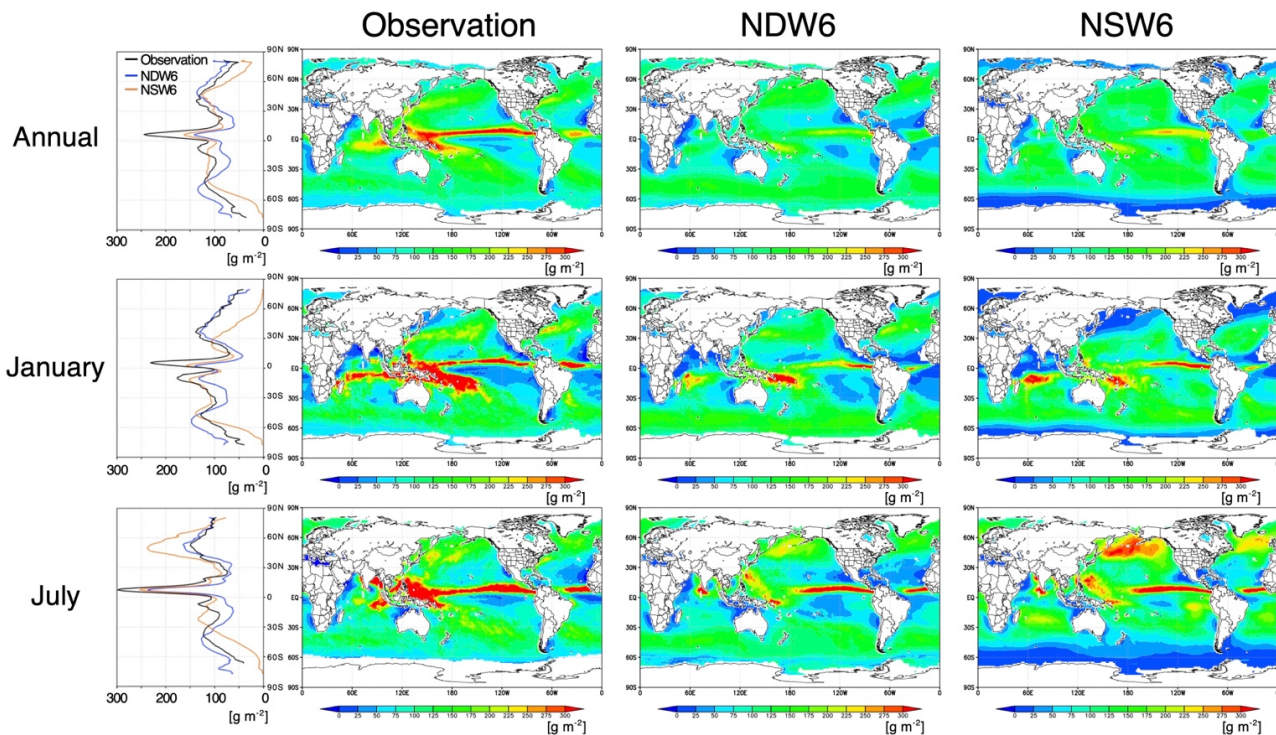
1235 Figure 2: Zonal and horizontal distributions of LWP (NDW6 and NSW6 simulations and MAC as observations) over only the ocean as annual, January, and July averages. All units are in \text{g m}^{-2} .
