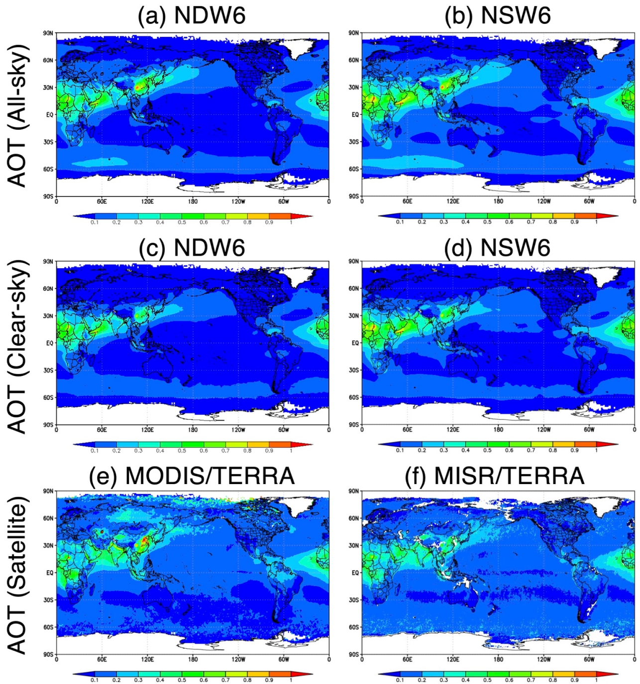
Figure 8: Global distributions of the annual averages of the NDW6-simulated AOT under (a) all-sky and (c) clear-sky conditions, the NSW6-simulated AOT under (b) all-sky and (d) clear-sky conditions, and (e) the MODIS/TERRA-retrieved and (f) the MISR/TERRA-retrieved AOT under clear-sky conditions.
