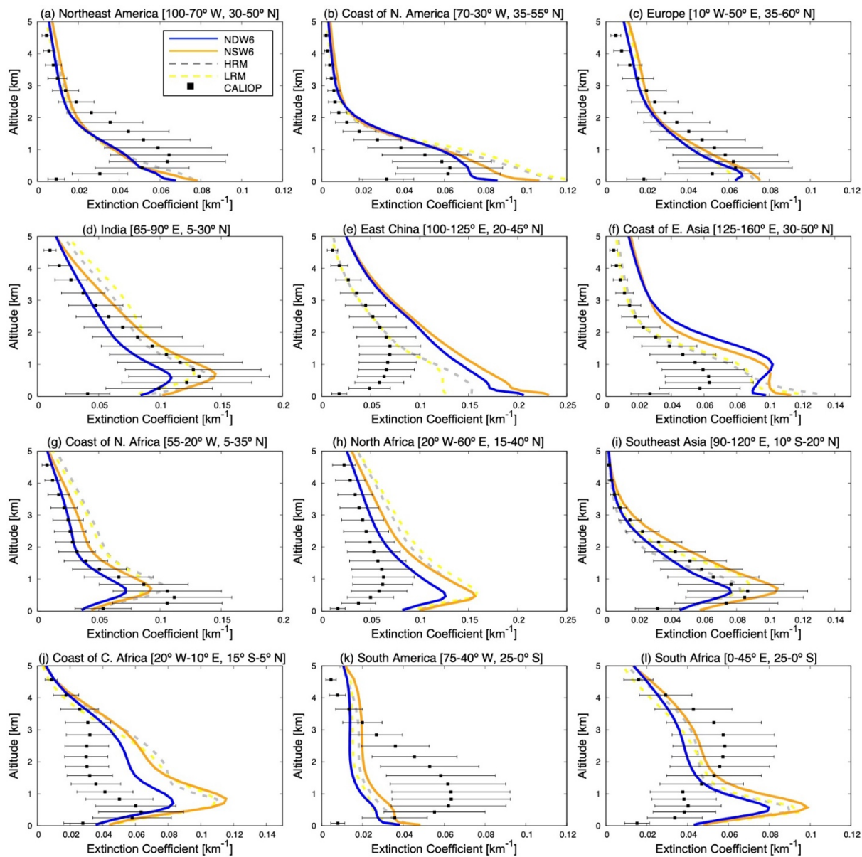
Figure 9: Vertical profiles of the annually and regionally averaged aerosol extinction coefficients from the NICAM simulations (NDW6, NSW6, HRM and LRM) and from CALIOP/CALIPSO observations in 12 different regions, which are generally defined in Goto et al. (2020) and Koffi et al. (2016). The CALIOP-retrieved values include the standard deviation of the results from 2014–2016 as bars. All units are in km -1 .
