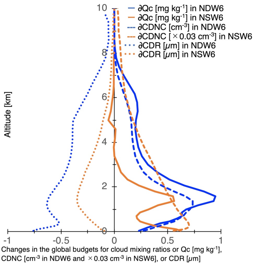
1310 Figure 14: Global budgets of the annual averages of the NDW6- and NSW6-simulated Q_c (mixing ratio of cloud droplets), the NDW6-simulated CDNC, the NSW6-simulated CDNC (which is equal to CCN number concentrations), and the NDW6- and NSW6-simulated CDR (cloud droplet effective radius for warm clouds)
