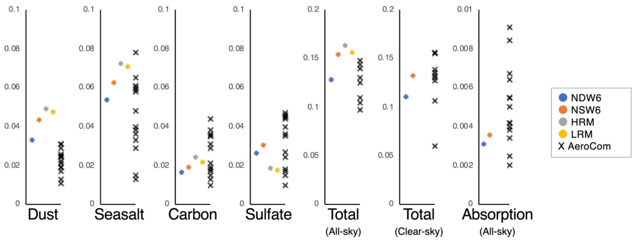
1330 Figure C1: Global and annual mean values of AOT for chemical components (dust, sea salt, carbonaceous aerosols, and sulfate) under all sky conditions, AOT of total aerosols under both all-sky and clear-sky conditions, and absorption AOT under all-sky conditions. There are no HRM and LRM results for AOT under clear-sky conditions and absorption AOT.
