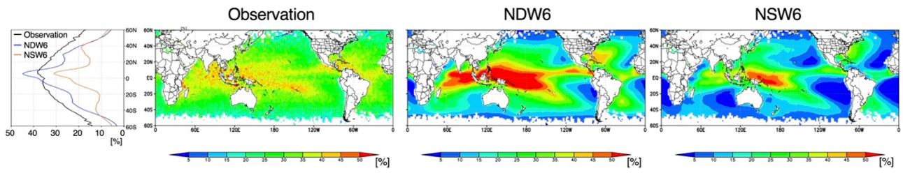
Figure 6: (a) NDW6-simulated, (b) NSW6-simulated, and (c) Cloudsat-retrieved ratio of column precipitation to the sum of column precipitation and total cloud water (RPCW) above 1 km height as annual averages. All units are in %.
