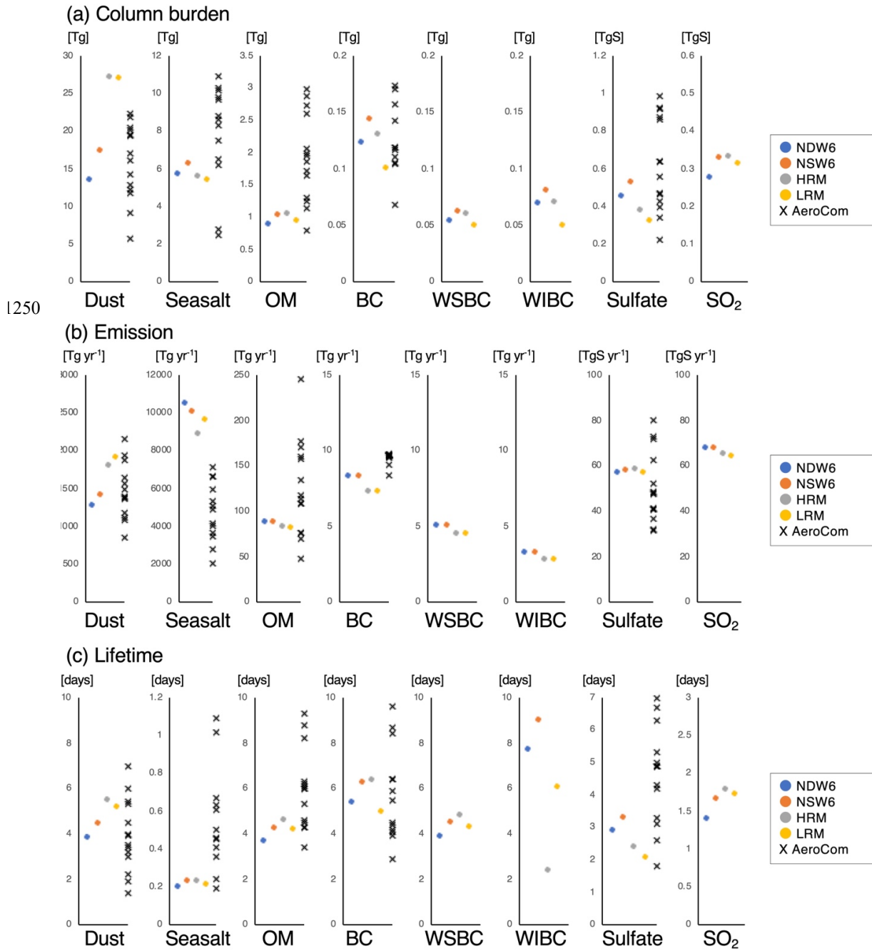
Figure 5: Global and annual mean values of (a) column burdens [Tg or TgS], (b) emission fluxes [Tg yr -1 or TgS yr -1 ], and (c) atmospheric lifetimes of the simulated aerosols and SO 2 [days]. The results include NDW6 and NSW6 in this study and references for the HRM and LRM in Goto et al. (2020) and AeroCom (Gliß et al., 2021). The values are also listed in Table A2.
