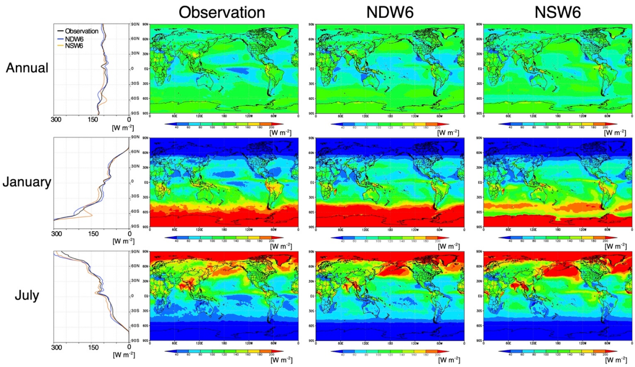
1340 Figure E2: Same as Figure E1 but for OSR.
