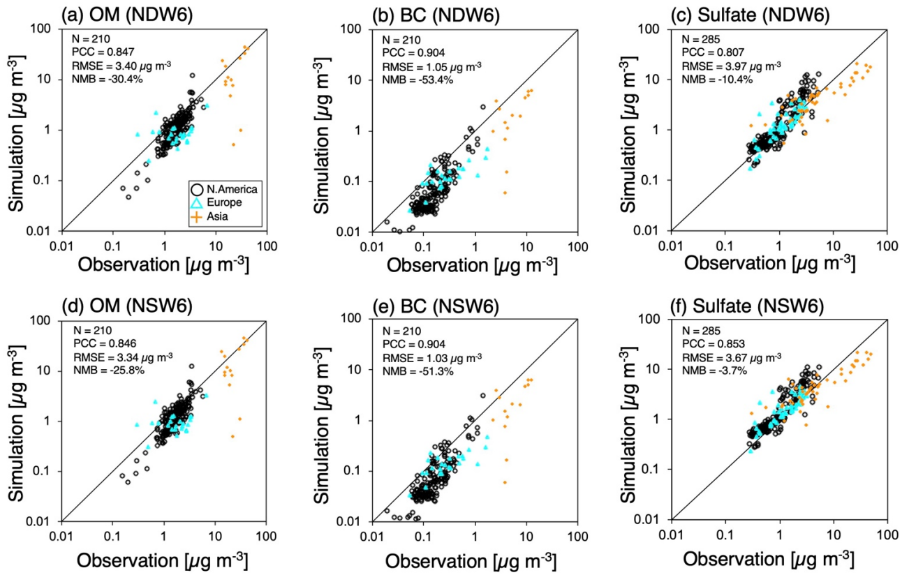
Figure 4: Scatterplots of the annual averages of surface aerosol mass concentrations (OM, BC, and sulfate) between in situ measurements (IMPROVE, EMEP, EANET and CAWNET) and the NICAM simulations (NDW6 and NSW6). All units are in \mu\text{g m}^{-3} . The statistical metrics (N: sampling number, PCC: Pearson correlation coefficient, RMSE: root-mean-square error, and NMB: normalized mean bias), defined as (A1)-(A3) in Appendix A, are also shown in each panel. The values are also listed in Table A1.
