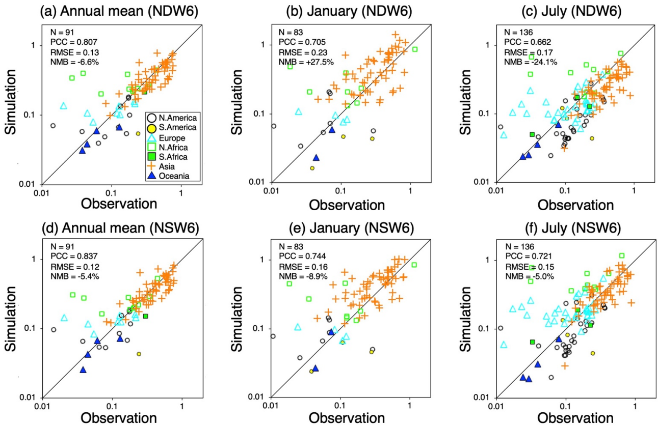
1265 Figure 7: Scatterplot of the annual, January and July averages of AOT between ground-based measurements (AERONET, SKYNET and CARSNET) and the NICAM (NDW6 and NSW6) simulations. The different colors and symbols reflect the sites in the different regions (North America, South America, Europe, North Africa, South Africa, Asia, and Oceania) as defined in panel (a). The numbers located in the upper-left corner in each panel represent the statistical metrics, N, PCC, RMSE and NMB, which are defined as (A1)-(A3) in Appendix A.
