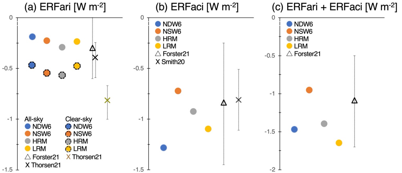
1290 Figure 11: Global and annual mean values of (a) effective radiative forcing for anthropogenic aerosol-radiation interaction (ERFari) for net (sum of shortwave and longwave) radiation, (b) ERFaci for anthropogenic aerosol-cloud interaction, and (c) the net ERF (sum of ERFari and ERFaci). All units are in \text{W m}^{-2} . In ERFari, the reference of Forster21 is estimated in the net radiation by IPCC-AR6 or Forster et al. (2021), whereas the reference of Thorsen21 is estimated in the shortwave radiation by Thorsen et al. (2021). The reference for Smith20 is Smith et al. (2020). The values are also listed in Table 2.
