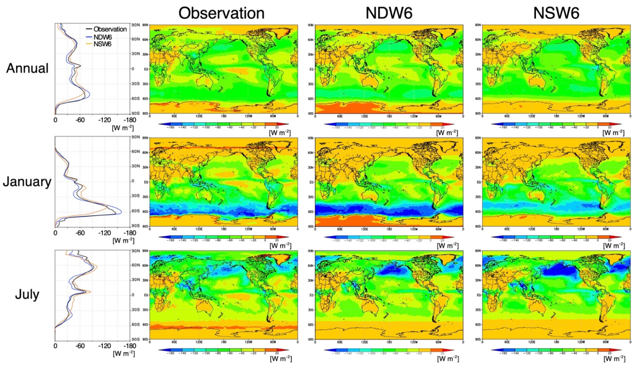
1365 Figure E1: Zonal and horizontal distribution of SWCRF (NDW6 and NSW6 simulations and CERES as observation) as annual, January, and July averages. All units are in W m^{-2} .
