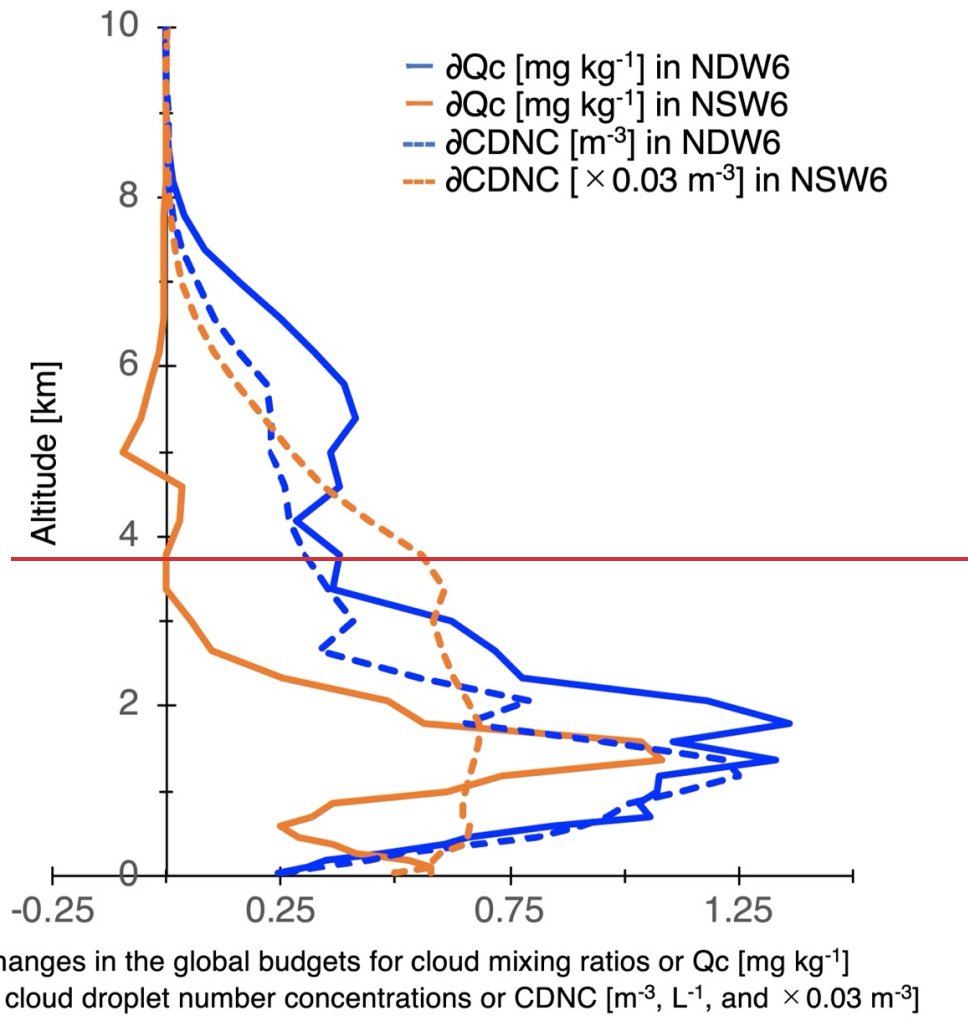
340 Figure 1314: Global budgets of the annual averages of the NDW6- and NSW6-simulated Q_c (mixing ratio of cloud droplets), the NDW6-simulated CDNC ( cloud droplet number concentration ), and the NSW6-simulated CDNC ( cloud droplet number concentration , which is equal to CCN number concentrations), and the NDW6- and NSW6-simulated CDR ( cloud droplet effective radius for warm clouds )
