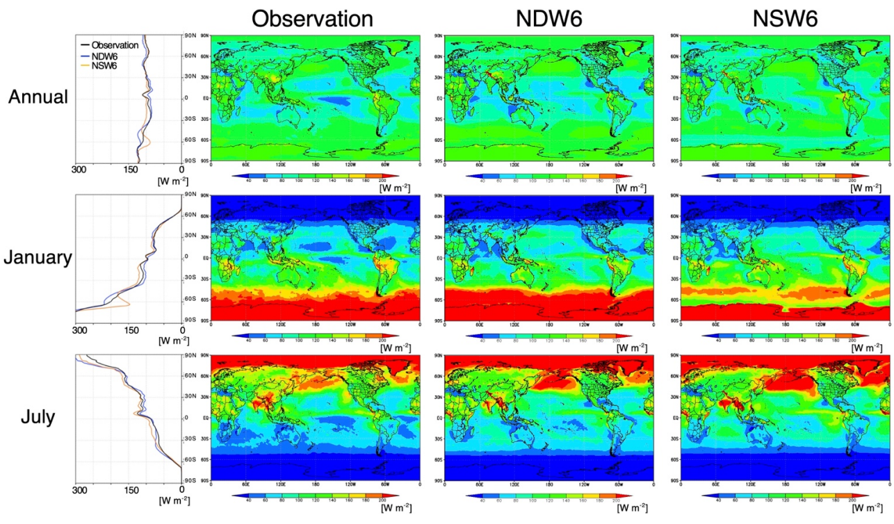
1370 Figure E2: Same as Figure E1 but for OSR.
