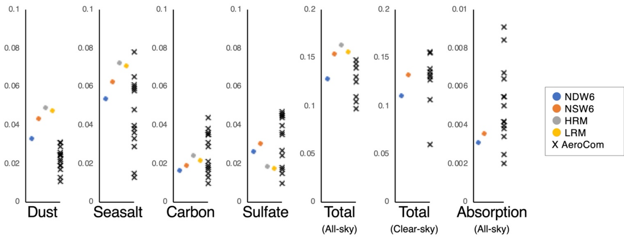
1360 Figure C1: Global and annual mean values of AOT for chemical components (dust, sea salt, carbonaceous aerosols, and sulfate) under all sky conditions, AOT of total aerosols under both all-sky and clear-sky conditions, and absorption AOT under all-sky conditions. There are no HRM and LRM results for AOT under clear-sky conditions and absorption AOT.
