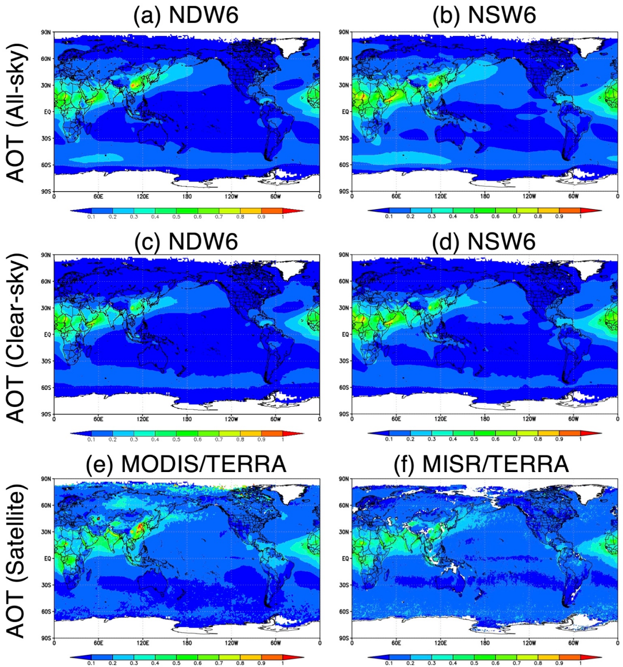
Figure 78: Global distributions of the annual averages of the NDW6-simulated AOT under (a) all-sky and (c) clear-sky conditions, the NSW6-simulated AOT under (b) all-sky and (d) clear-sky conditions, and (e) the MODIS/TERRA-retrieved and (f) the MISR/TERRA-retrieved AOT under clear-sky conditions.
