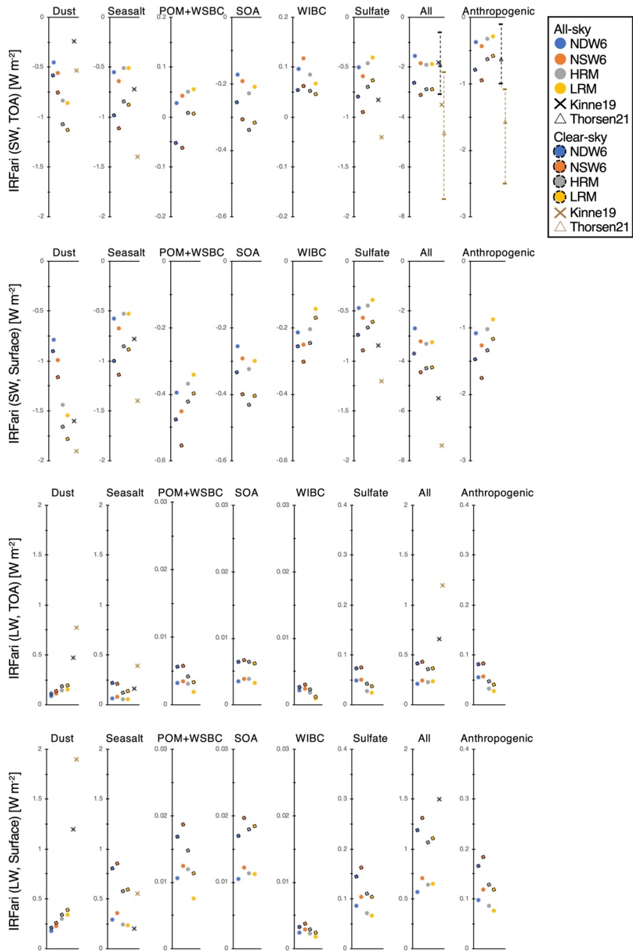
Figure 910: Instantaneous radiative forcing due to aerosol-radiation interaction (IRFari) for each aerosol (dust, sea salt, POM+WSBC, SOA, WIBC, and sulfate), total aerosols (all), and anthropogenic aerosols only (anthropogenic) for shortwave and longwave radiation at the TOA and the surface. The references are Thorsen et al. (2021) and Kinne (2019). All units are in \text{W m}^{-2} .
