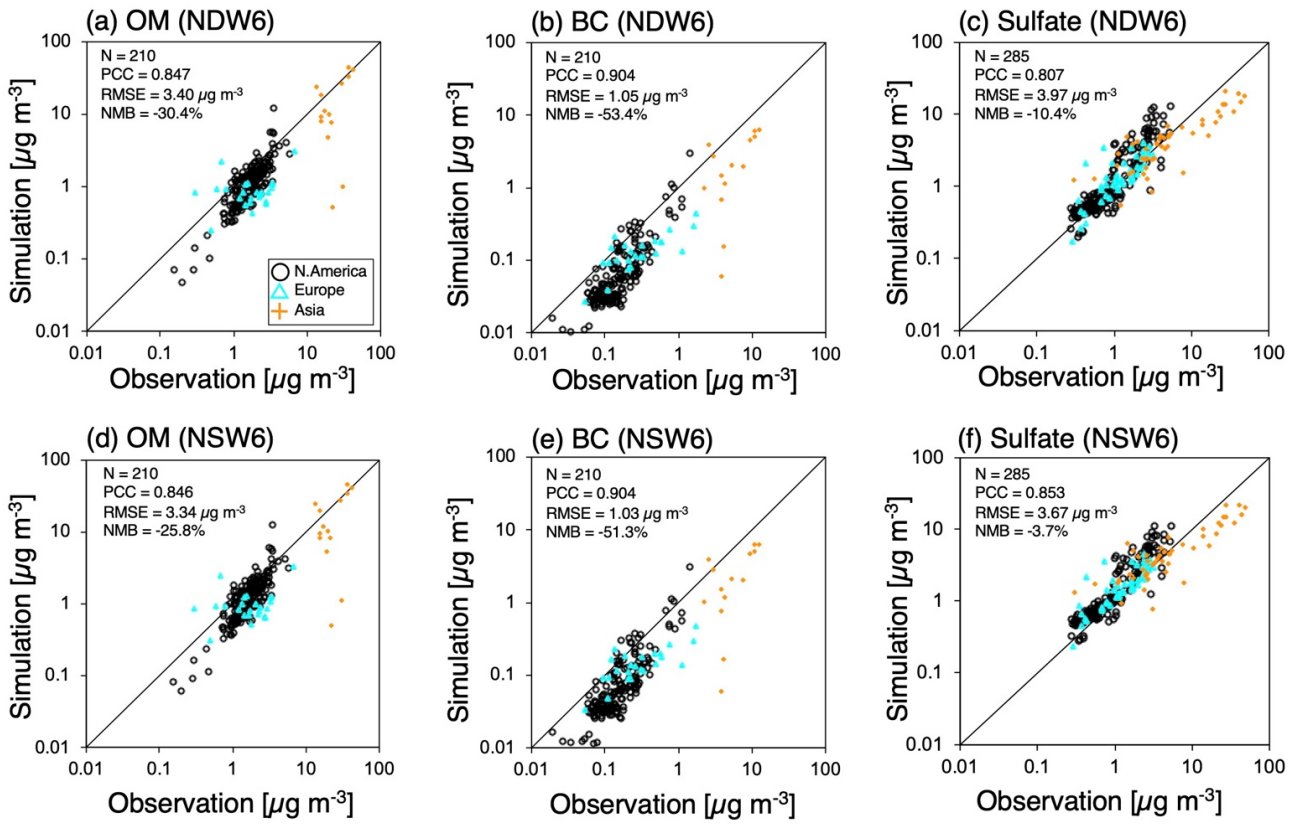
Figure 34: Scatterplots of the annual averages of surface aerosol mass concentrations (OM, BC, and sulfate) between in situ measurements (IMPROVE, EMEP, EANET and CAWNET) and the NICAM simulations (NDW6 and NSW6). All units are in \mu\text{g m}^{-3} . The statistical metrics (N: sampling number, PCC: Pearson correlation coefficient, RMSE: root-mean-square error, and NMB: normalized mean bias), defined as (A1)-(A3) in Appendix A, are also shown in each panel. The values are also listed in Table A1.
