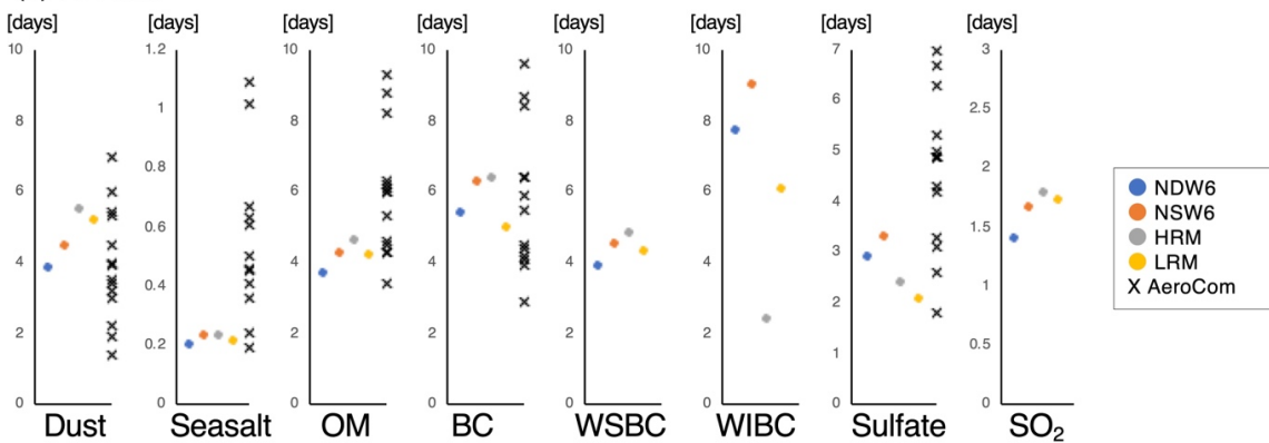
Figure 45: Global and annual mean values of (a) column burdens [Tg or TgS], (b) emission fluxes [Tg yr -1 or TgS yr -1 ], and (c) atmospheric lifetimes of the simulated aerosols and SO 2 [days]. The results include NDW6 and NSW6 in this study and references for the HRM and LRM in Goto et al. (2020) and AeroCom (Gliß et al., 2021). The values are also listed in Table A2.
