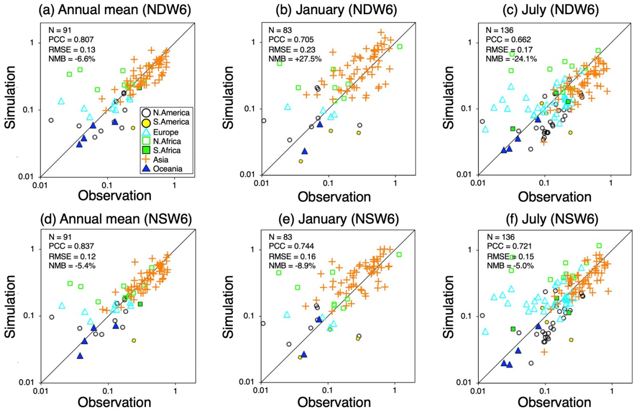
285 | Figure 67: Scatterplot of the annual, January and July averages of AOT between ground-based measurements (AERONET, SKYNET and CARSNET) and the NICAM (NDW6 and NSW6) simulations. The different colors and symbols reflect the sites in the different regions (North America, South America, Europe, North Africa, South Africa, Asia, and Oceania) as defined in panel (a). The numbers located in the upper-left corner in each panel represent the statistical metrics, N, PCC, RMSE and NMB, which are defined as (A1)-(A3) in Appendix A.
