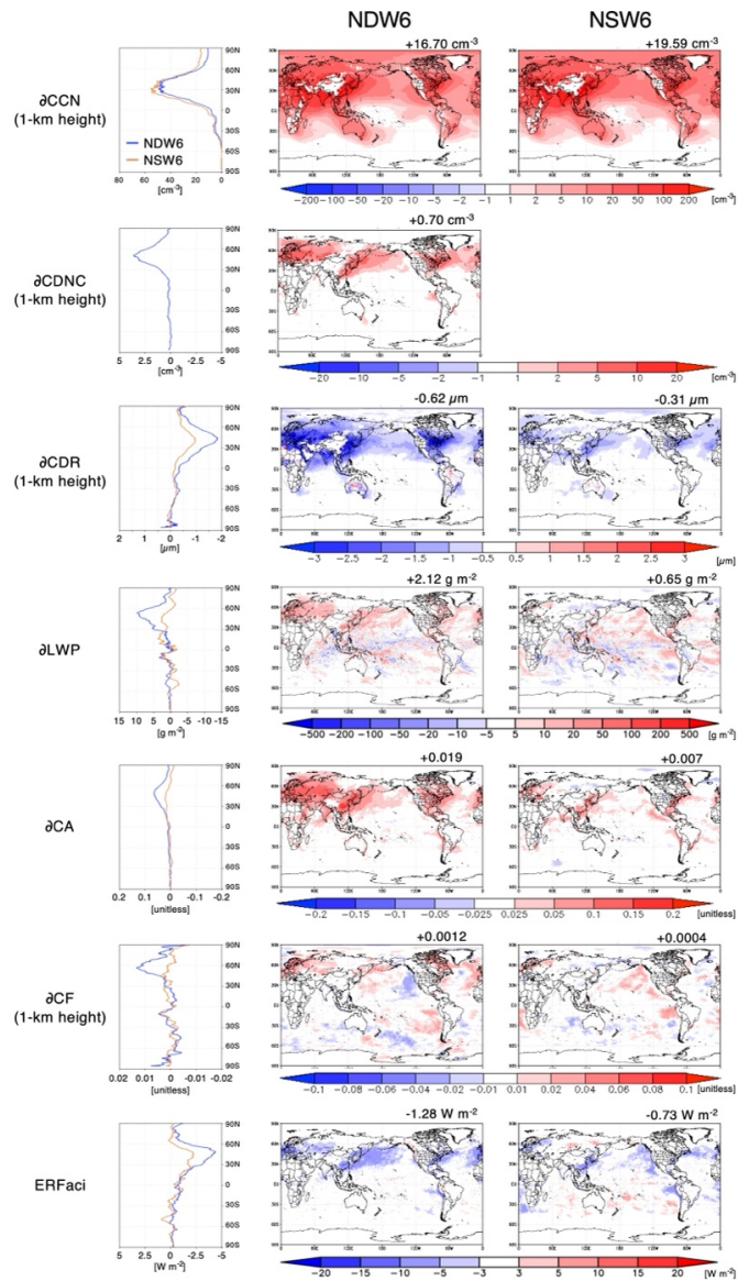
1295 Figure 12: Global distributions of the annual averages of the NDW6- and NSW6-simulated CCN change at 1-km height ( \partial\text{CCN} ), CDNC (which in NSW6 is equal to the CCN concentrations in NSW6 due to the ignorance of sink processes in the CDNC in NSW6) change at 1-km height ( \partial\text{CDNC} ), CDR change for warm clouds at 1-km height ( \partial\text{CDR} ), LWP change ( \partial\text{LWP} ), CA change ( \partial\text{CA} ), CF change at 1-km height ( \partial\text{CF} ), and net ERFaci by comparing the results between NDW6 and NSW6 for simulations with aerosol 1300 and precursor gas emissions for the present and the preindustrial era. The number located in the upper right in each panel represents the global and annual mean value. The results at 1-km height also include areas with elevations higher than 1-km height in white.
