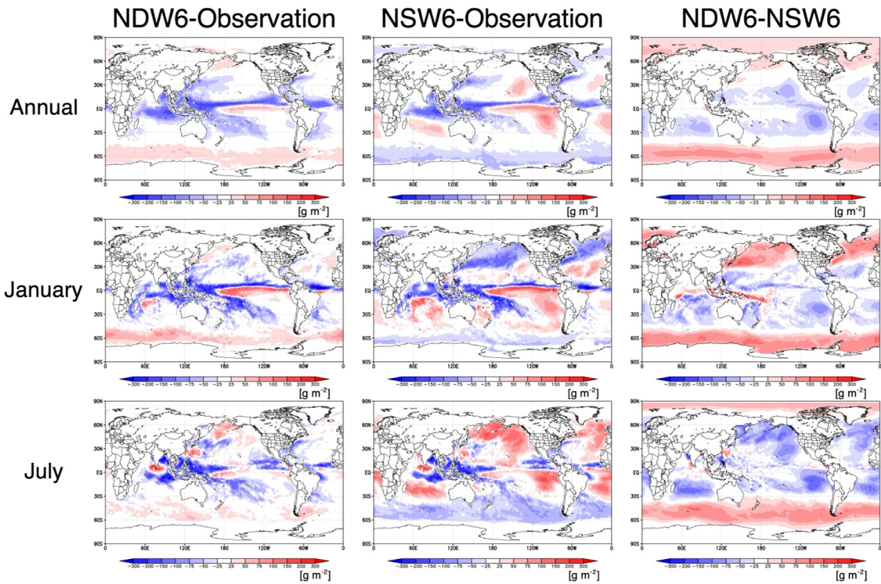
Figure 3: Horizontal distributions of differences in LWP among NDW6, NSW6 and Observation (MAC) over only the ocean as annual, January, and July averages. All units are in g m -2 .
