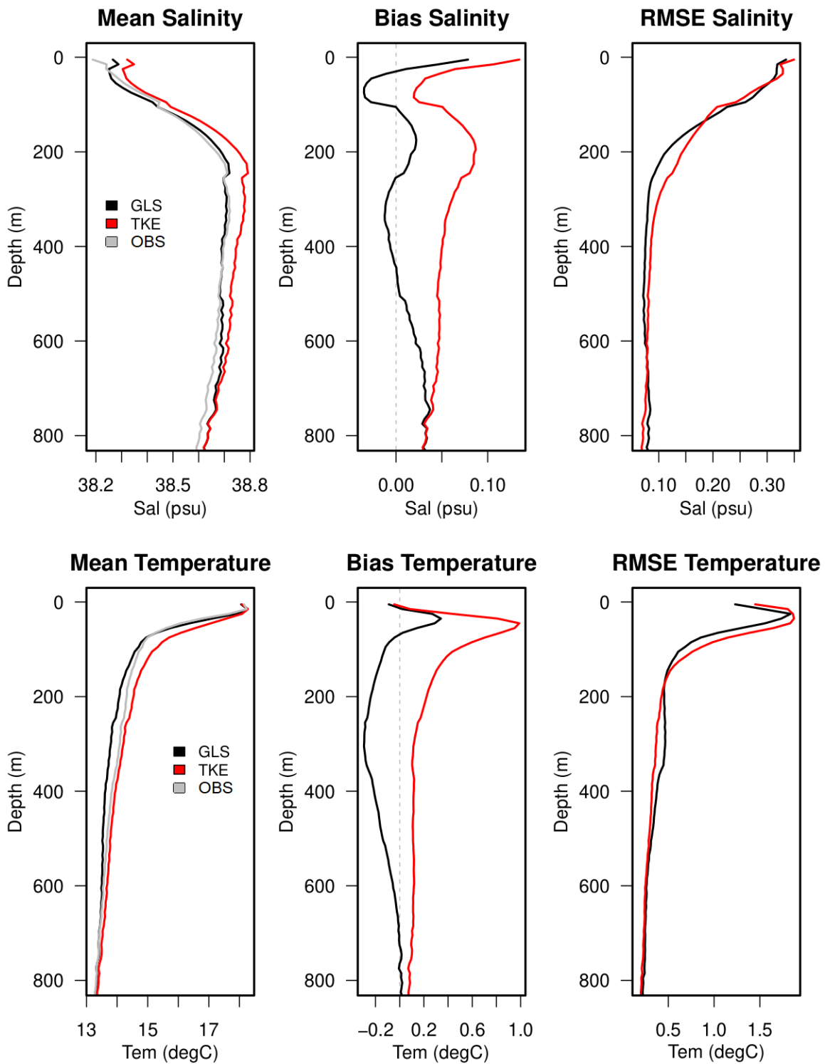
755 Figure 6. As for Figure 4, for the mean, bias, and RMSE profiles against Argo floats, for the GLS and TKE experiments with different oceanic vertical mixing schemes. Mean profiles also report data from the observations (in gray).
