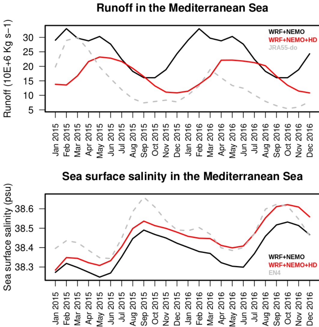
Figure 2. Monthly means of river discharge into the ocean (top panel) and sea surface salinity (bottom panel) averaged over the Mediterranean Sea, from the experiments with and without the interactive river discharge. Also shows for reference the bias-corrected discharge from the JRA55-do reanalysis and the sea surface salinity from the UKMO EN4 objective analyses.
