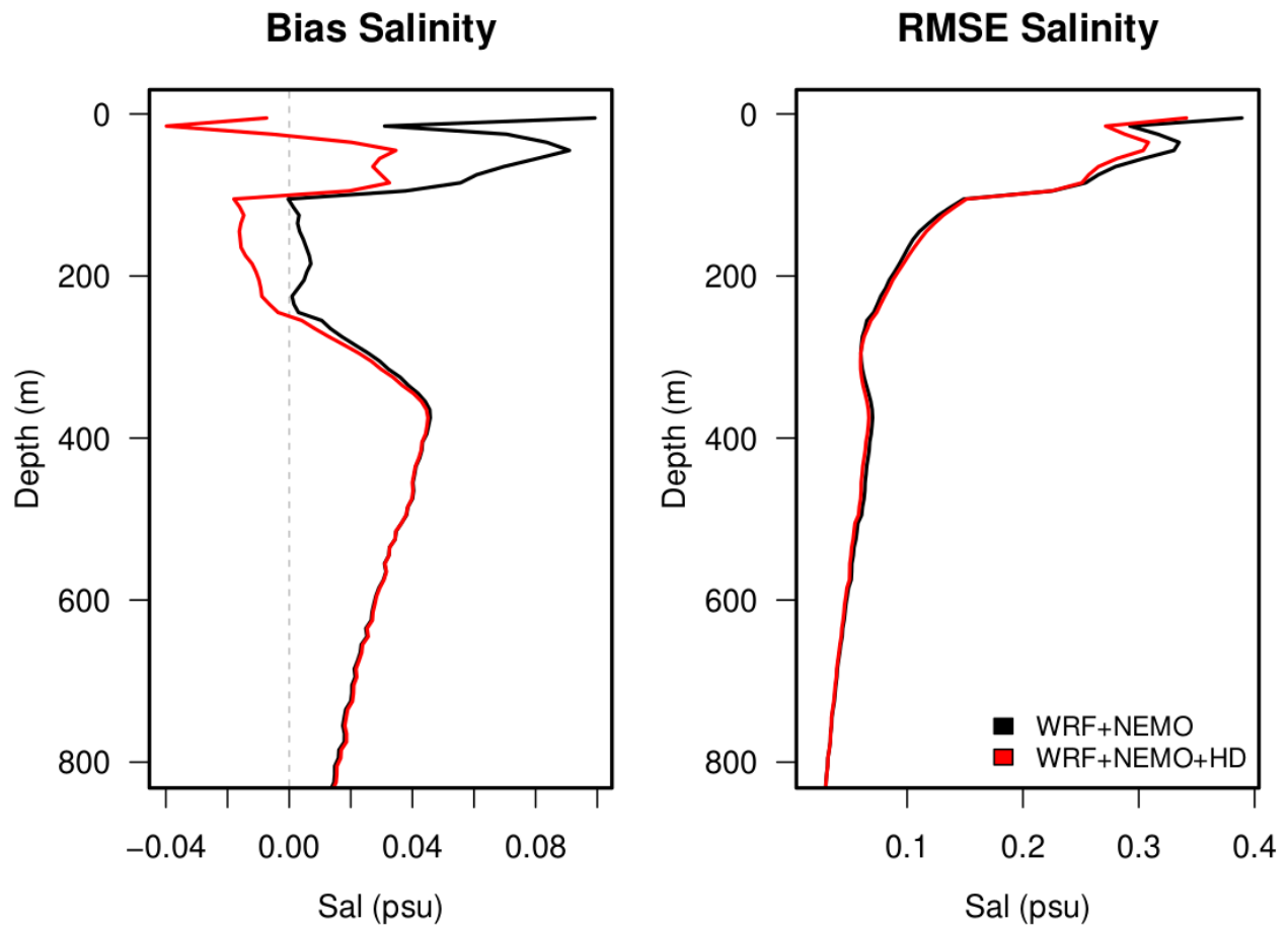
745 Figure 4. Profiles of bias and RMSE against observations from Argo floats (EN4 profile dataset) for the experiments with and without the interactive river discharge, over the Mediterranean Sea.
