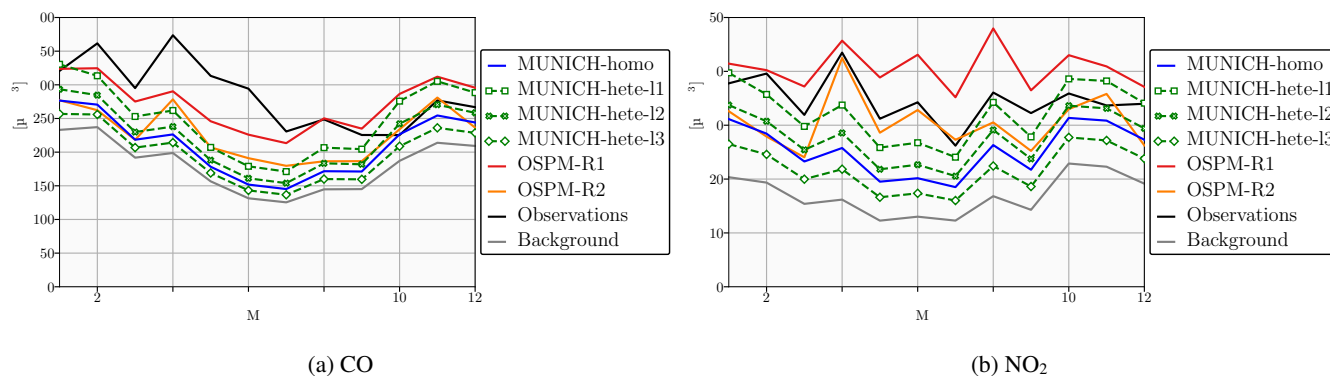
Figure 3. Monthly-average concentrations (in \mu\text{g m}^{-3} ) of CO (a) and \text{NO}_2 (b) at HCAB monitoring station. The solid blue line represents the homogeneous version of MUNICH. The three green dashed lines represents the three levels of the heterogeneous version of MUNICH, the lowest level (11) with square markers, the intermediate level (12) with cross markers and the top level (13) with diamond markers. The solid red line represents the OSPM receptor that is close to the measurement station and the solid orange line the second OSPM receptor located on the other side of the street. The observations are in solid black and the background concentrations in solid grey.
