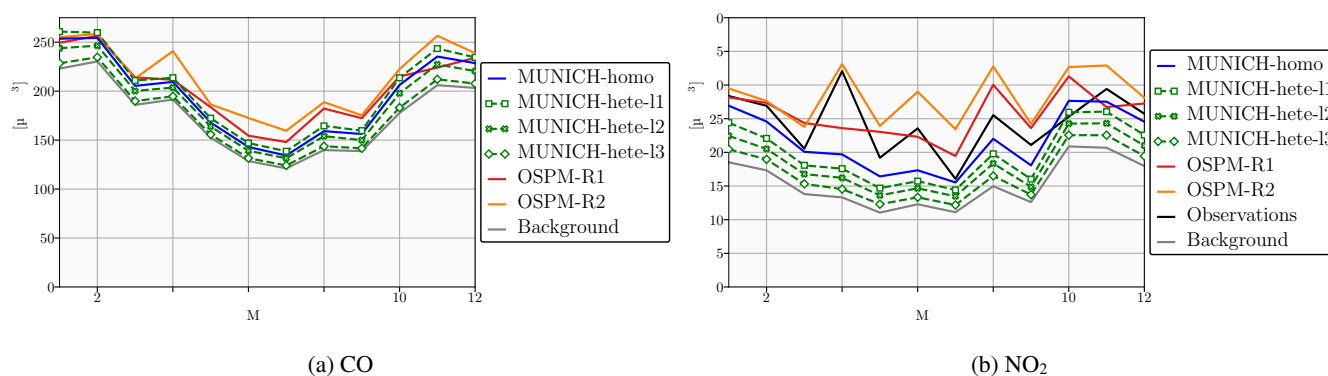
Figure 5. Monthly-average concentrations (in \mu\text{g m}^{-3} ) of CO (a) and NO 2 (b) at JGTV monitoring station. The solid blue line represents the homogeneous version of MUNICH. The three green dashed lines represents the three levels of the heterogeneous version of MUNICH, the lowest level (11) with square markers, the intermediate level (12) with cross markers and the top level (13) with diamond markers. The solid orange line represents the OSPM receptor that is close to the measurement station and the solid red line the second OSPM receptor located on the other side of the street. The observations (only available for NO 2 ) are in solid black and the background concentrations in solid grey
