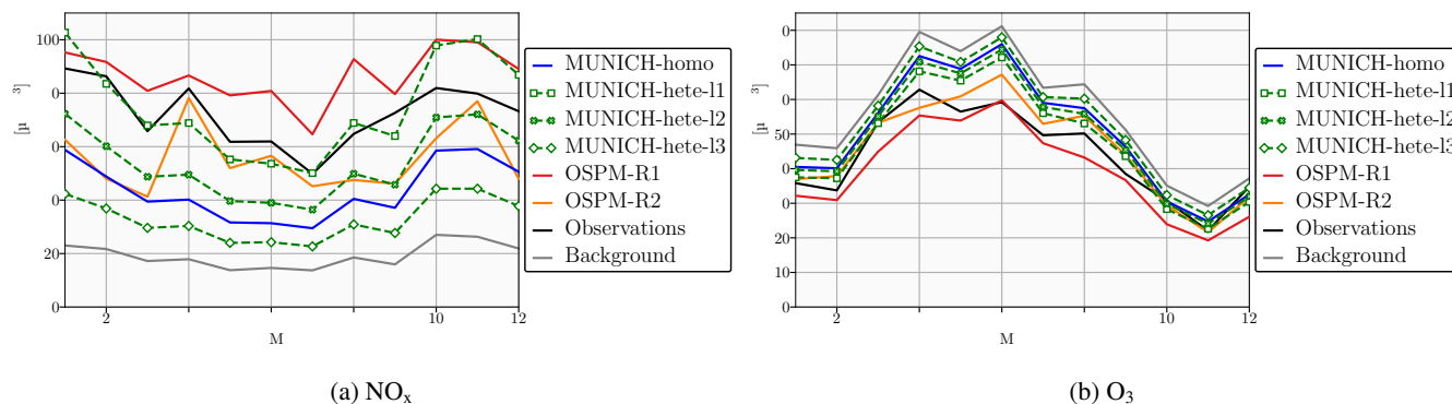
Figure C1. Monthly-average concentrations (in \mu\text{g m}^{-3} ) of NO x (a) and O 3 (b) at HCAB monitoring station. The solid blue line represents the homogeneous version of MUNICH. The three green dashed lines represent the three levels of the heterogeneous version of MUNICH, the lowest level (11) with square markers, the intermediate level (12) with cross markers and the top level (13) with diamond markers. The solid red line represents the OSPM receptor that is close to the measurement station and the solid orange line the second OSPM receptor located on the other side of the street. The observations are in solid black and the background concentrations in solid grey
