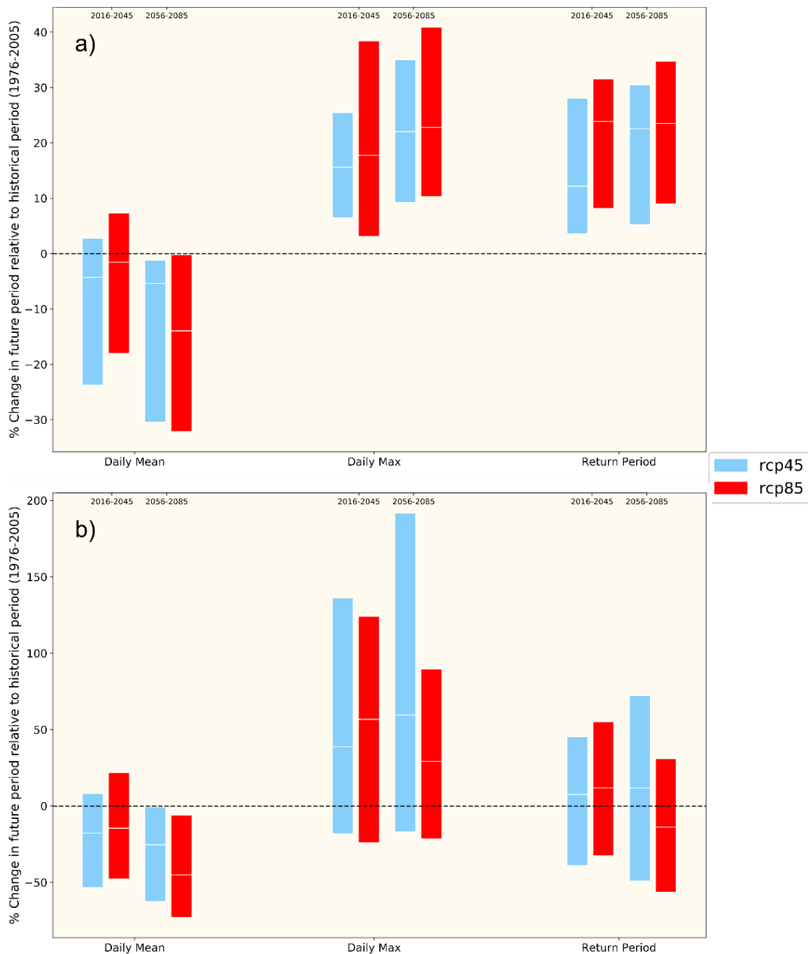
Figure 15: Changes (%) in mean daily, maximum daily and 20-year return period daily rainfall (a) and runoff (b).
