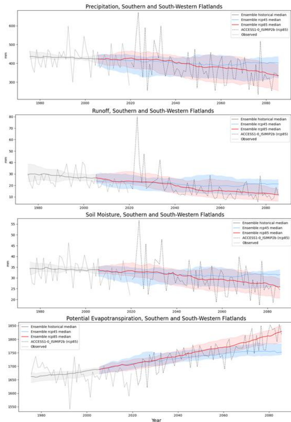
5 Figure 11: Projected ensemble change in precipitation, runoff, root-zone soil moisture and potential evapotranspiration for RCP4.5 (blue) and RCP 8.5 (red) scenarios in the SSWF NRM region. The shaded area represents the 10th to 90th percentile range for all ensemble members. The time-series for ACCESS1-0 (rcp8.5) is included after 2020 to show the variability projected for an individual ensemble member. The reference gridded observations are shown prior to 2020. The ensemble has been smoothed with a 30-year running mean.
