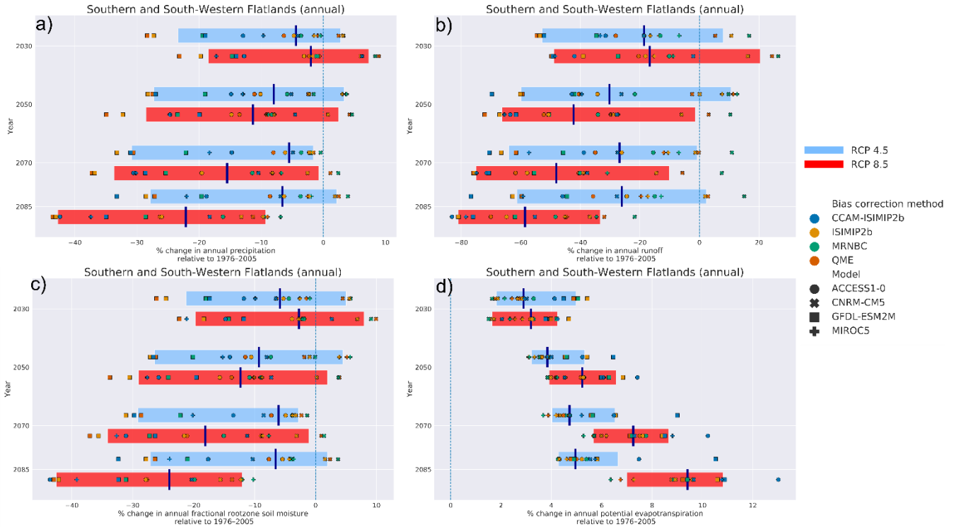
Figure 12: Relative change of annual (a) precipitation, (b) runoff, (c) root-zone soil moisture and (d) potential evapotranspiration. Changes are indicated for each GCM and BC method combination for four 30-year time periods centred on 2030, 2050, 2070 and 2085. The change is the difference of the future from the historical period (1976–2005) expressed as a percentage. The left and right extent of the shaded boxes represent the 10 th and 90 th percentile of the GCM/BC ensemble and the vertical solid line shows the median (50 th percentile). RCP4.5 is shown in blue, RCP 8.5 in red. The ensemble spread for each RCP has been offset from the centre from of our 30-year time slices for legibility, however, each box represents the average of the variability centred on the time slice indicated on the ordinate. Note that time is descending on the ordinate and the change (in percent) is shown on the abscissa.
