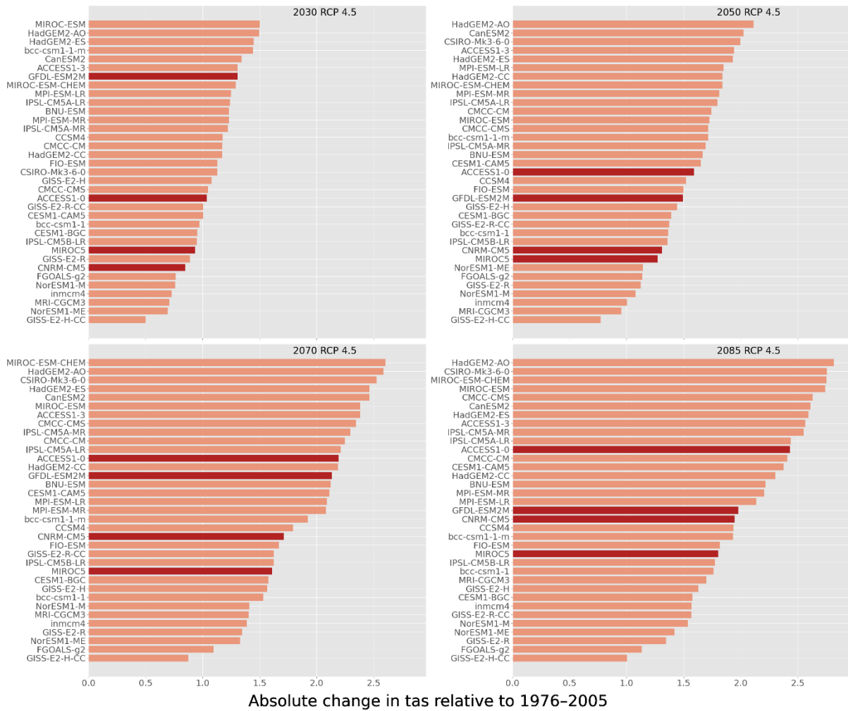
Figure S1: The same as Figure 2 for RCP4.5.
