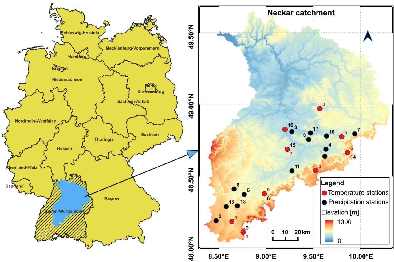
Fig. 2: Weather station locations and elevations in the Neckar catchment. The red circles represent temperature stations (ID corresponds to Table 1b), and the black circles represent precipitation stations (ID corresponds to Table 1a). The colormap shows the elevation and delineates the extent of the catchment.
