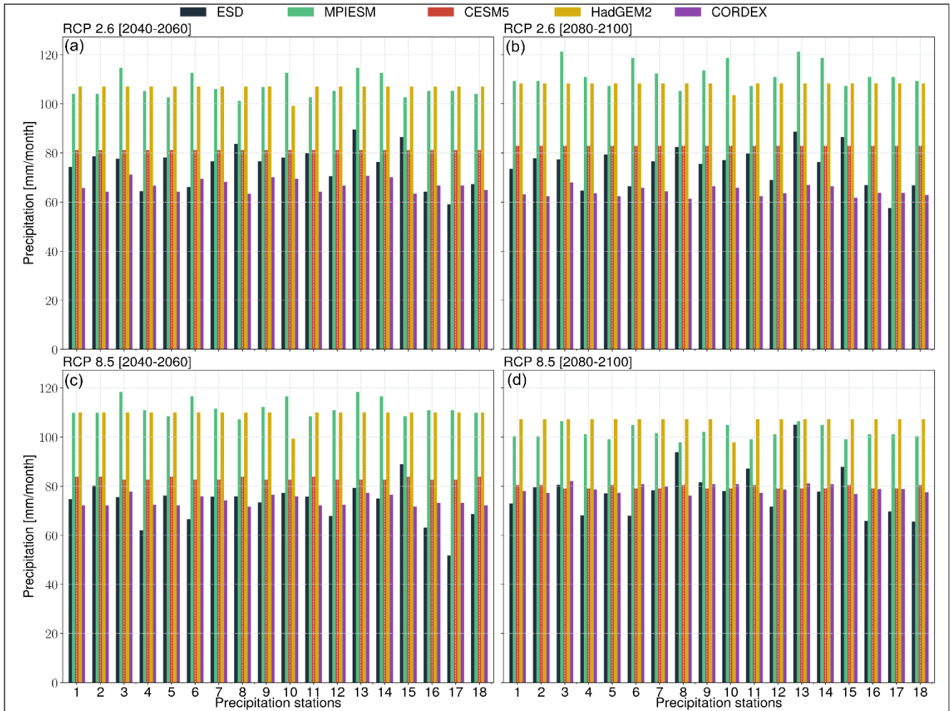
820 Fig. 12: Comparison of 20-year annual precipitation climatologies predicted by the ESD models of this study (black), GCMs (i.e., MPI-ESM (green), CESM5 (red), HadGEM2 (gold) and RCMs (i.e., and CORDEX (purple)) for RCPs 2.6 (a, b) and 8.5 (c, d).
