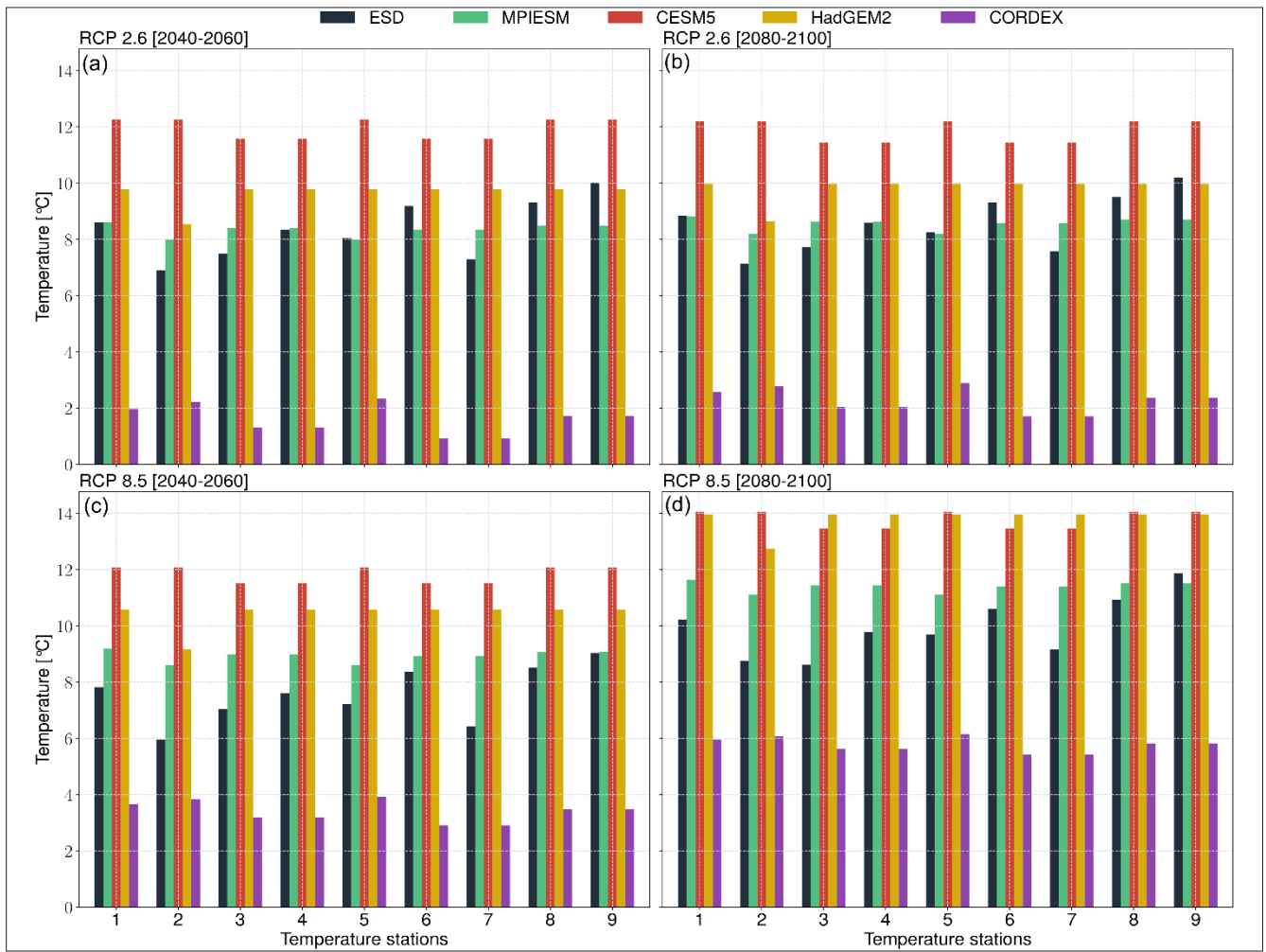
Fig. 13: Comparison of 20-year annual temperature climatologies predicted by the ESD models of this study (black), GCMs (i.e., MPI-ESM (green), CESM5 (red), HadGEM2 (gold) and RCMs (i.e., and CORDEX (purple)) for RCPs 2.6 (a, b) and 8.5 (c, d).
