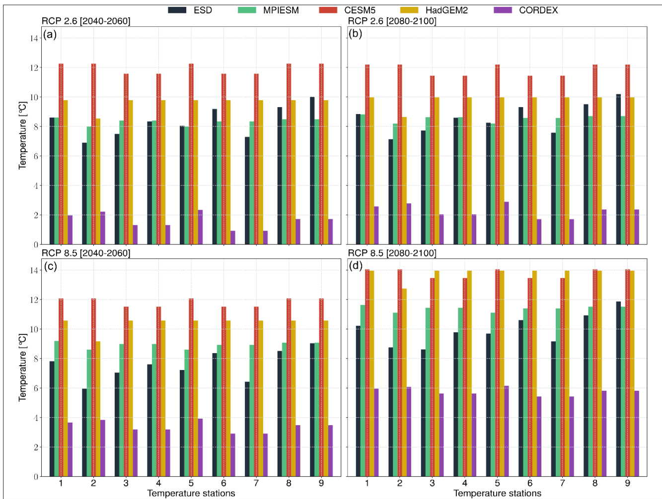
810 Fig. 13: Comparison of 20a annual temperature climatologies predicted by the ESD models of this study (black), GCMs (i.e., MPI-ESM (green), CESM5 (red), HadGEM2 (gold) and RCMs (i.e., and CORDEX (purple)) for RCPs 2.6 (a, b) and 8.5 (c, d).
