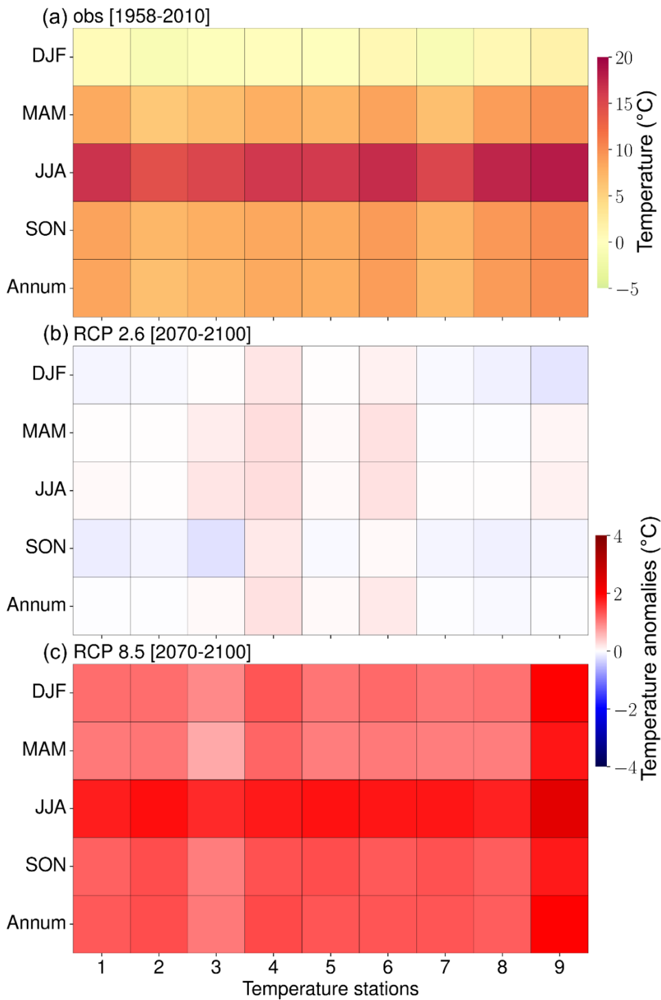
775 Fig. 10: Observed temperature (1958-210), and seasonal (i.e., spring (MAM), summer (JJA), autumn (SON), and winter (DJF)) and annual end-of-century (30-year) temperature climatologies as a result of RCPs 2.6 (b), and RCP 8.5 (c) forcing. The blue (red) colors indicate a decrease (increase) in temperature relative to the observed means (1958-2010).
