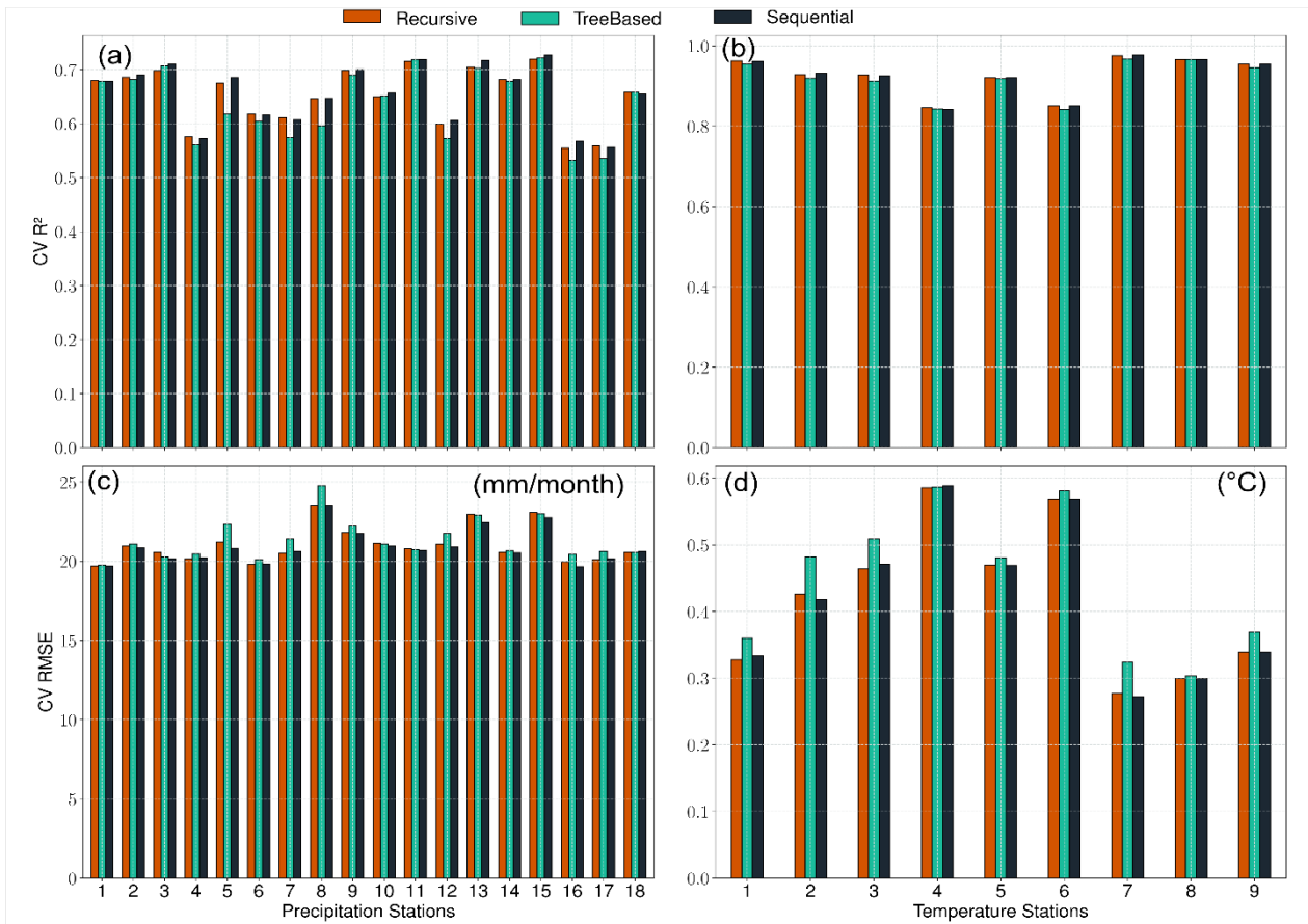
Fig. 4: Cross-validation R^2 and RMSE for the predictor selection methods ( Recursive (red), Tree-based (green), and Sequential (black)) for precipitation (a, c) and temperature (b, d) station records. The individual performed similarly well, suggesting that each of the implemented methods may be used to refine the list of potential predictors.
