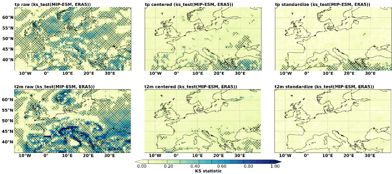
790 Fig. 11: KS two-sided statistical testing score maps the ERA5 reanalysis product and MPI-ESM GCM output for precipitation (top panel) and temperature (bottom panel). The KS test was applied to raw values, anomalies (centered with zero means), and standardized anomalies with unit variance values (columns from left to right, respectively). The grid boxes with black cross stipplings represent low p values ( p < 0.05 ), suggesting statistically significant differences in distribution between the ERA5 and MPI-ESM time series.
