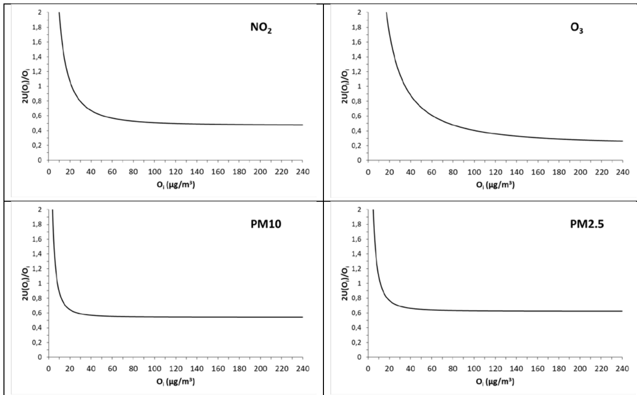
Figure A1: Double relative measurement uncertainties as a function of concentration values for NO 2 (top, left), O 3 (top, right), PM 10 (bottom, left) and PM 2.5 (bottom, right).
