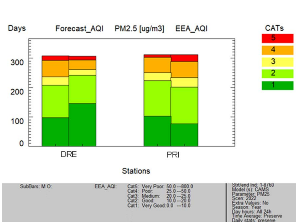
395 Figure 9: FA5 validation outcomes for PM2.5 at Drenas and Pristina. AQI diagram provide for each monitoring station the number of predicted (left bar) and measured (right bar) concentration values that fall within each air quality category. The last two EEA AQI classes (“Very poor” and “Extremely poor”) are merged into one.
