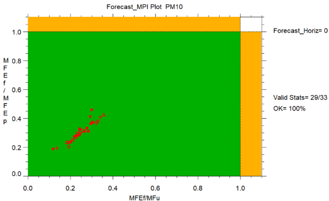
355 Figure 7: FA3 validation outcomes for day0. Forecast Target Plots (top) provide MQI_f values for each monitoring station, as the distance between the origin and a given point. Forecast MPI Plots (bottom) provide for each monitoring station MPI_1 along Y axis and MPI_2 along the X axis.
