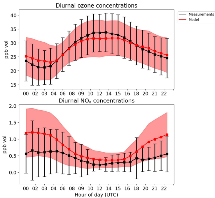
|890 Figure 1515: Diurnal variation of O 3 and NO x at the SMEAR-II site (from 15 June until 30 August of 2019). The extent of the bars and the shaded areas denotes the one standard deviation ( 1\sigma ). Measurements data are shown in in black and model data in red. Units are in ppb vol.
