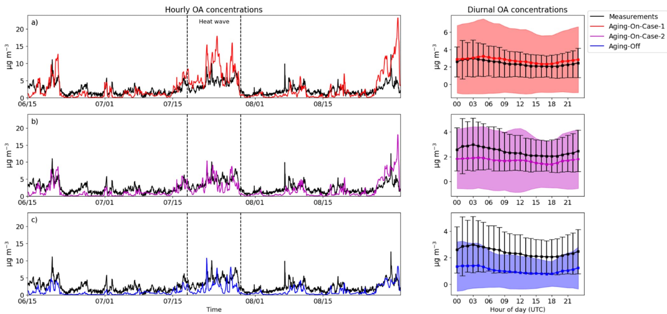
845 | Figure 9: Model (different colors) and measured (black) air concentrations of OA for the a) Aging-On-Case-1, b) Aging-On-Case-2 and c) Aging-Off BSOA schemes. Hourly (left) and diurnal (right) comparisons at the SMEAR-II station. The dashed lines delimit the periods with sustained elevated temperature, denote here as “heat wave”. The extent of the bars and the shaded areas denotes the one standard deviation ( 1\sigma ). Units are in \mu\text{g m}^{-3} .
