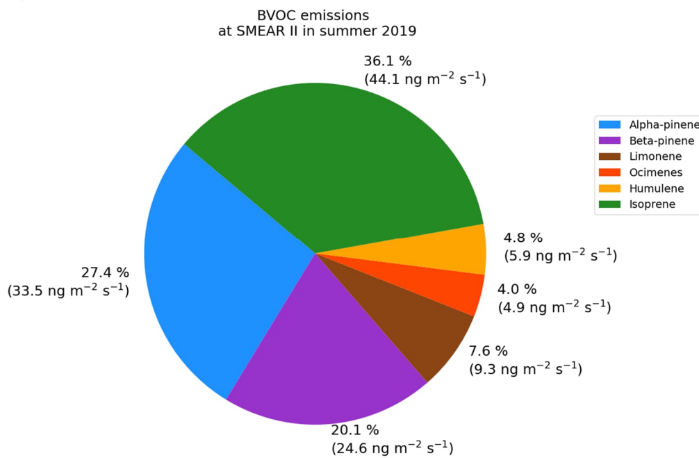
835 Figure 7: Average relative contribution of the BVOCs species as predicted by the MEGAN model for the astronomical summer of 2019 (15 Jun–30 Aug 2019) at the SMEAR-II station. Units are in \text{ng m}^{-2} \text{s}^{-1} .
