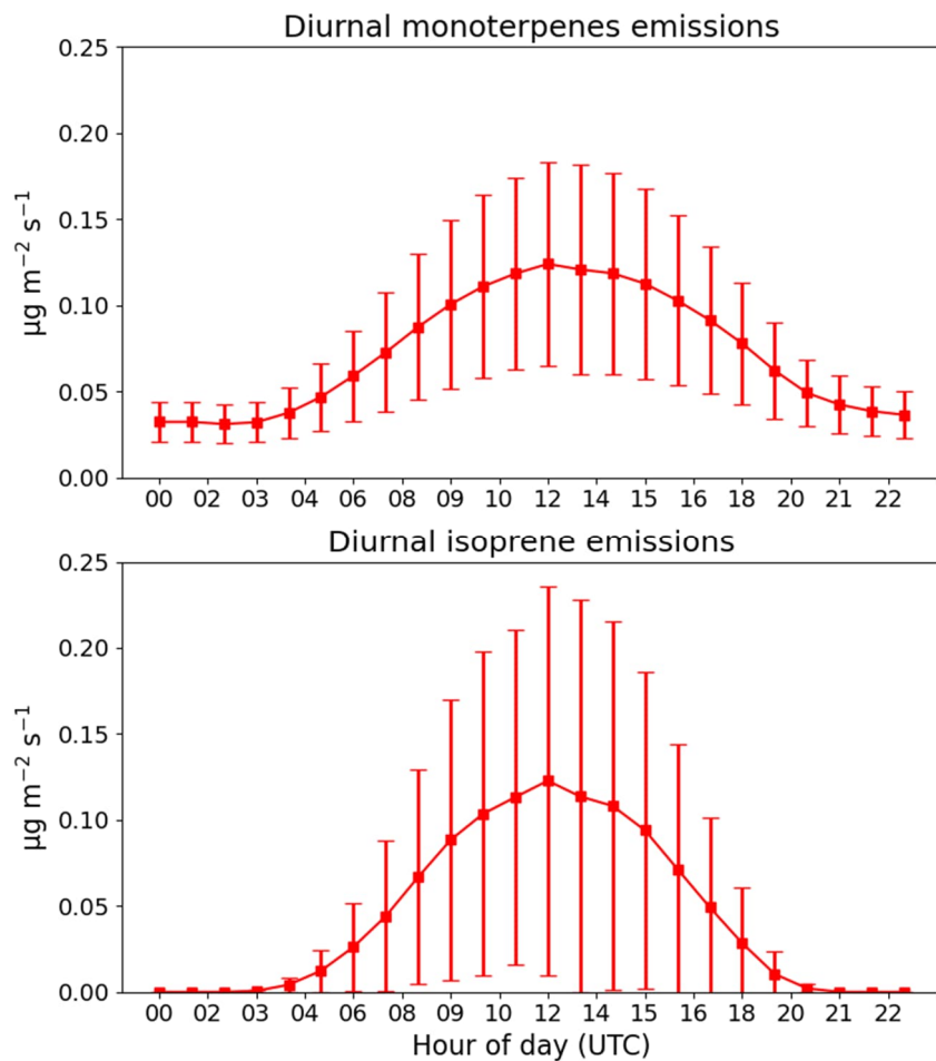
Figure 6: Average diurnal variation of monoterpenes (upper panel) and isoprene (lower panel) emissions ( \mu\text{g m}^{-2} \text{s}^{-1} ) for the astronomical summer of 2019 ( 15 Jun–30 Aug 2019 ) at the SMEAR-II station. The extent of the red bars denotes the one standard deviation ( 1\sigma ). Monoterpenes represent here the sum of all the available terpenes species.
