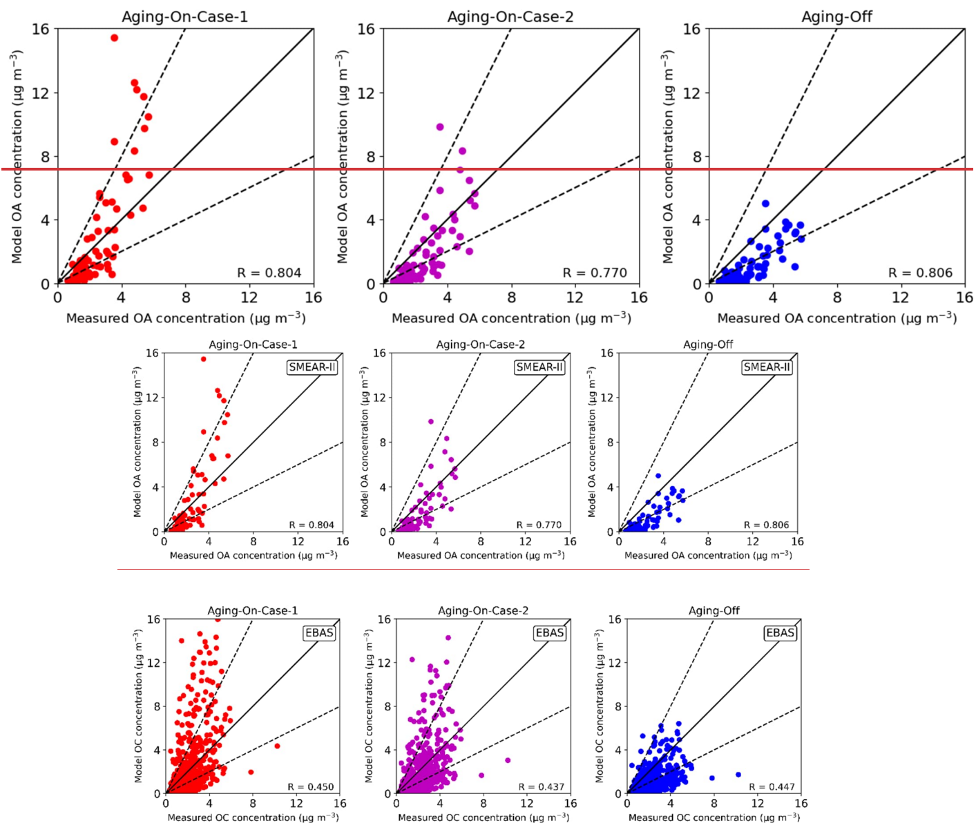
Figure 10: Daily average-Model (y-axis) and measured (x-axis) air concentrations of OA for the Aging-On-Case-1 (left), b) Aging-On-Case-2 (center) and c) Aging-Off (right) BSOA schemes at the SMEAR-II station (upper pane, daily averages) and at available EBAS sites (bottom panel). Solid line indicates the 1:1 line. The dashed lines delimit 1:2 and 2:1 line. Units are in µg m -3 . Data from the EBAS database has a time resolution varying from 4 hours to 1 week, depending on the specific site.
