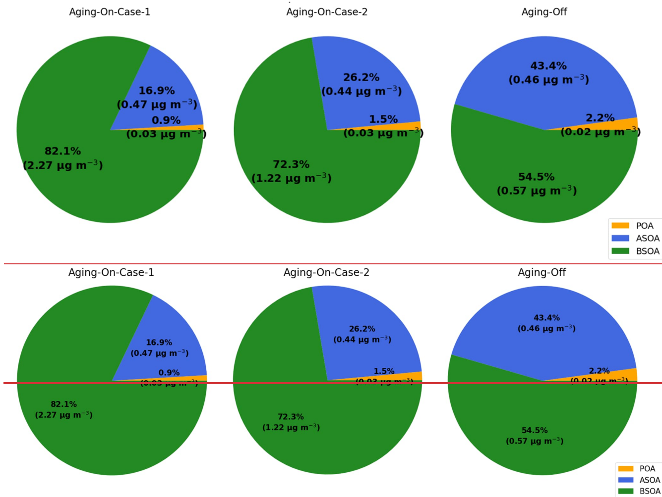
865 Figure 12: POA (orange), ASOA (blue) and BSOA (green) modeled average relative contribution to the total OA fraction for the astronomical summer of 2019 (15 Jun–30 Aug 2019) and for the Aging-On-Case-1 (left), b) Aging-On-Case-2 (center) and c) Aging-Off (right) BSOA schemes. Absolute concentration concentrations are reported along with their relative contribution to the total OA.
