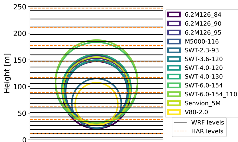
Figure 2. WRF (black solid) and HARMONIE (orange dashed) model levels and rotor areas of the different turbine types used in this study.
