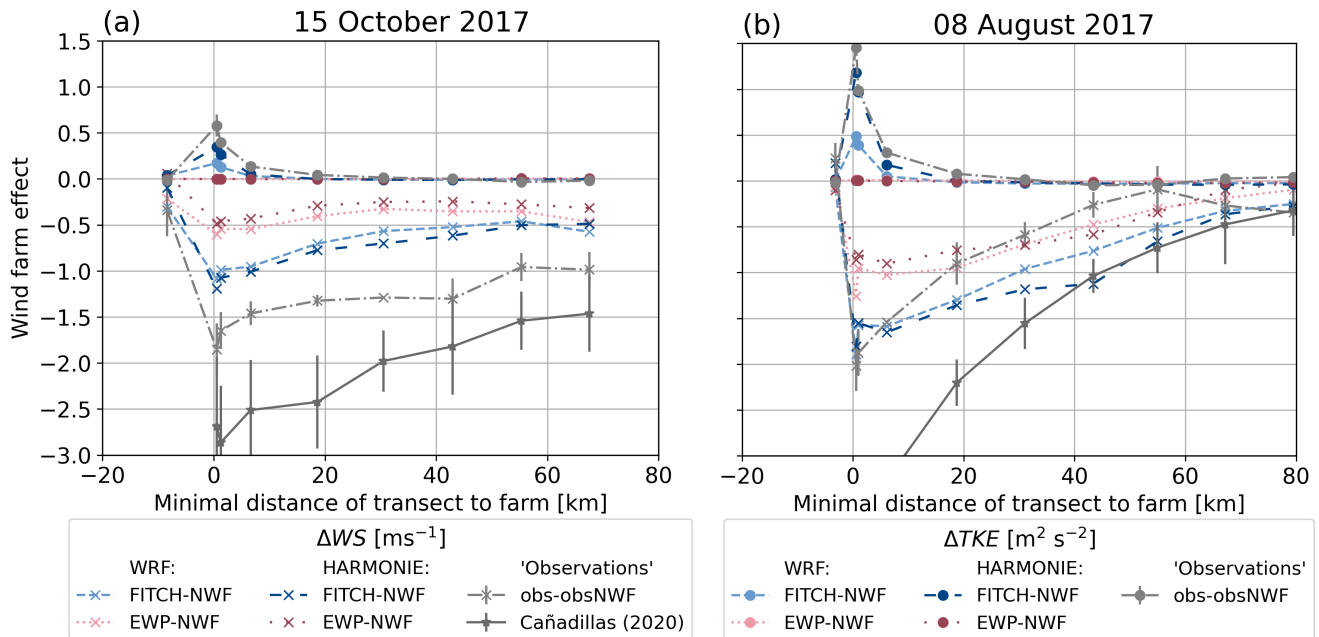
Figure 12. Wake effect at around hub height defined as scenario with WFP (FITCH and EWP) minus scenario without wind farm (NWF) in terms of WS reduction (lines with crosses) and TKE increase (lines with circles) for different transects with a certain minimal distance to the farm for WRF and HARMONIE with same color and line style coding as in Fig. 8 for (a) 15 October 2017 and (b) 08 August 2017. Observational wake effects have been derived based on the methods described in Sect. 2.6. The unbiased standard error of the mean is used to draw the error bars around the observational wake effect.
