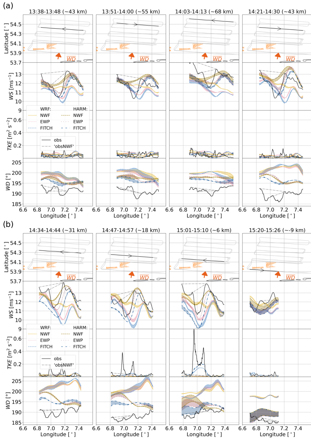
Figure A1. As Fig. 8, but for 15 October 2017 and for around 120 m height for later flight transects as those shown in Fig. 11.
