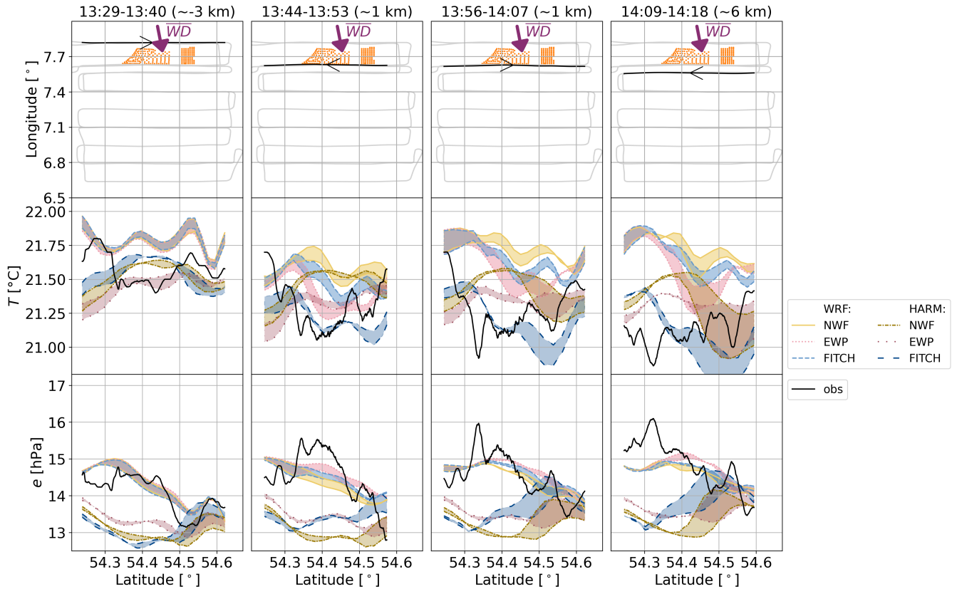
Figure 13. As Fig. 8, but for 08 August 2017 and around 90 m height and for (center row) temperature, (last row) vapour pressure.
