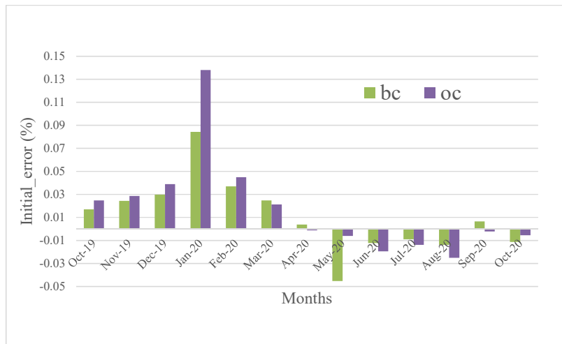
760 Figure 5: BC and OC initial errors (%) at the beginning of each month for the GEFS-Aerosols simulation time period from October 2019 to October 2020.
