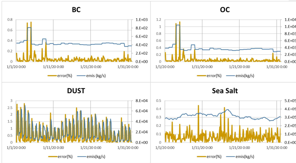
Figure 6: absolute value of model error (brown line, Primary Axis ) for BC, OC, DUST and Sea Salt during GEFS-Aerosol simulations in January 2020, and corresponding aerosol emissions (blue line, Secondary Axis ).
