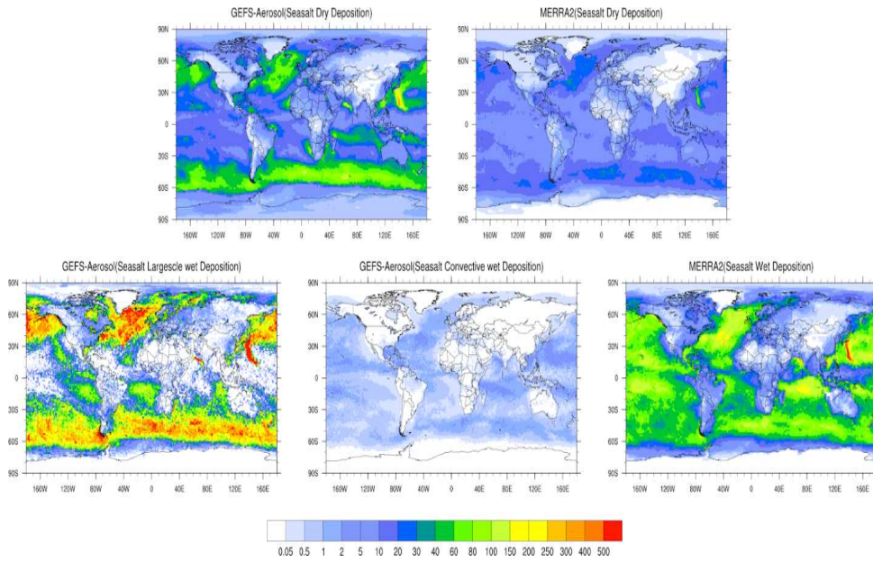
750 Figure 4: sea salt Deposition (October, 2019) in \text{ng/m}^2/\text{s} for GEFS-Aerosols (left side) and MERRA-2 (right side).
