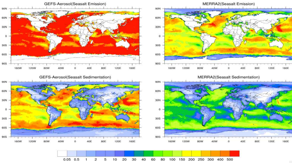
Figure 3: sea salt emission and sedimentation (October, 2019) in \text{ng}/\text{m}^2/\text{s} for GEFS-Aerosols (left side) and MERRA-2 (right side).
